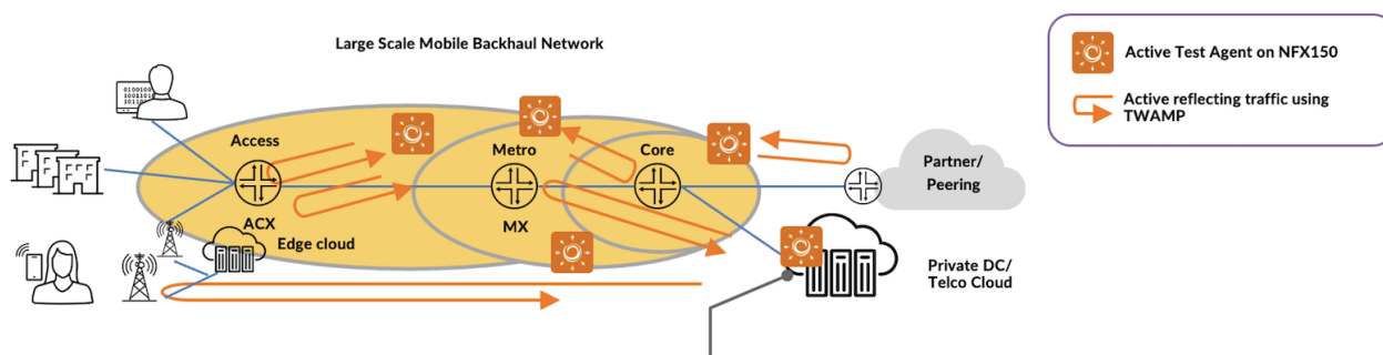
Figure 2: Figure 2. ASEAN mobile operator Routing Active Testing deployment. TAs are run on NFX150
