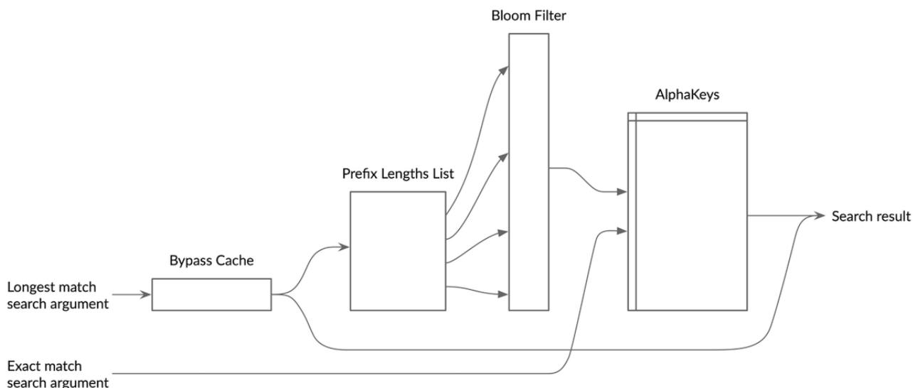
Figure 3: Figure 3 ALPHA (Absolute Longest Prefix Hash Algorithm) Function Block Diagram
