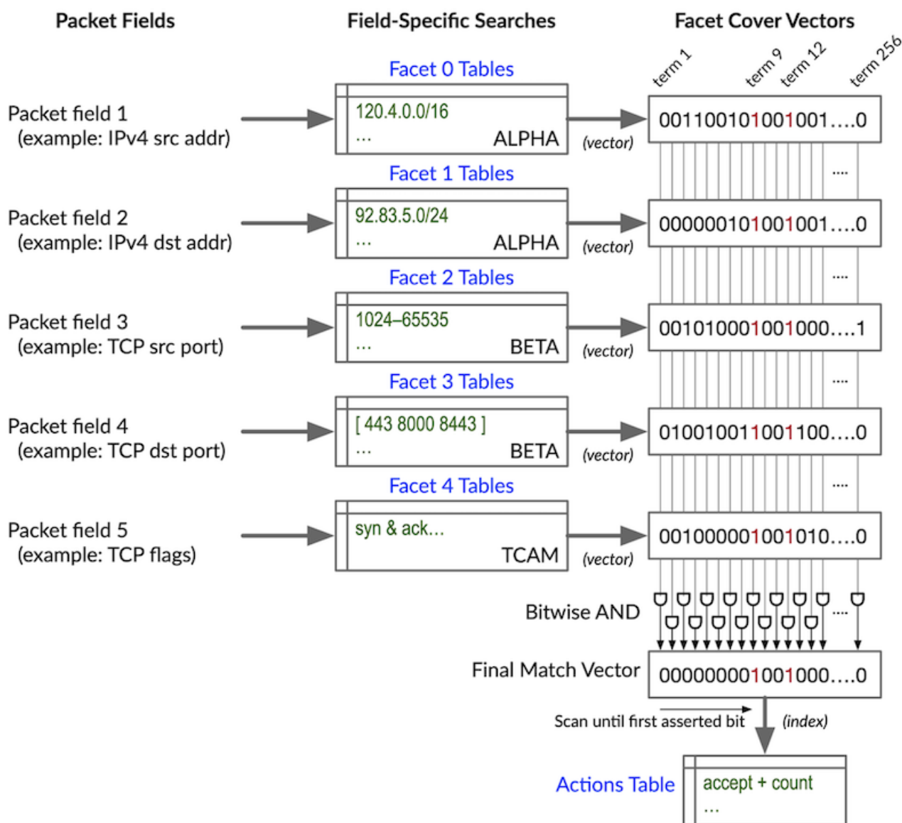
Figure 1: Figure 1 Facet Cover Vector Algorithm Principles
