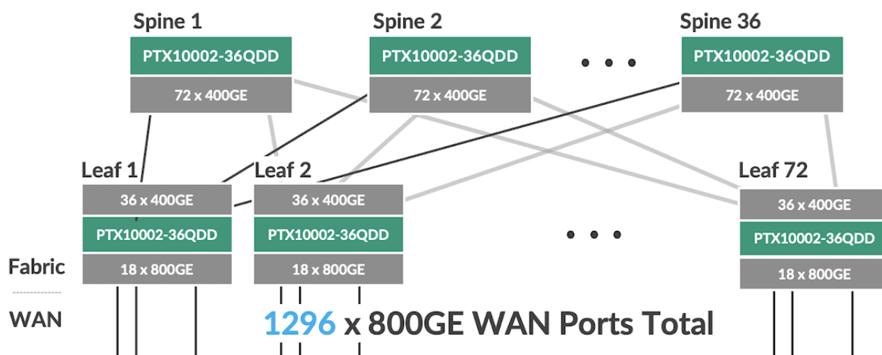
Figure 3: 3-stage WAN Ethernet fabric configuration
