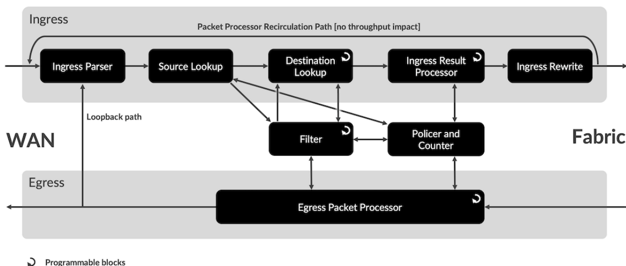
Figure 10: Express 5 Packet Processing Blocks
