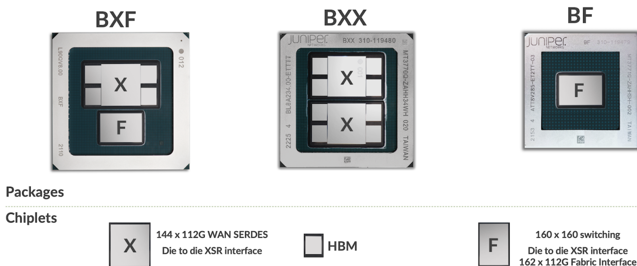
Figure 2: Express 5 Chiplets and Packages, more information in the Hot Chips 34 presentation.
