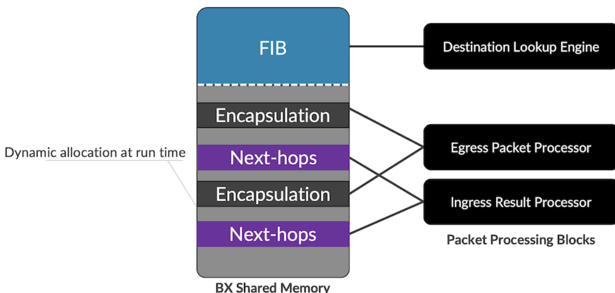
Figure 11: Shared Memory Concept
