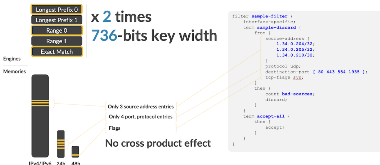
Figure 9: Express 5 Filter Engines and Memories
