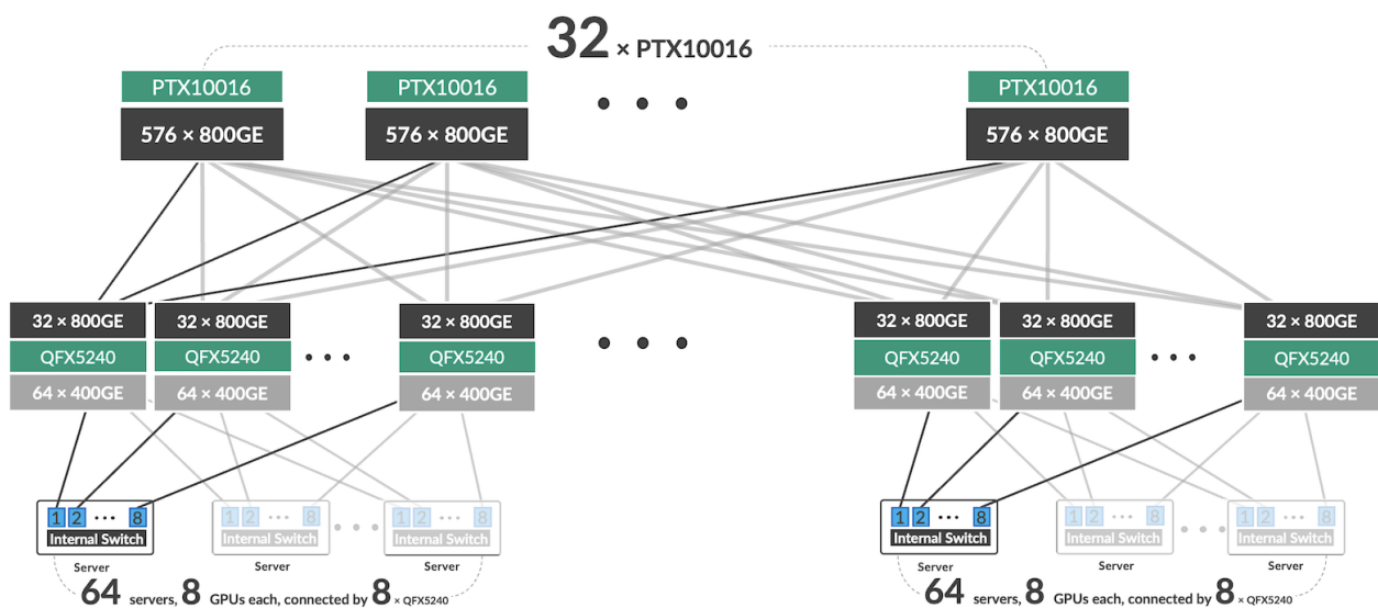
Figure 5: AI/ML Training Cluster GPU Interconnect Network with 36,864 400GE ports. 3-stage fat-tree topology.
