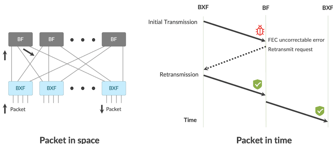
Figure 13: Reliable transmission over Juniper cell-based fabric
