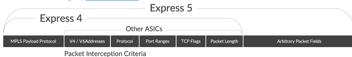
Figure 14: Traffic visibility in the core, interception criteria
