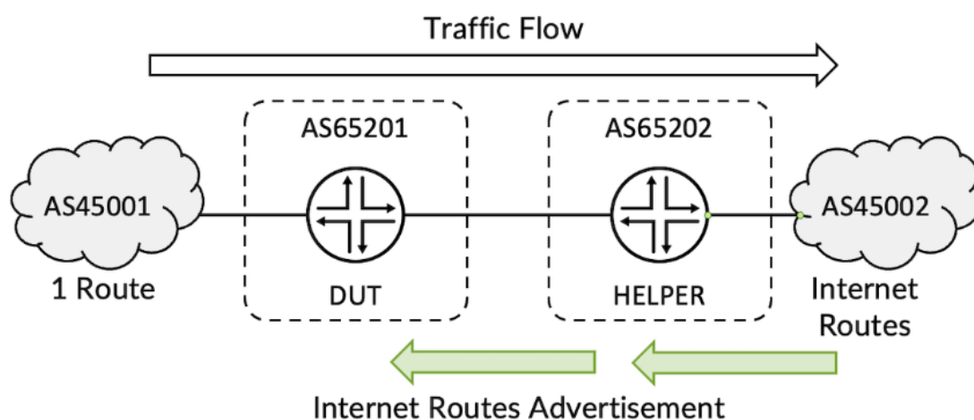
Figure 1: Test topology
