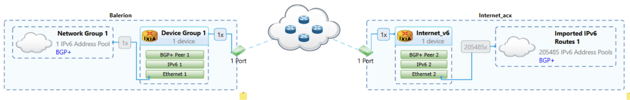
Figure 7: Ixia Configuration for IPv6 Routes
