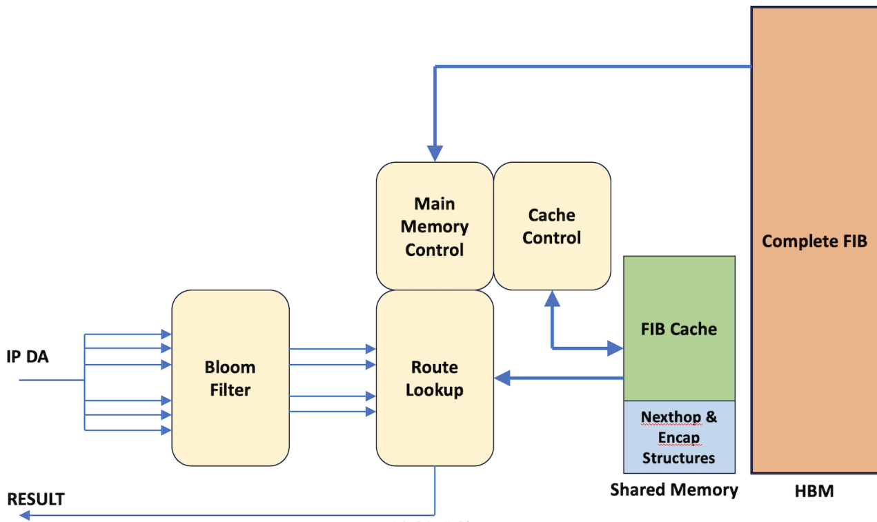
Figure 1: FIB table subsystem
