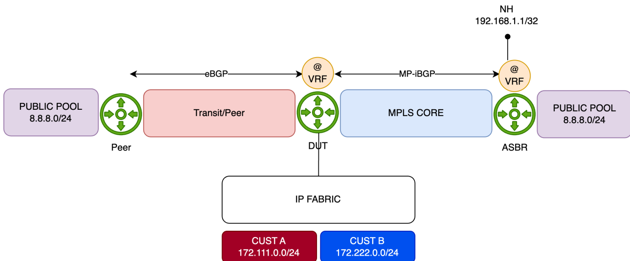
Figure 2: Example 1 - Topology
