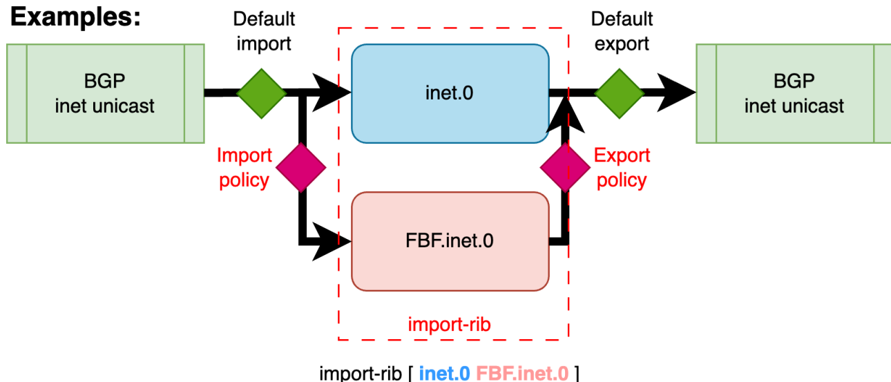
Figure 6: Routes leaking thanks to rib-group feature
