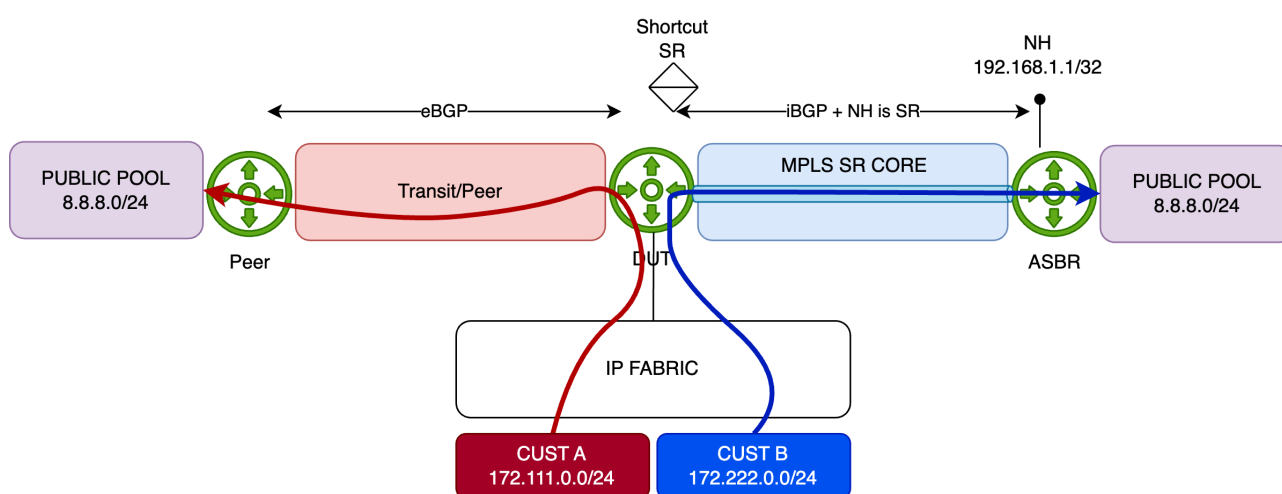
Figure 7: Network topology
