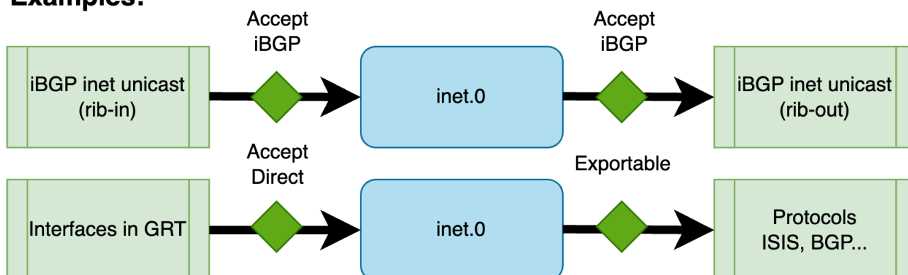
Figure 5: Default routing table management
