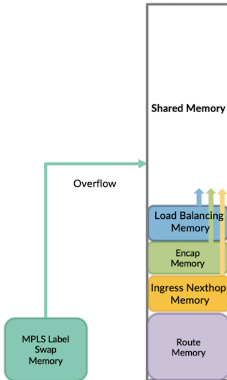
Figure 2: Express 5 Flexible Shared Memory Approach
