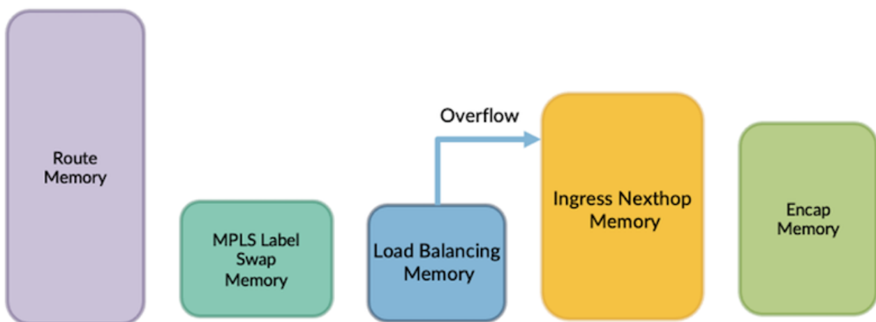
Figure 1: Traditional Pipeline ASICs Memory Allocation
