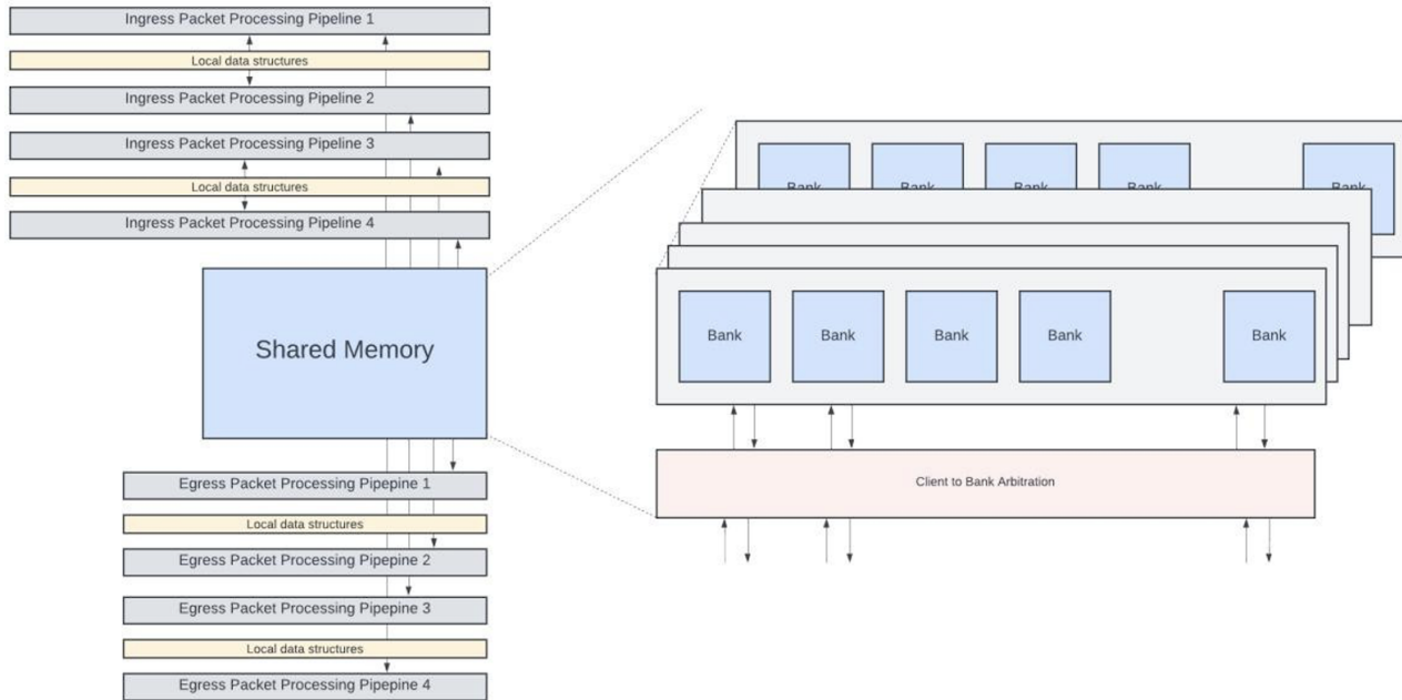
Figure 8: Shared Memory for Large Data Structures
