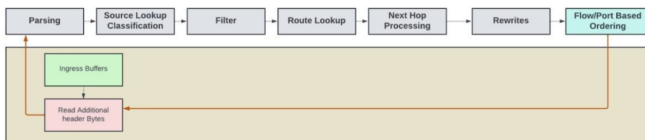
Figure 6: Conceptual diagram illustrating recirculation
