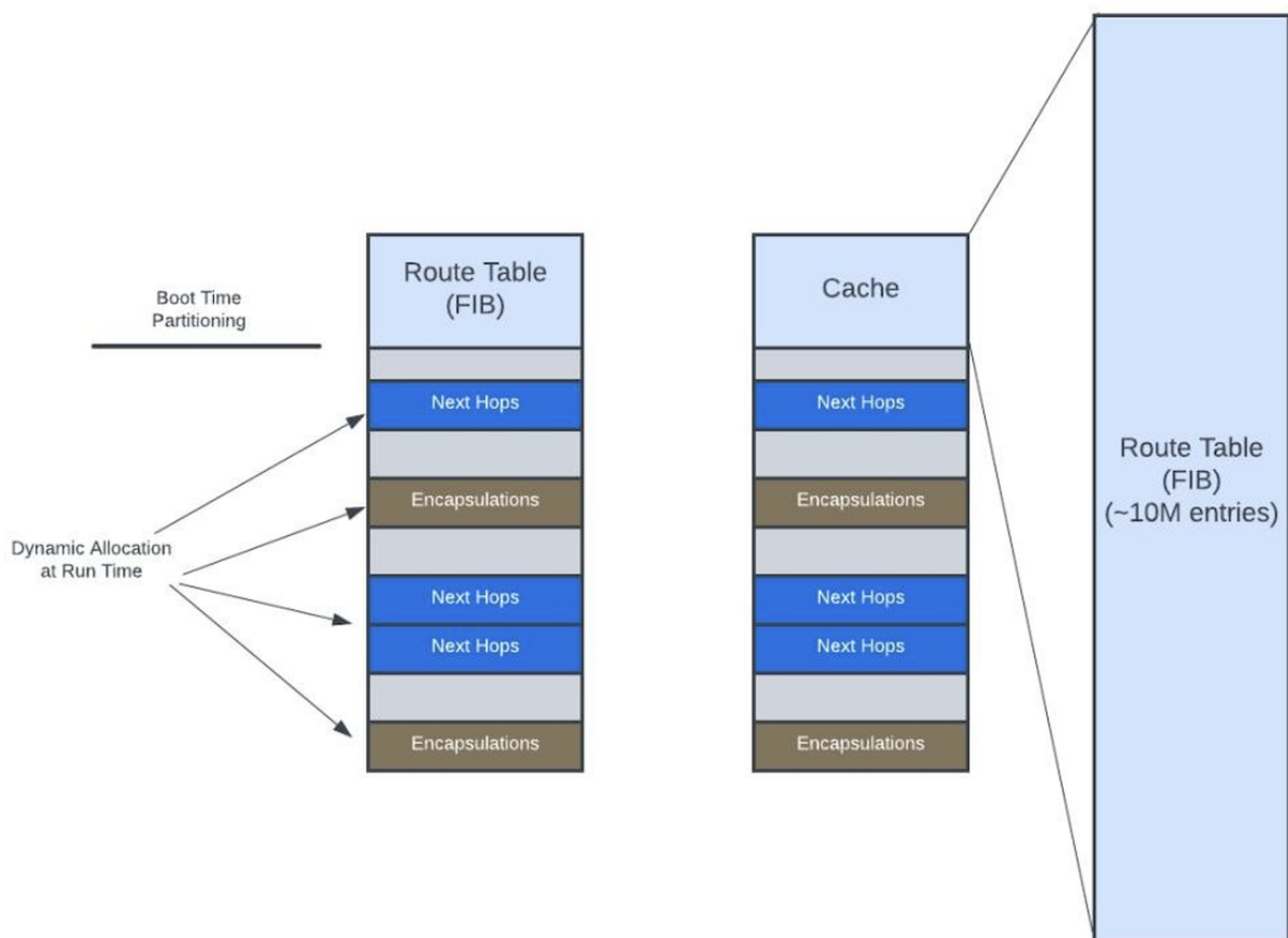
Figure 9: Shared Memory
