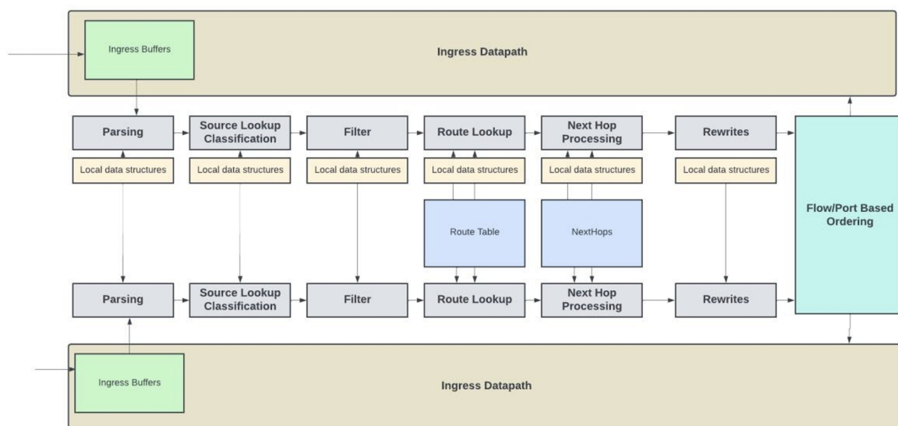
Figure 7: two pipelines
