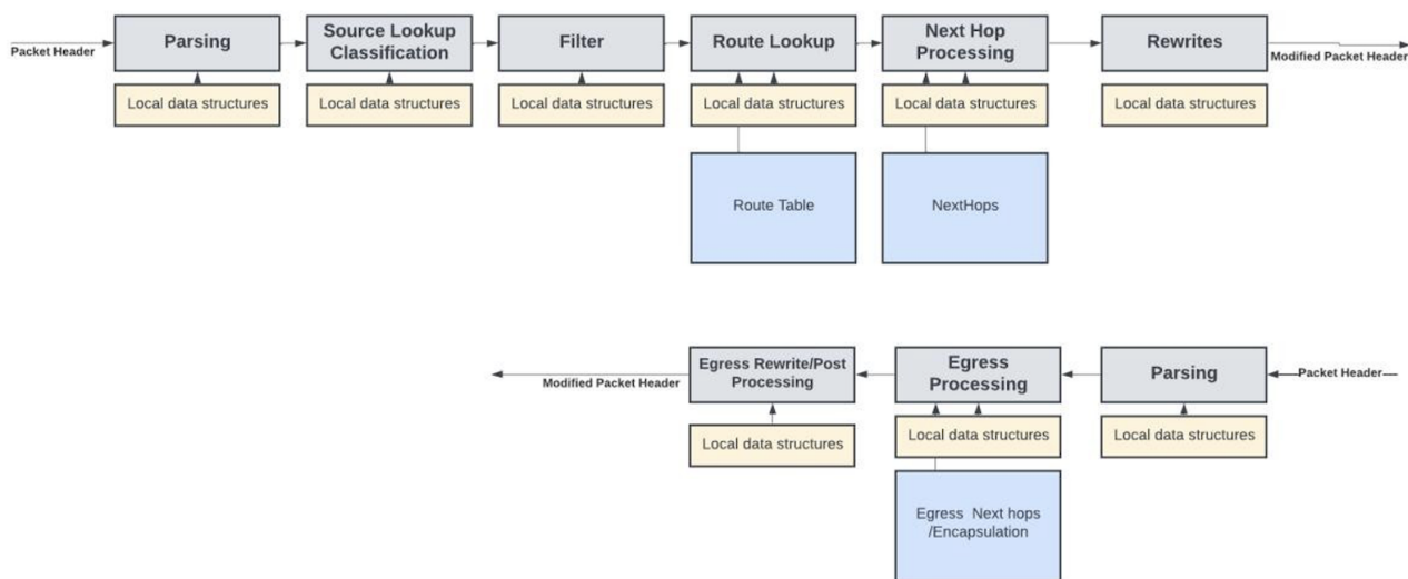
Figure 3: Conceptual diagram of ingress and egress packet processing pipelines with their data structures.
