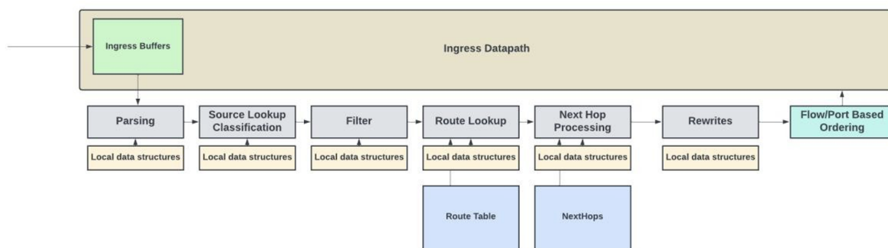
Figure 5: Packet processing pipeline with reorder engine for per-flow packet ordering
