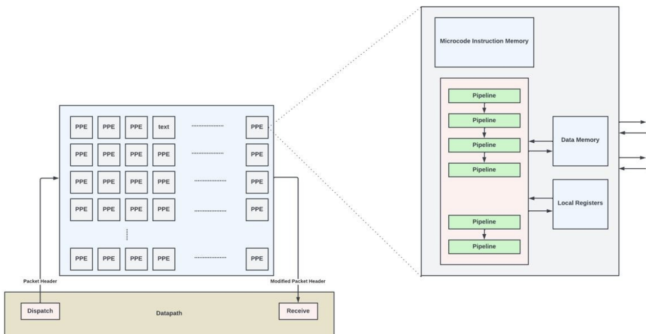
Figure 2: A conceptual diagram that shows how the packets can recirculate within each lookup module.
