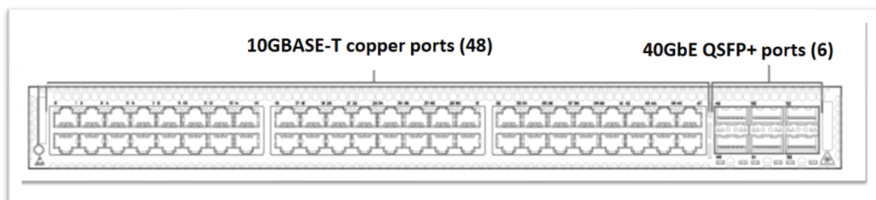
Figure 6: QFX5100-48T
