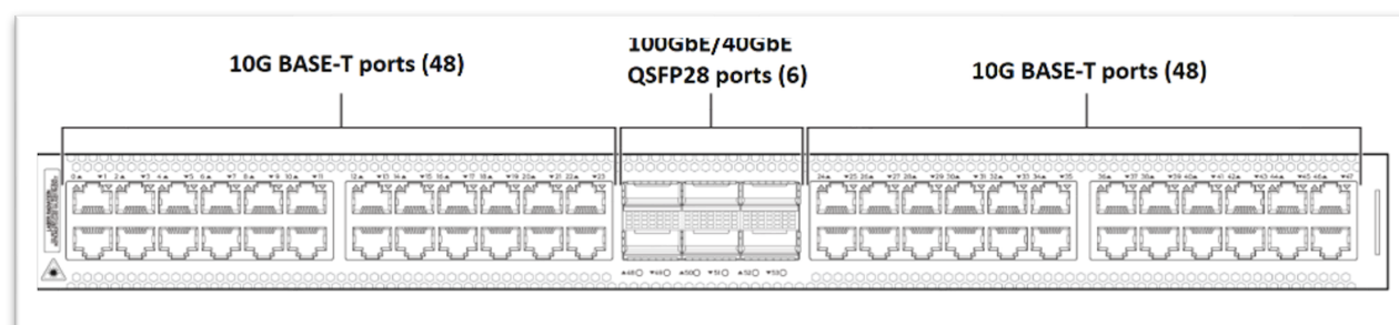
Figure 7: QFX5120-48T
