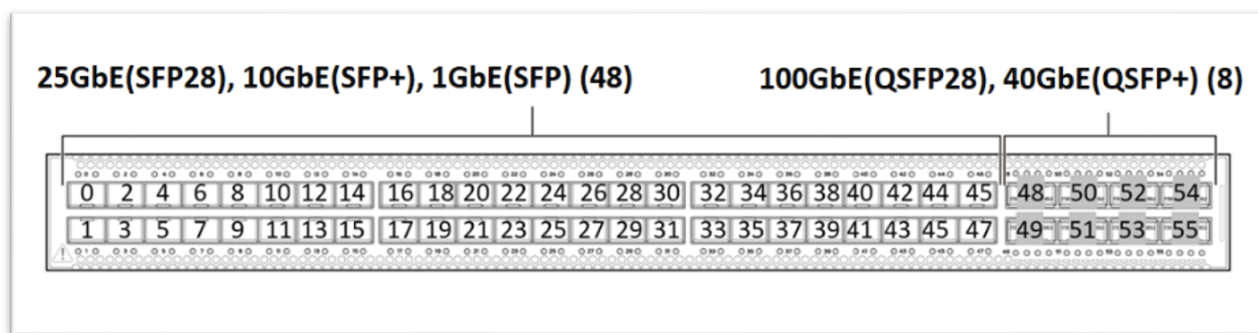
Figure 2: QFX5120-48Y
