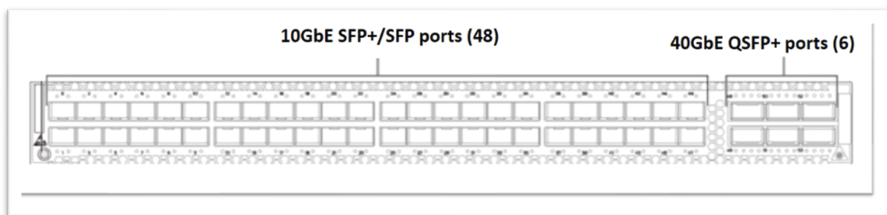
Figure 1: QFX5100-48S
