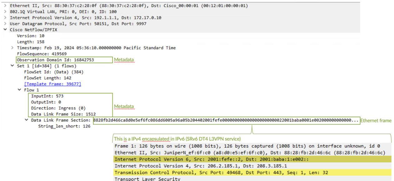
Figure 7: Example of a IMON flow record
