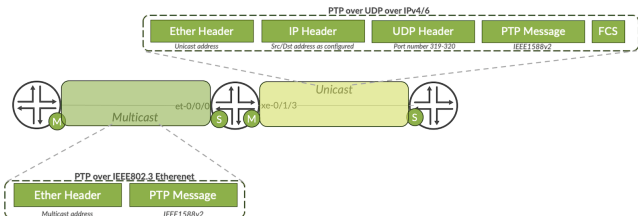
Figure 5: G.8275.1.ENH with one side PTPoEth and another PTPoIP
