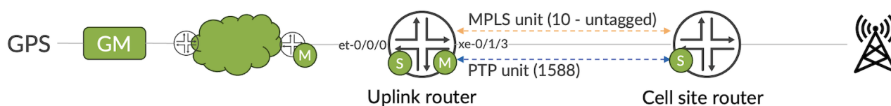
Figure 2: PTP with VLAN
