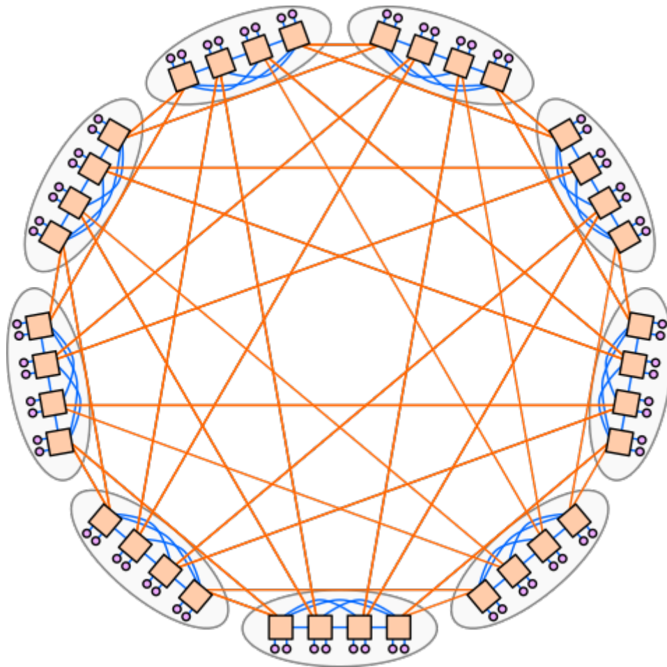
Figure 18: Dragonfly Topology Example.
