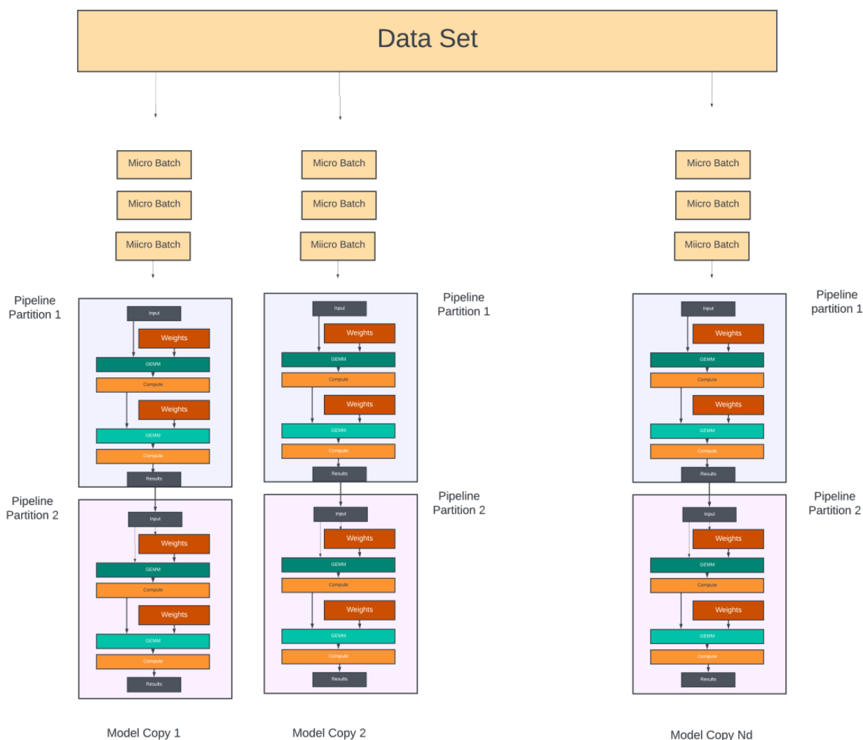
Figure 5: A conceptual example of pipeline and data parallelism (with two pipeline stages for each model copy).
