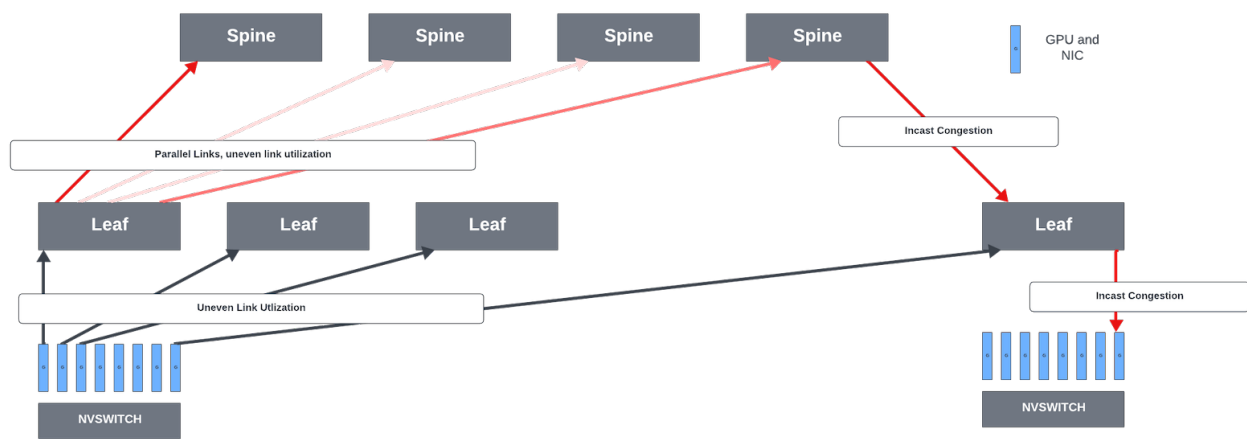
Figure 19: Network congestion points
