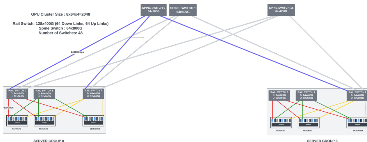
Figure 14: 2048 GPU Cluster with rail-spine switches. No oversubscription between leaf and spine links
