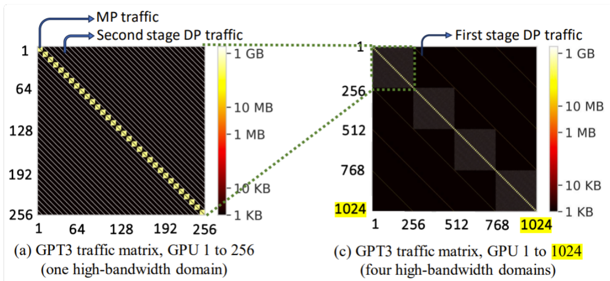
Figure 11: Traffic pattern between GPU pairs when training a GPT-3 model
