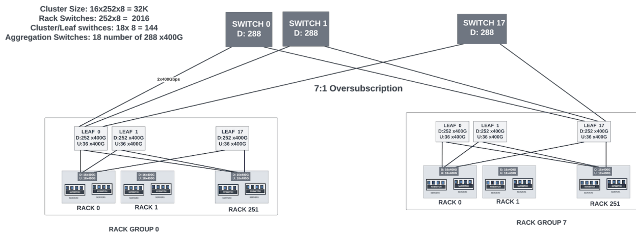
Figure 16: A 32K cluster from Meta (as seen in the At-Scale conference).
