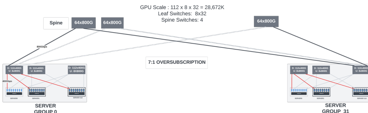
Figure 15: 28K cluster. 7:1 Oversubscription at the cluster (server group) to spine links.
