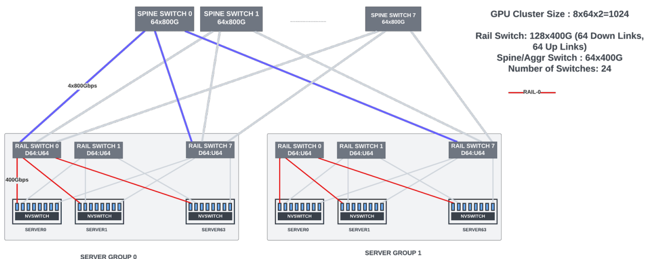
Figure 13: A CLOS topology for 1024 GPU cluster with rail and spine switches. Spine-leaf links are not oversubscribed
