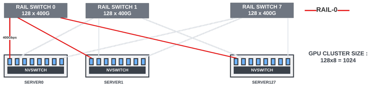
Figure 12: 1024 GPU cluster with rail-only switches
