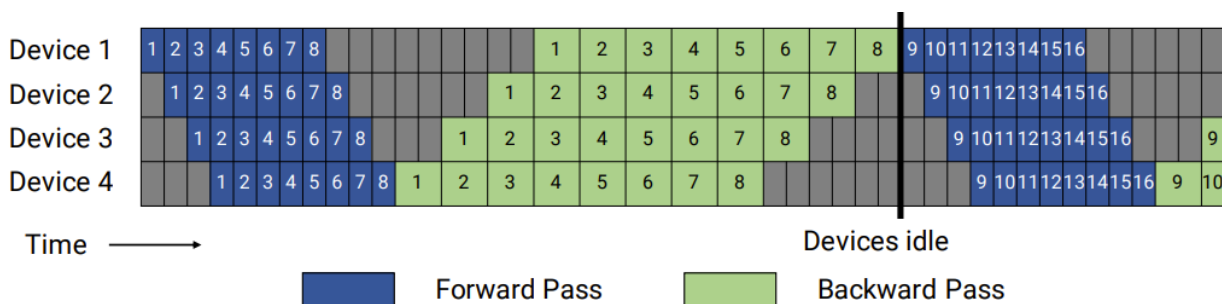
Figure 6: Illustration of pipeline parallelism and the bubbles (gray regions)
