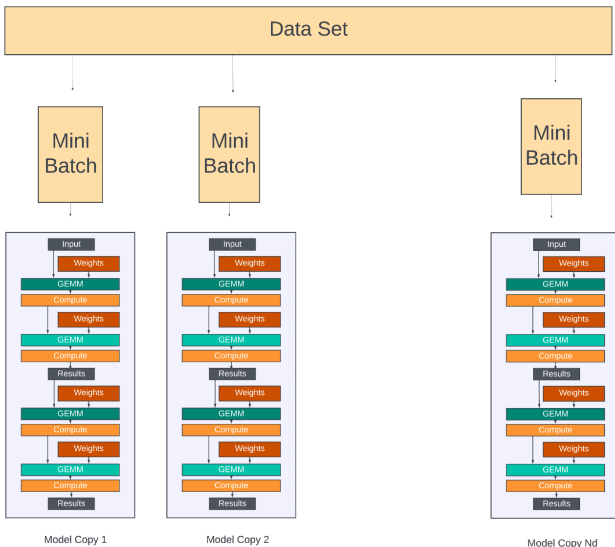
Figure 4: A conceptual example of data parallelism. GEMM is a matrix multiplication unit.
