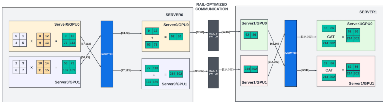
Figure 9: Row parallelism with rail-optimized data communication between two servers
