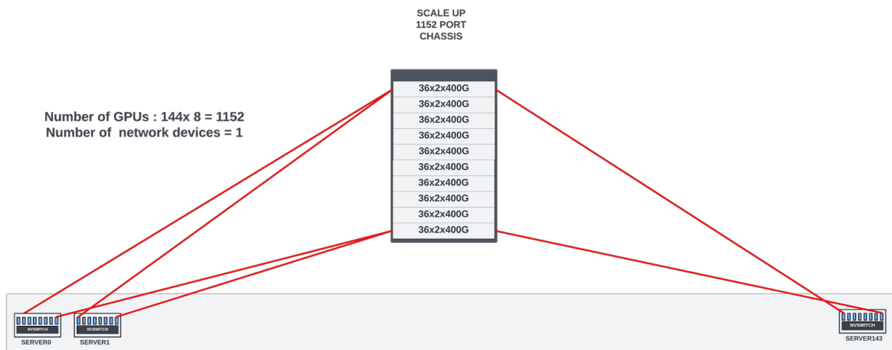
Figure 17: Conceptual Diagram of 1152 GPU cluster with a modular system
