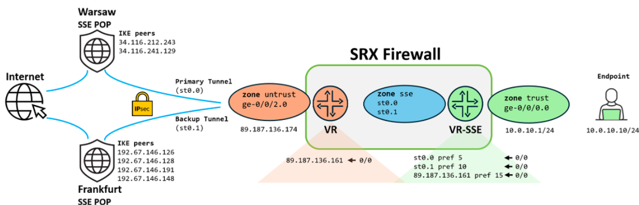
Figure 2: Demo topology layout
