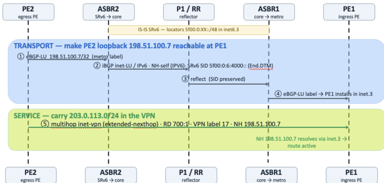
Figure 3: Control-plane establishment: transport first, then service
