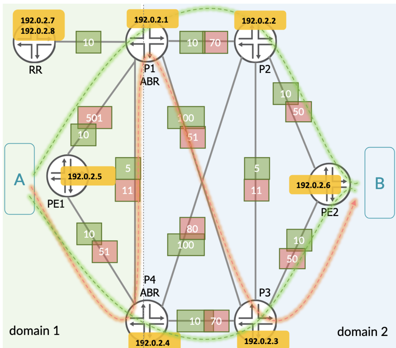
Figure 1: Inter-domain on-demand SR-TE LSPs with BGP-LS Topology
