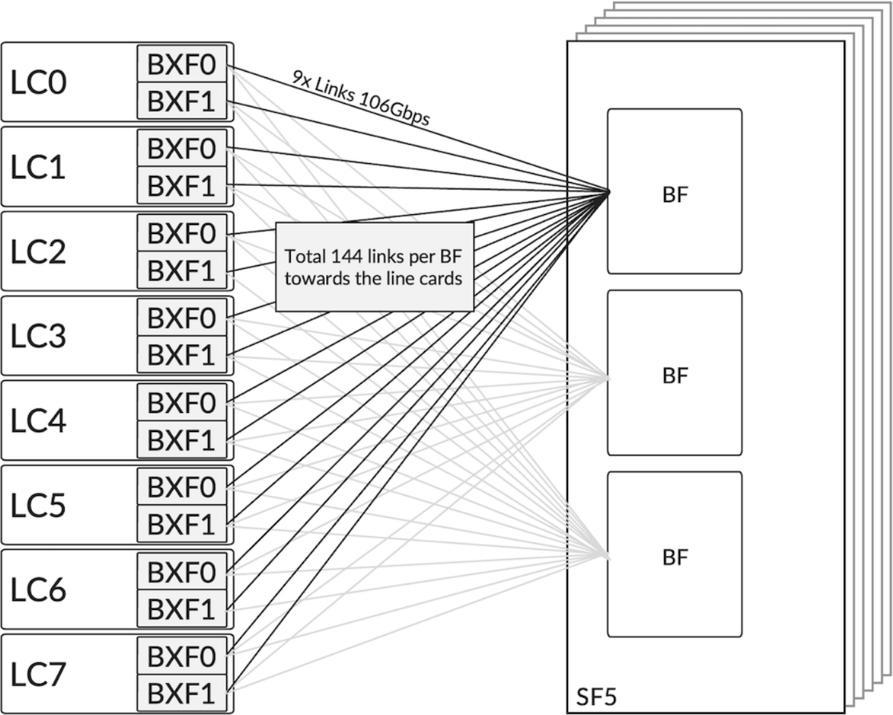
Figure 18: Full Mesh connectivity from one SF5 card’s perspective
