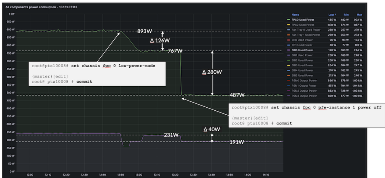
Figure 30: Low power mode + pfe-instance power off
