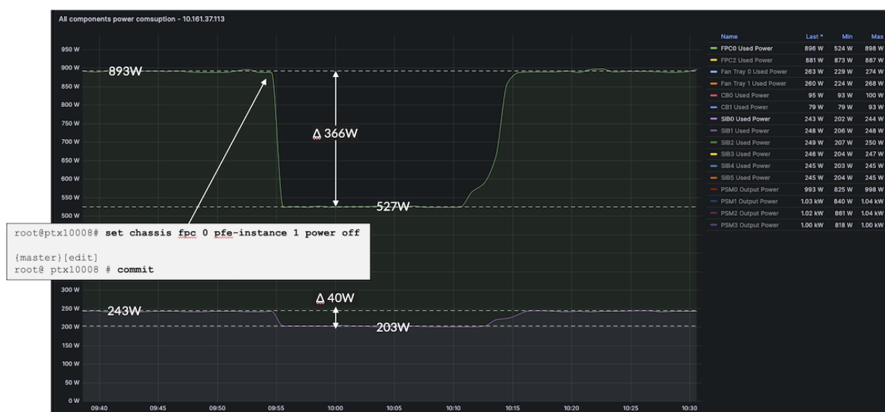
Figure 27: Power saved by turning off one PFE on LC1301
