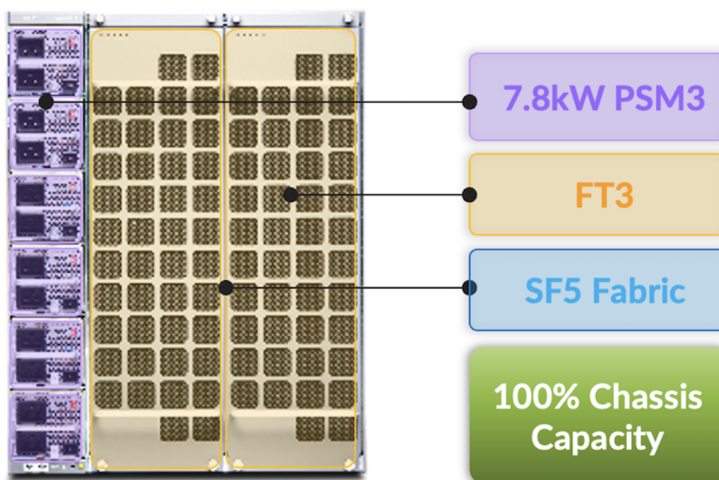
Figure 16: LC1301 capacity with new v3 power modules and fans, + new SF5 Fabric
