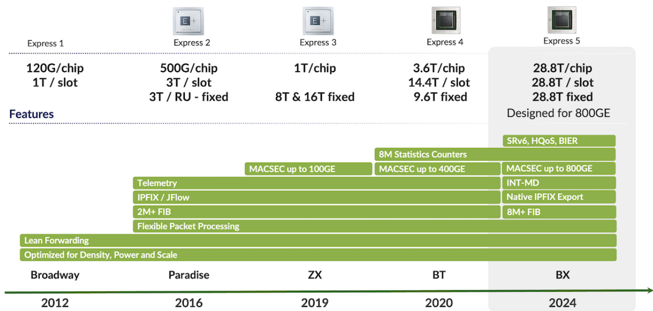
Figure 3: Express Packet Forwarding Engine Generations
