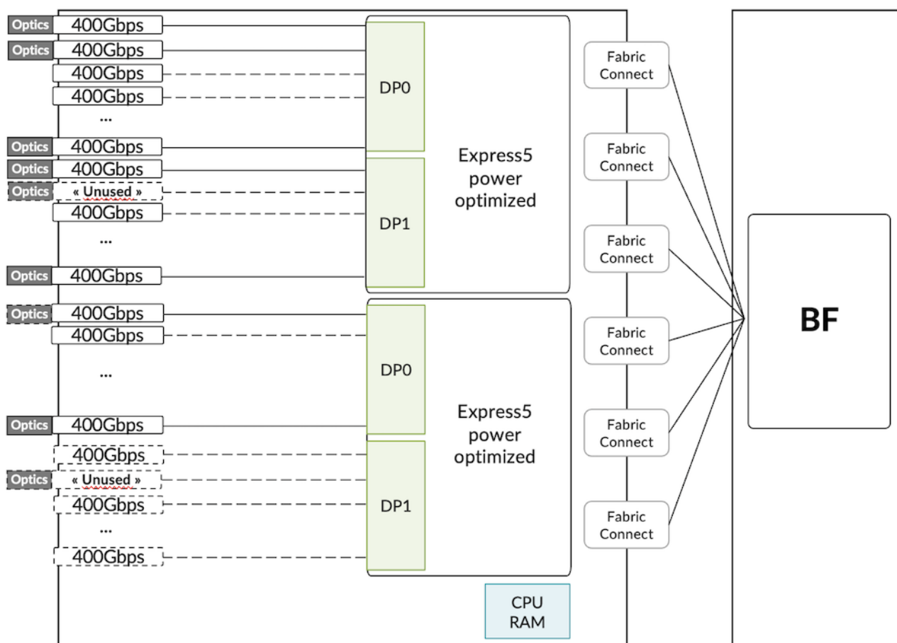
Figure 28: Low power mode configured on LC1301
