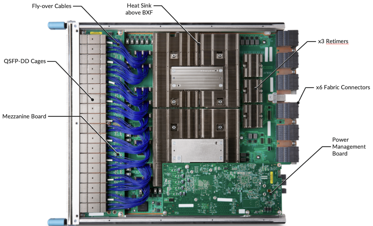
Figure 8: LC1301 Picture
