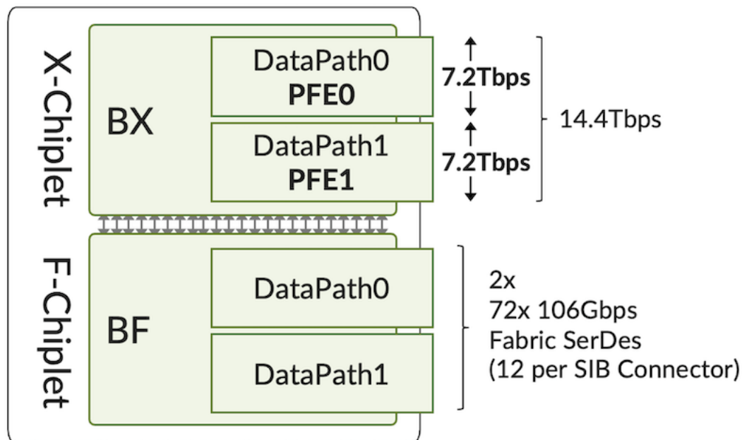
Figure 6: Express 5 BXF Chiplets and DataPaths
