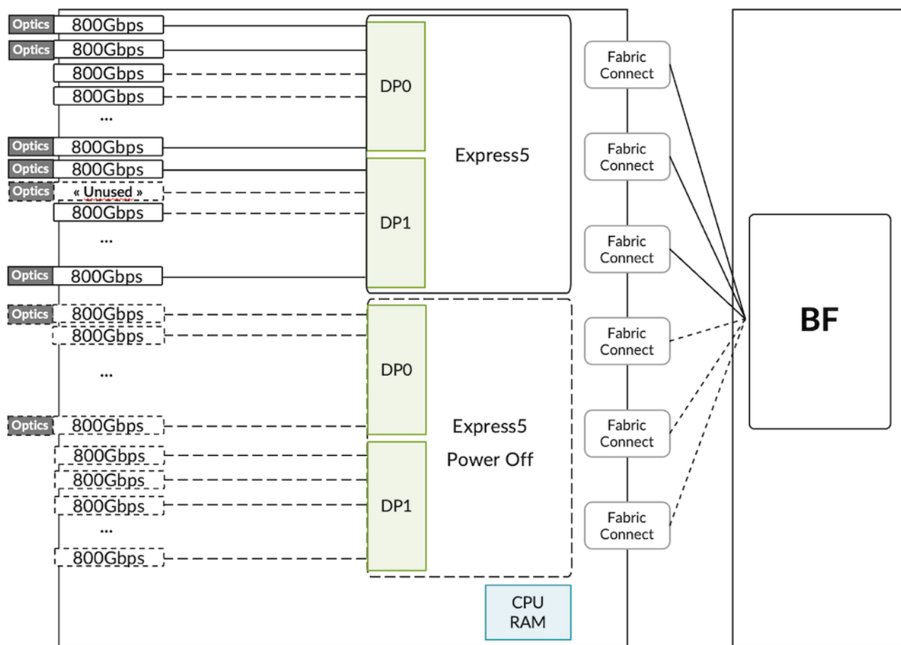
Figure 26: Impact of Express5 powered off
