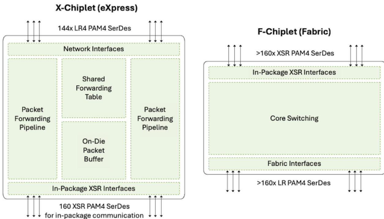
Figure 4: The Building Bricks of Express 5 ASIC Family: X-chiplet and F-chiplet
