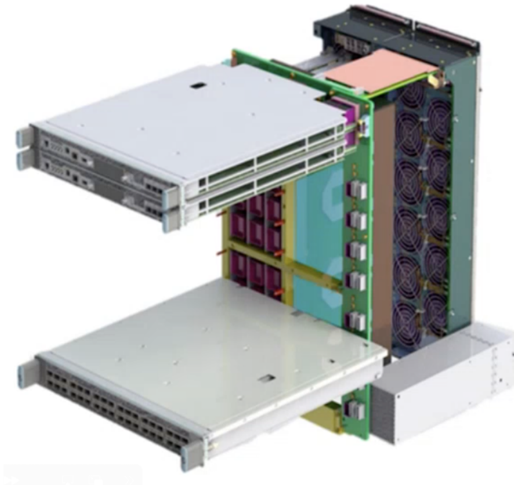
Figure 2: PTX 8-slot Chassis Illustration
