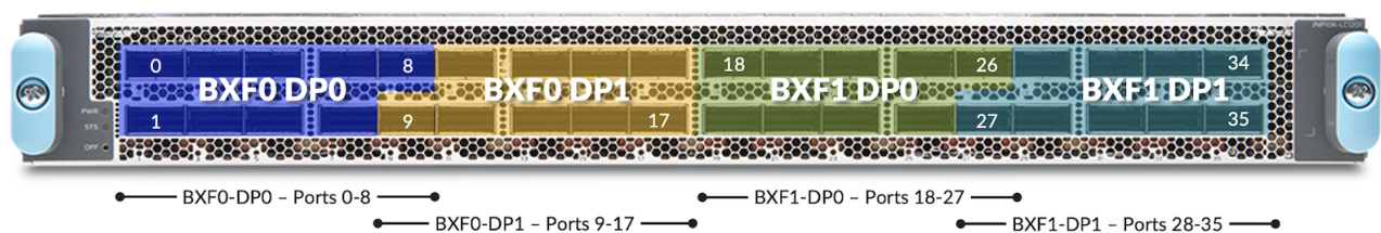
Figure 9: LC1301 PFEs and Port Numbers
