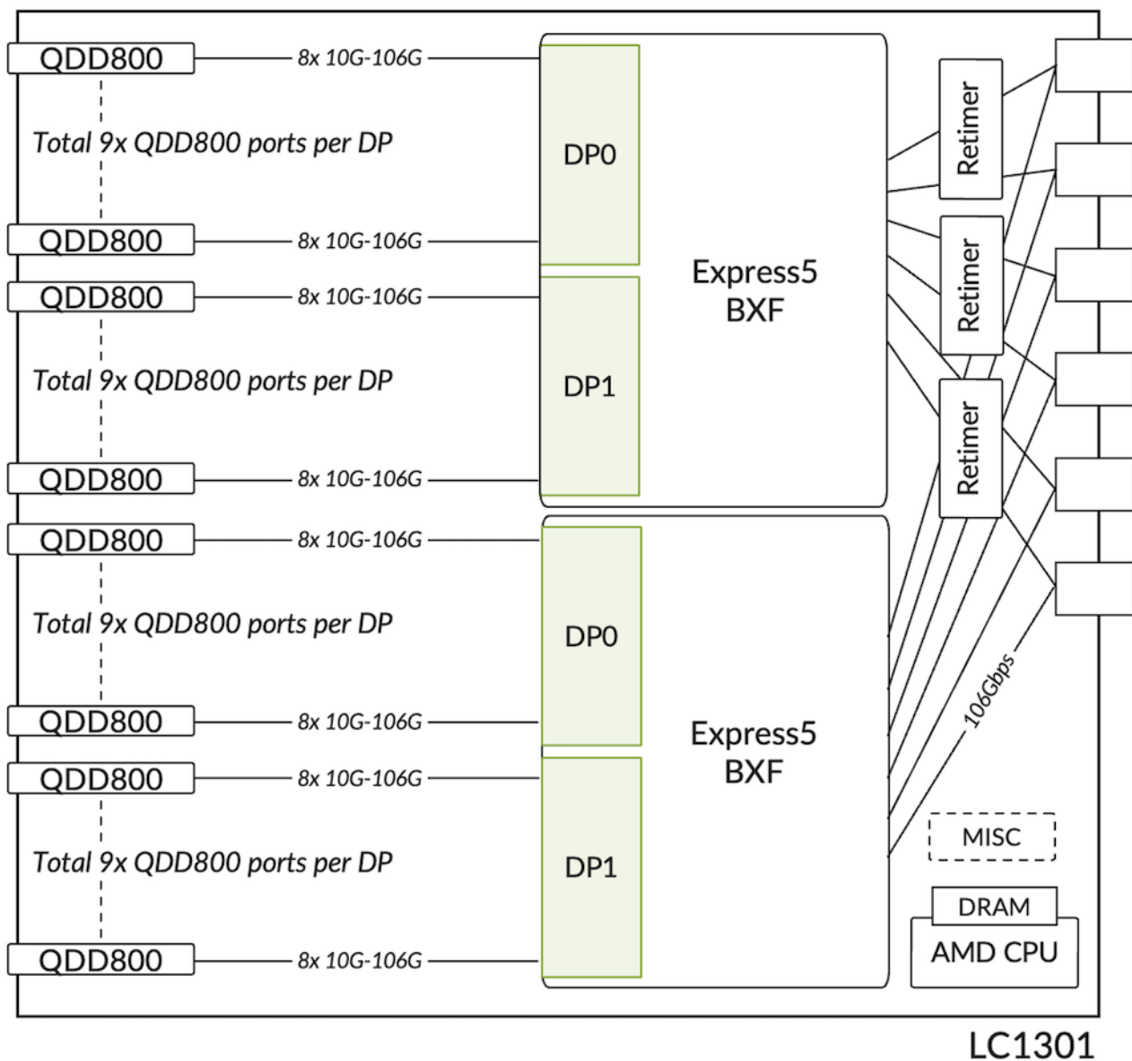
Figure 7: High-Level Block Diagram of an LC1301
