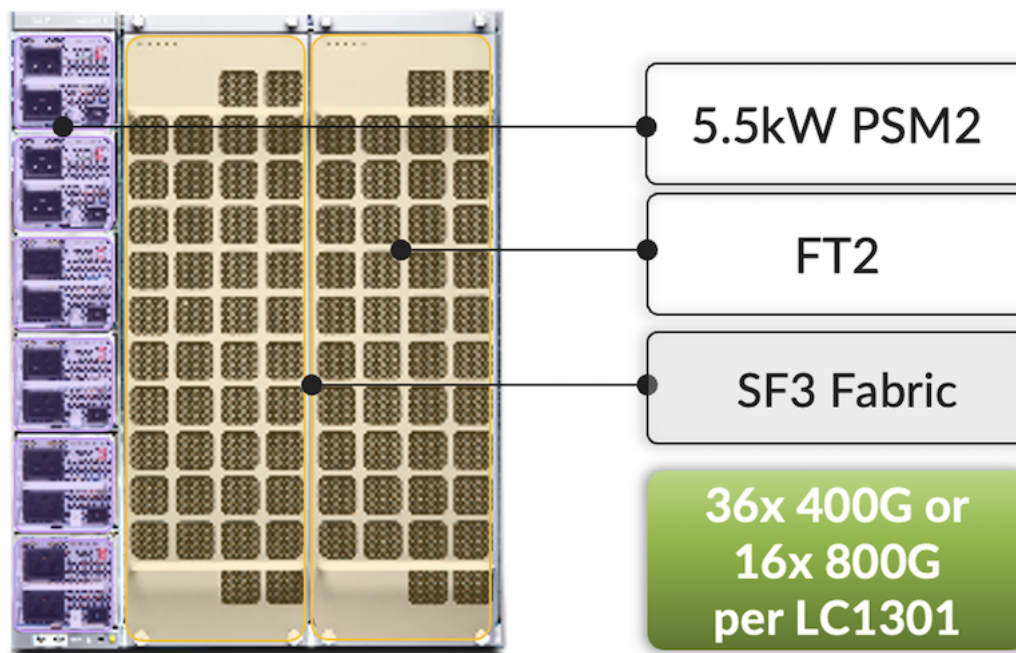
Figure 14: LC1301 capacity with existing v2 power modules, fans and SF3 Fabric
