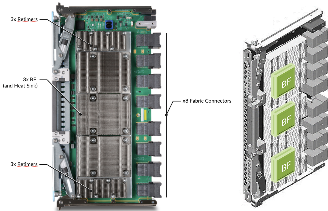
Figure 17: PTX10008 new SF5 Fabric Cards
