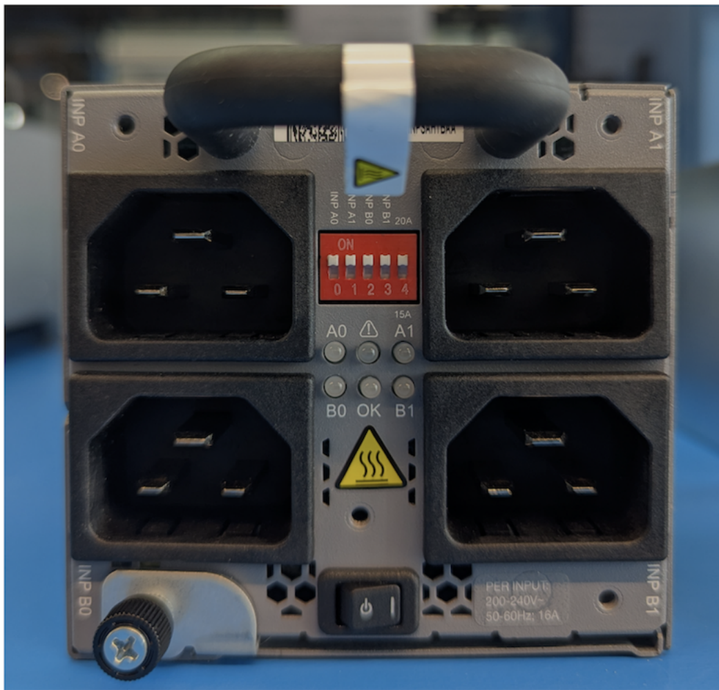
Figure 23: Front view of the PSM3 AC and the dipswitches
