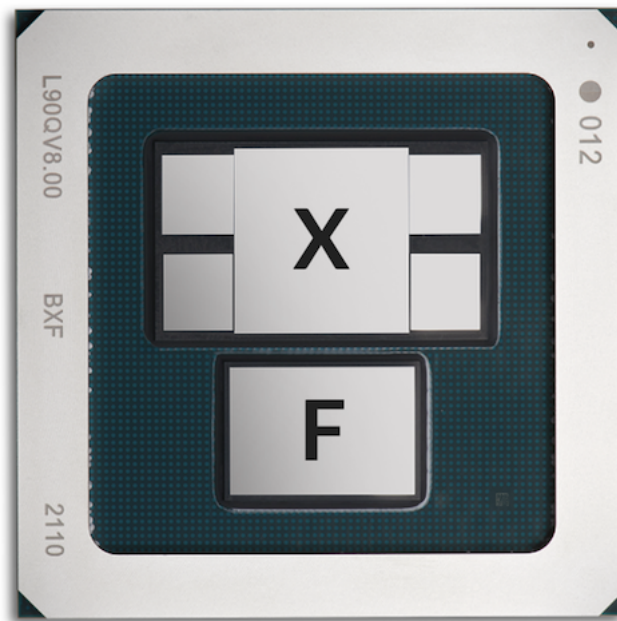
Figure 5: Express 5 Forwarding ASIC in BXF Configuration
