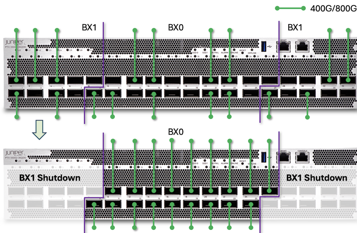
Figure 19: Optimal Port Position to Allow BX1 Power Off
