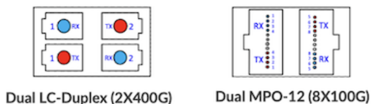
Figure 10: New 800G “Paired Connectors”
