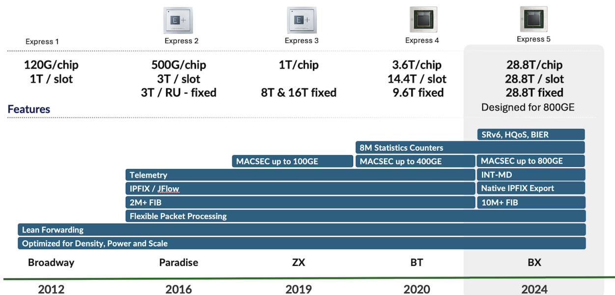
Figure 2: Express Packet Forwarding Engine Generations
