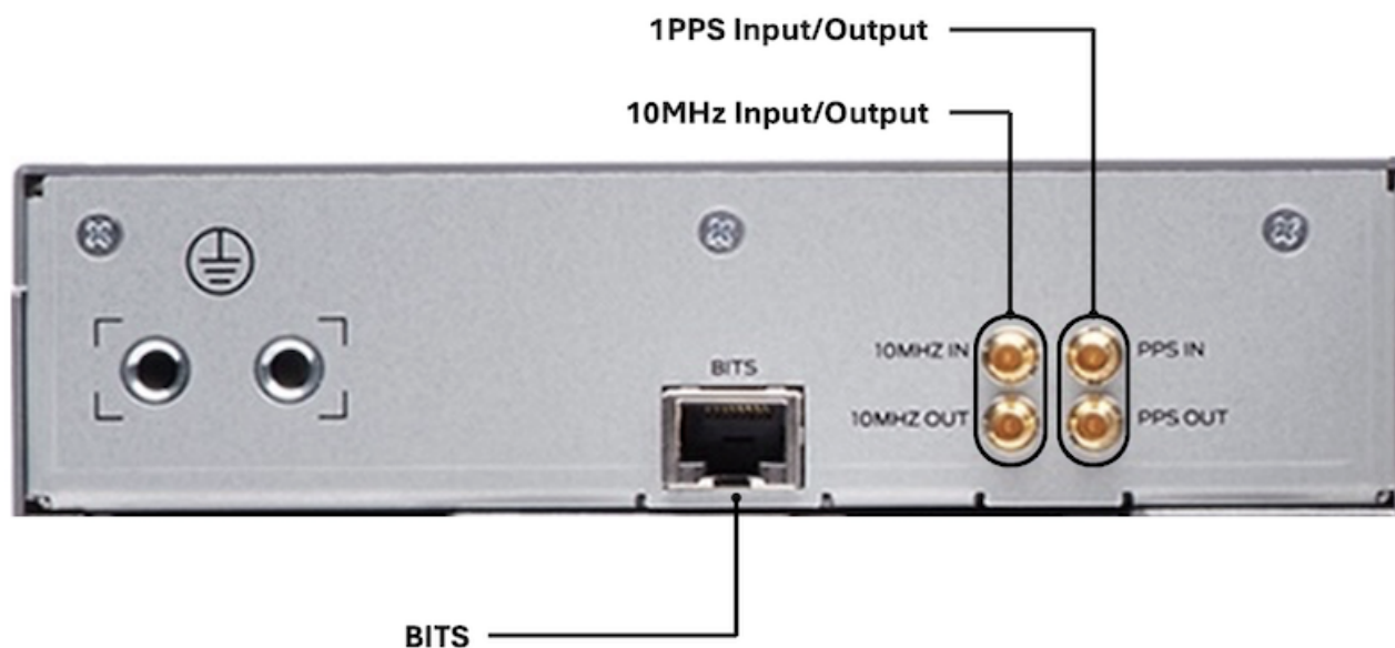
Figure 11: Timing Ports on the Rear Side of the Router
