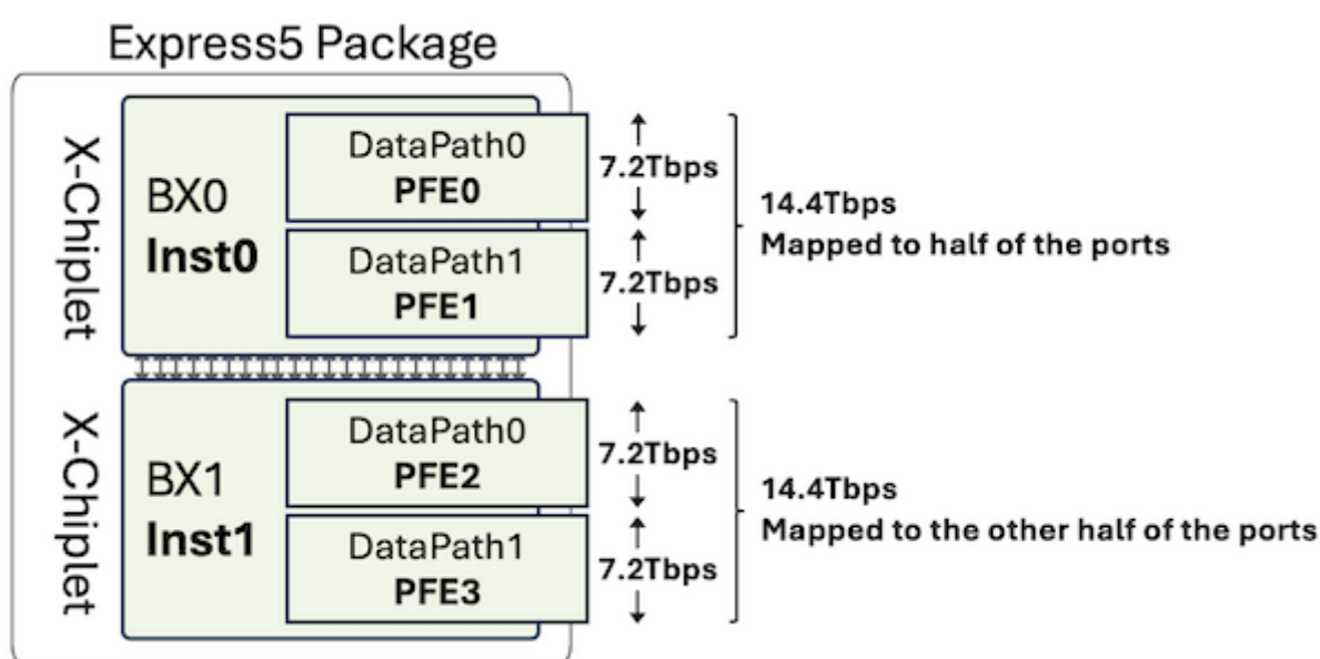
Figure 5: Express 5 BXX Chiplets and Datapaths
