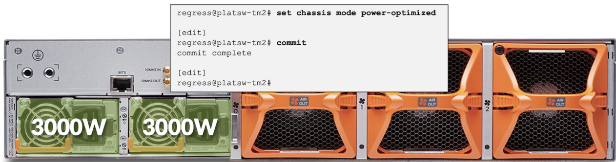
Figure 14: PTX10002-36QDD in Power-Optimized Mode with 3000W PSM
