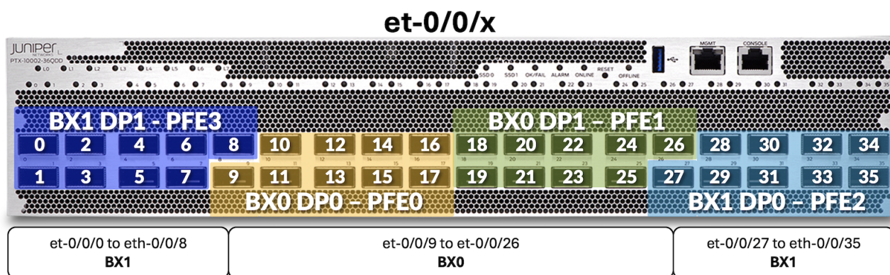
Figure 8: Port Mapping to Chiplet Dies and Datapaths
