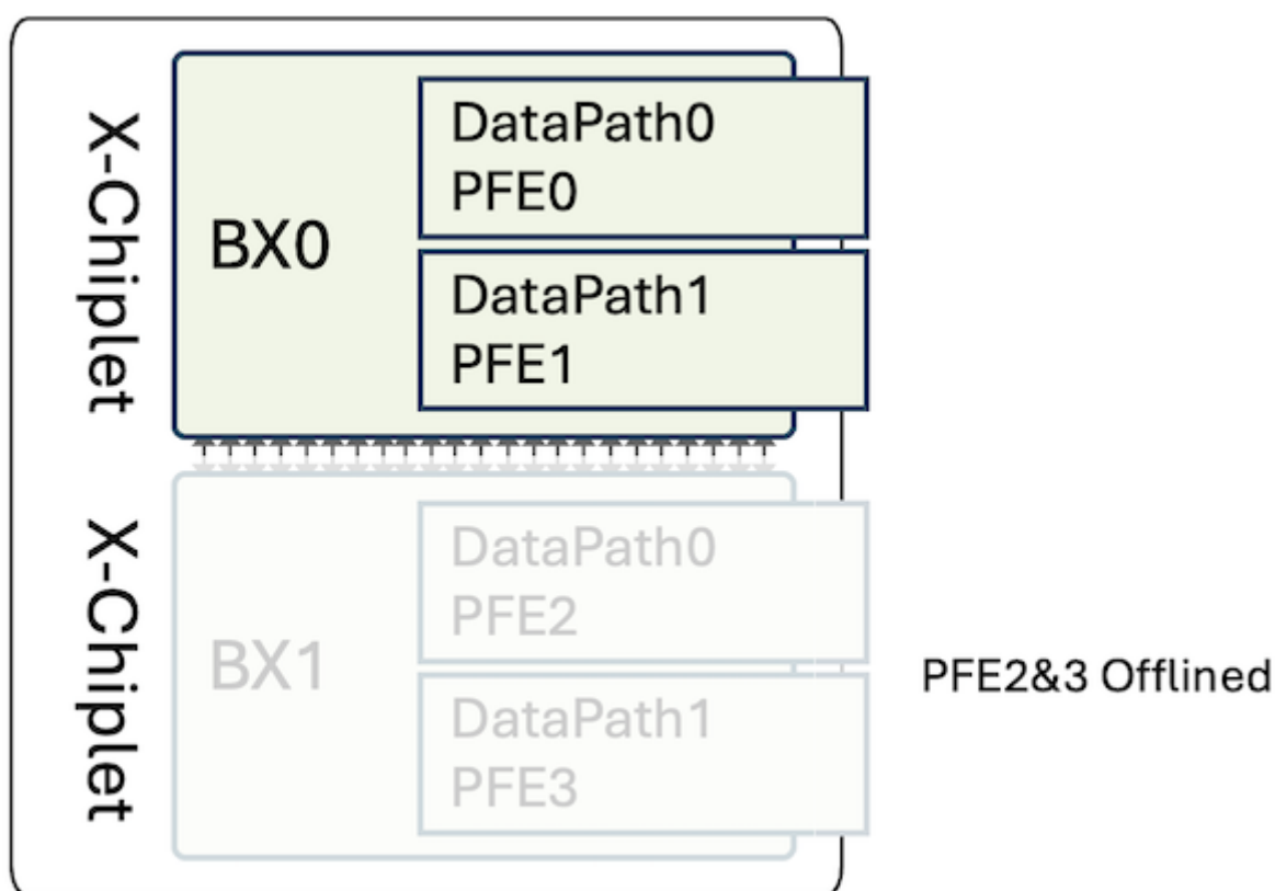
Figure 16: Express 5 BXX with one X-Chiplet Powered Off
