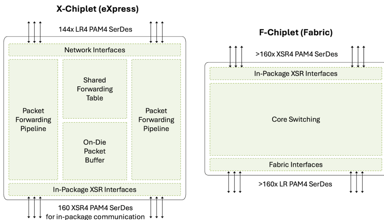
Figure 3: The Building Bricks of Express 5 ASIC Family: X-chiplet and F-chiplet
