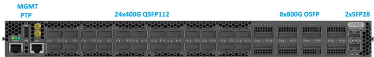
Figure 2: QFX Front Panel
