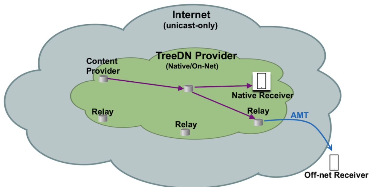
Figure 1: TreeDN Architecture
