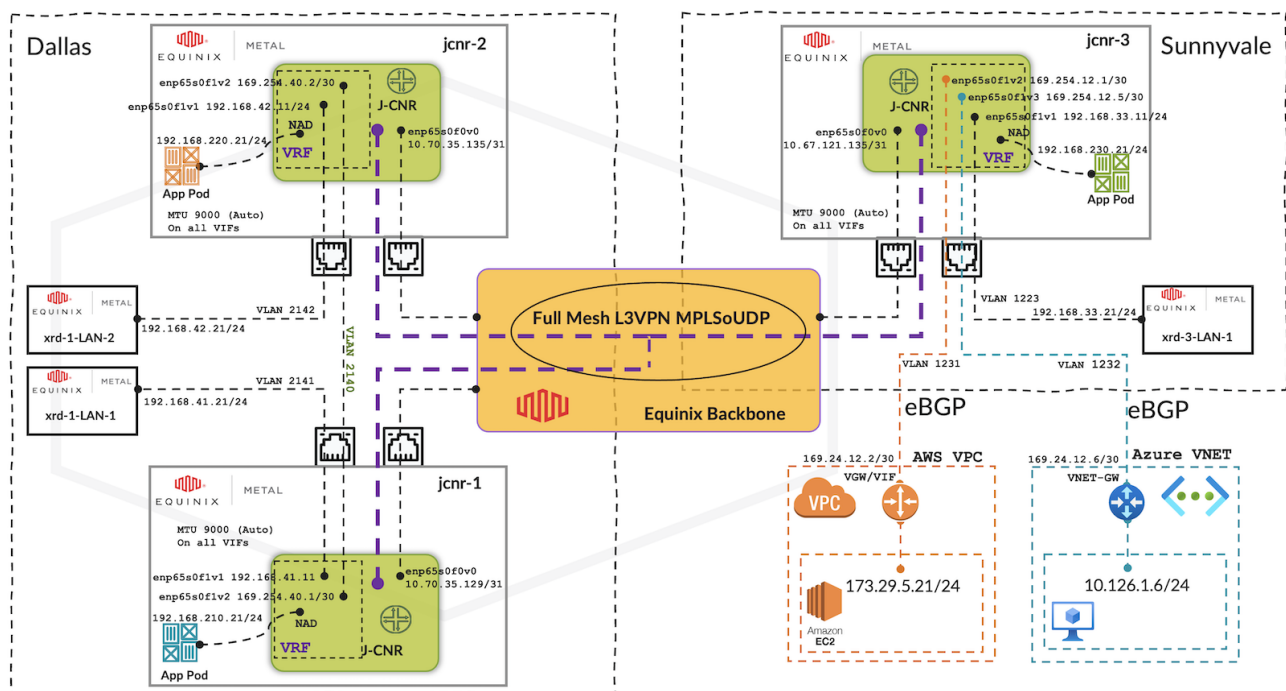
Figure 2: Solution topology and architecture
