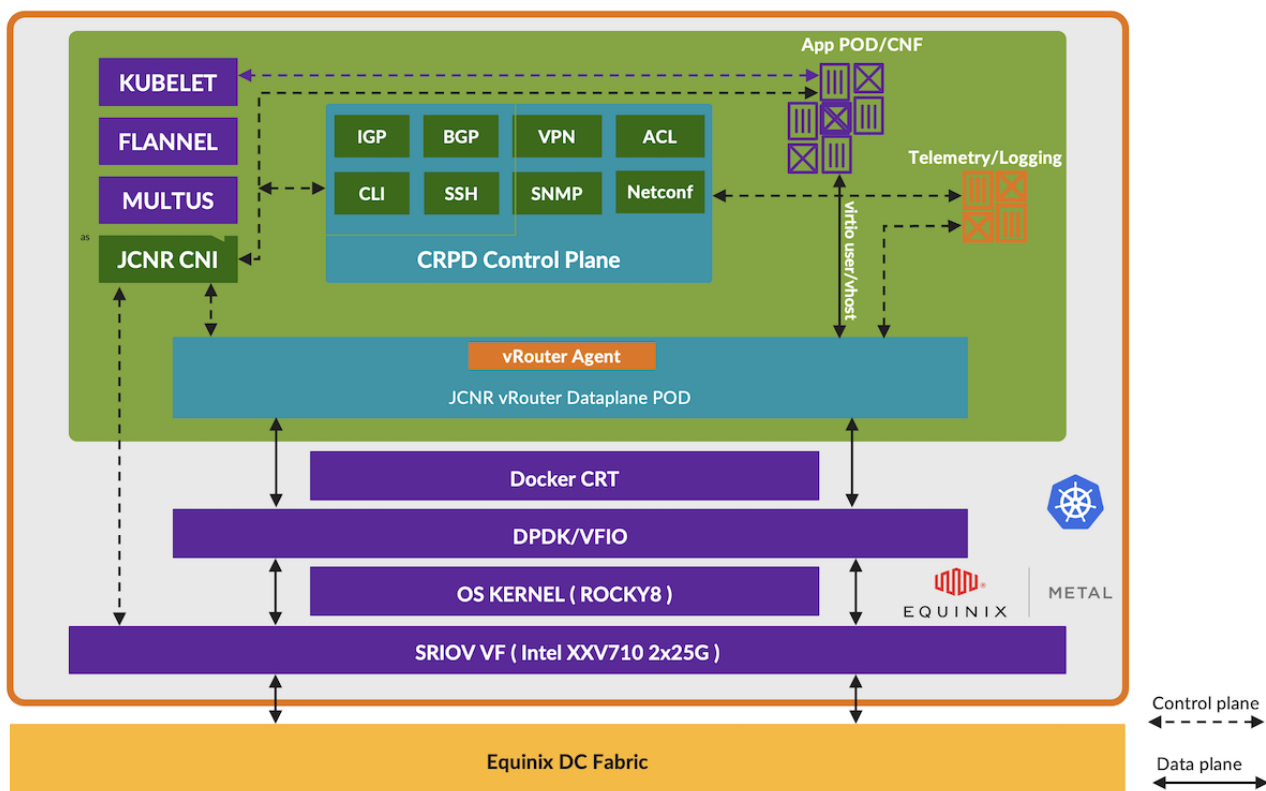
Figure 1: JCNR Equinix Architecture
