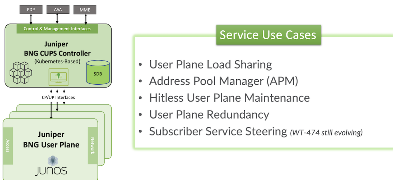
Figure 9: Juniper BNG CUPS use cases
