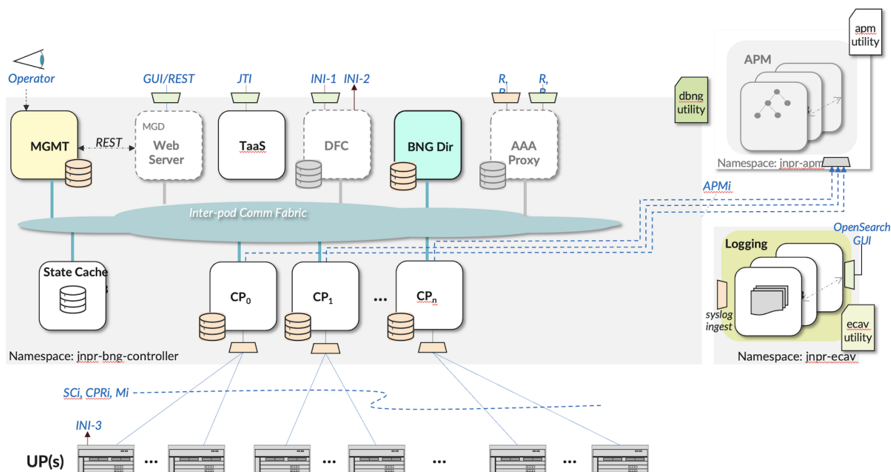
Figure 6: Juniper BNG CUPS Controller Software Architecture
