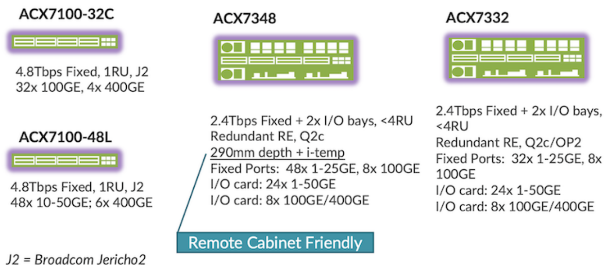
Figure 8: ACX Platform Families Supporting BNG User Planes
