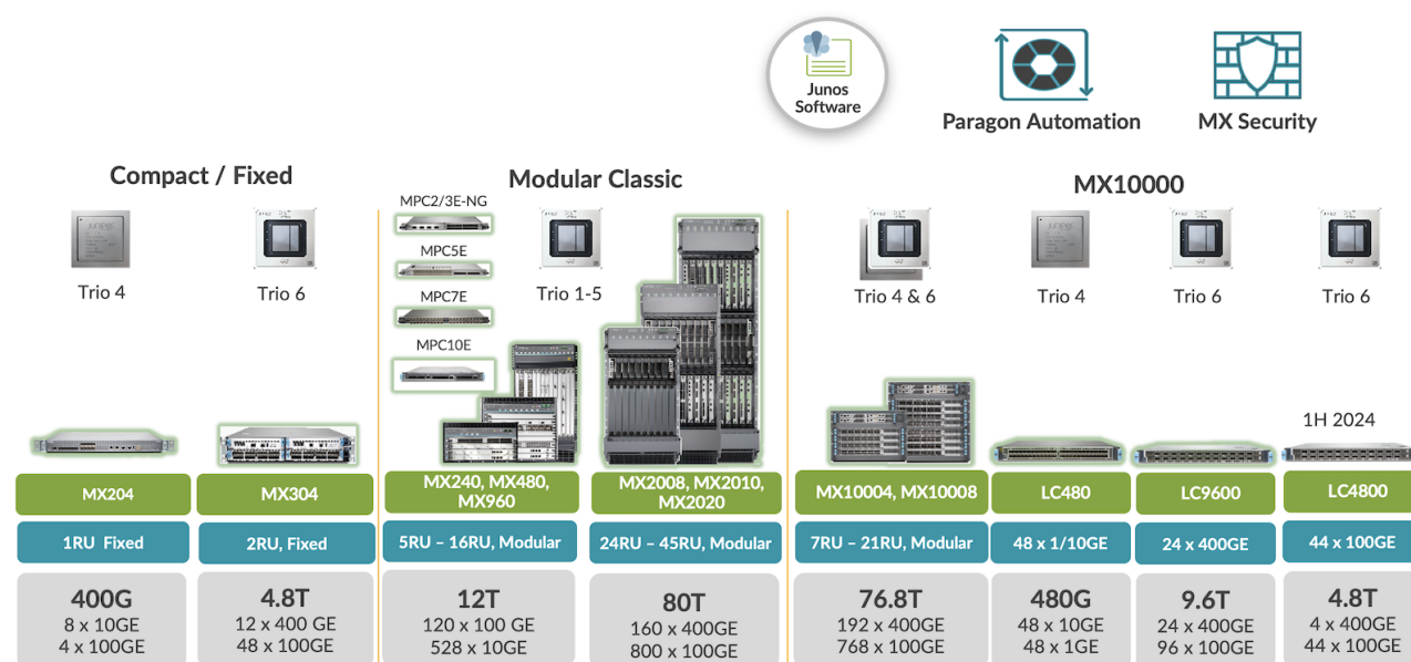
Figure 7: Juniper MX Platforms and Line Cards Supporting the BNG User Planes
