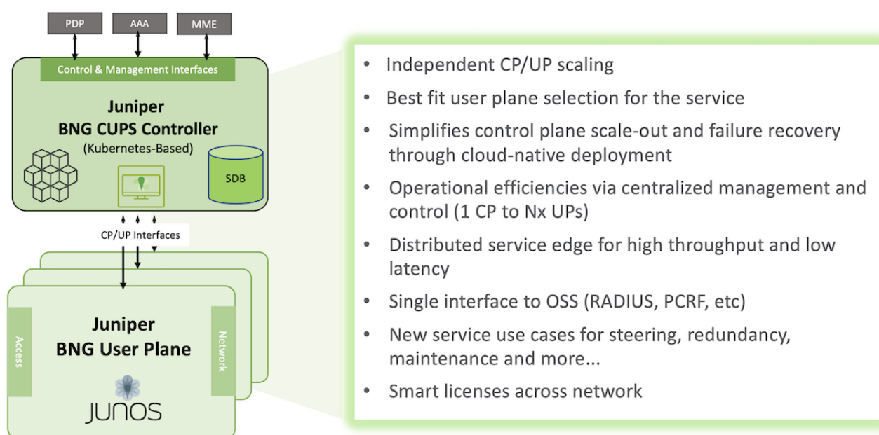
Figure 5: Juniper BNG CUPS Overview Architecture
