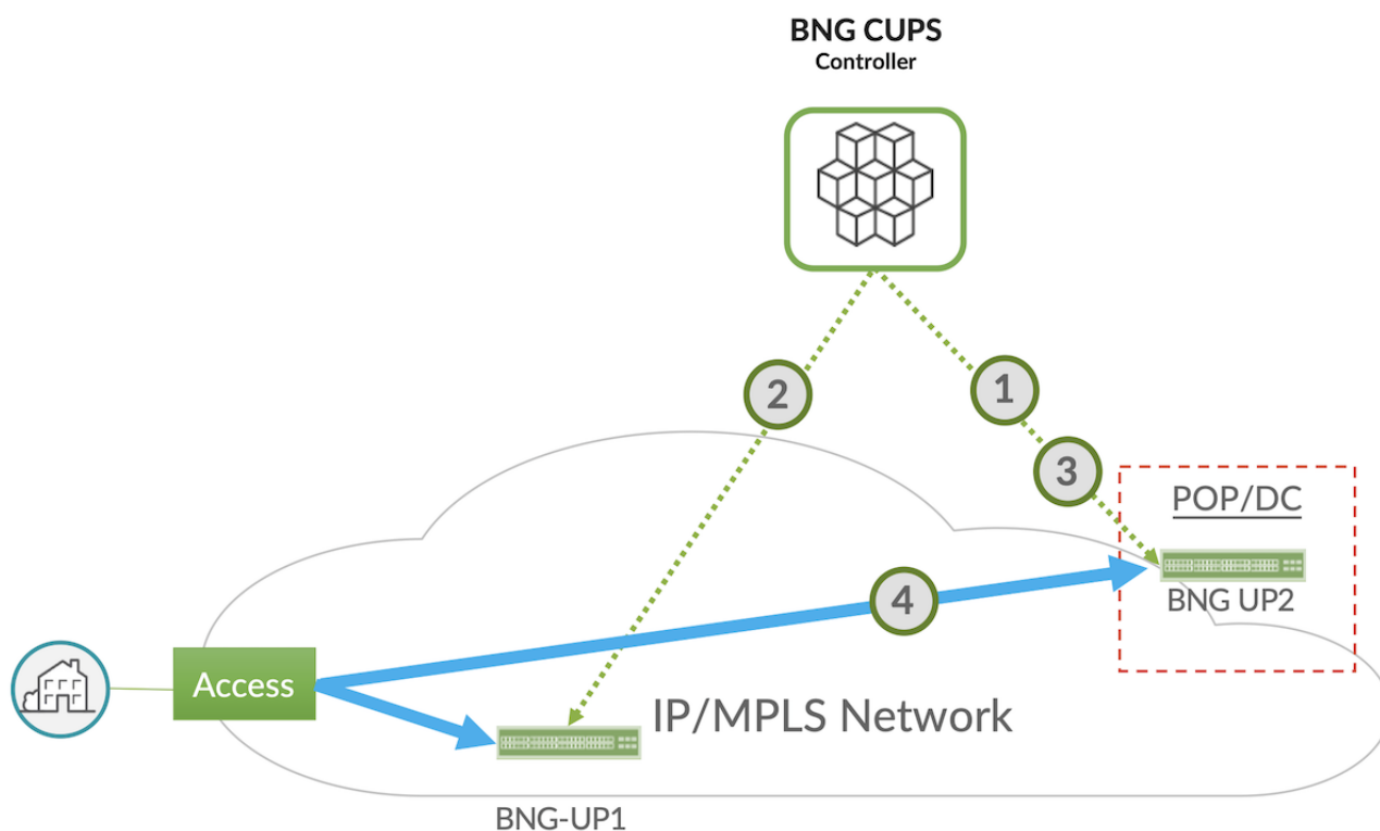
Figure 2: Juniper BNG CUPS hitless user plane maintenance in action
