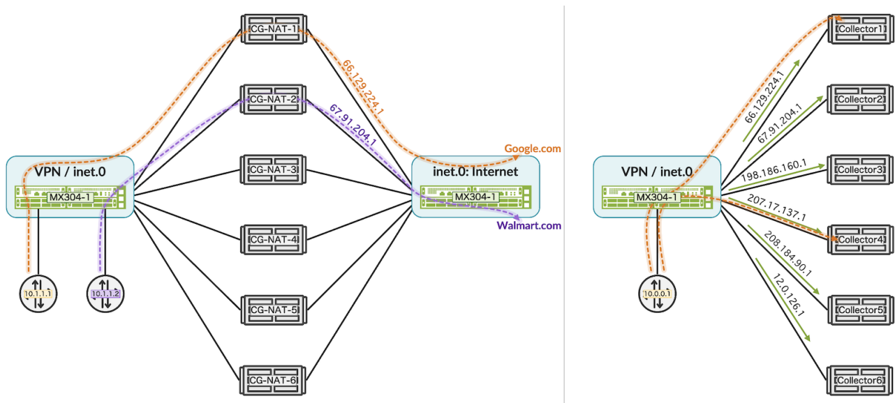
Figure 1: Illustration of symmetric load balancing
