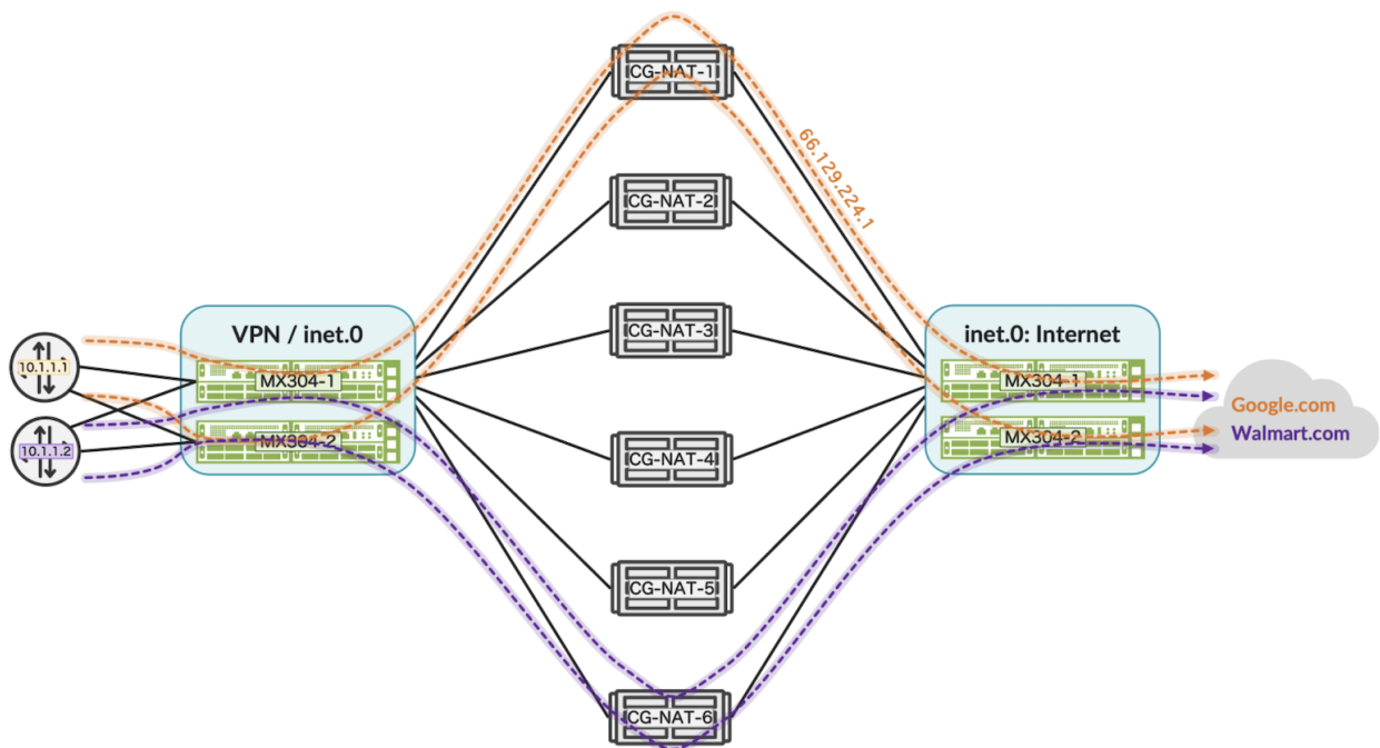
Figure 2: Illustration of consistent and symmetric load balancing
