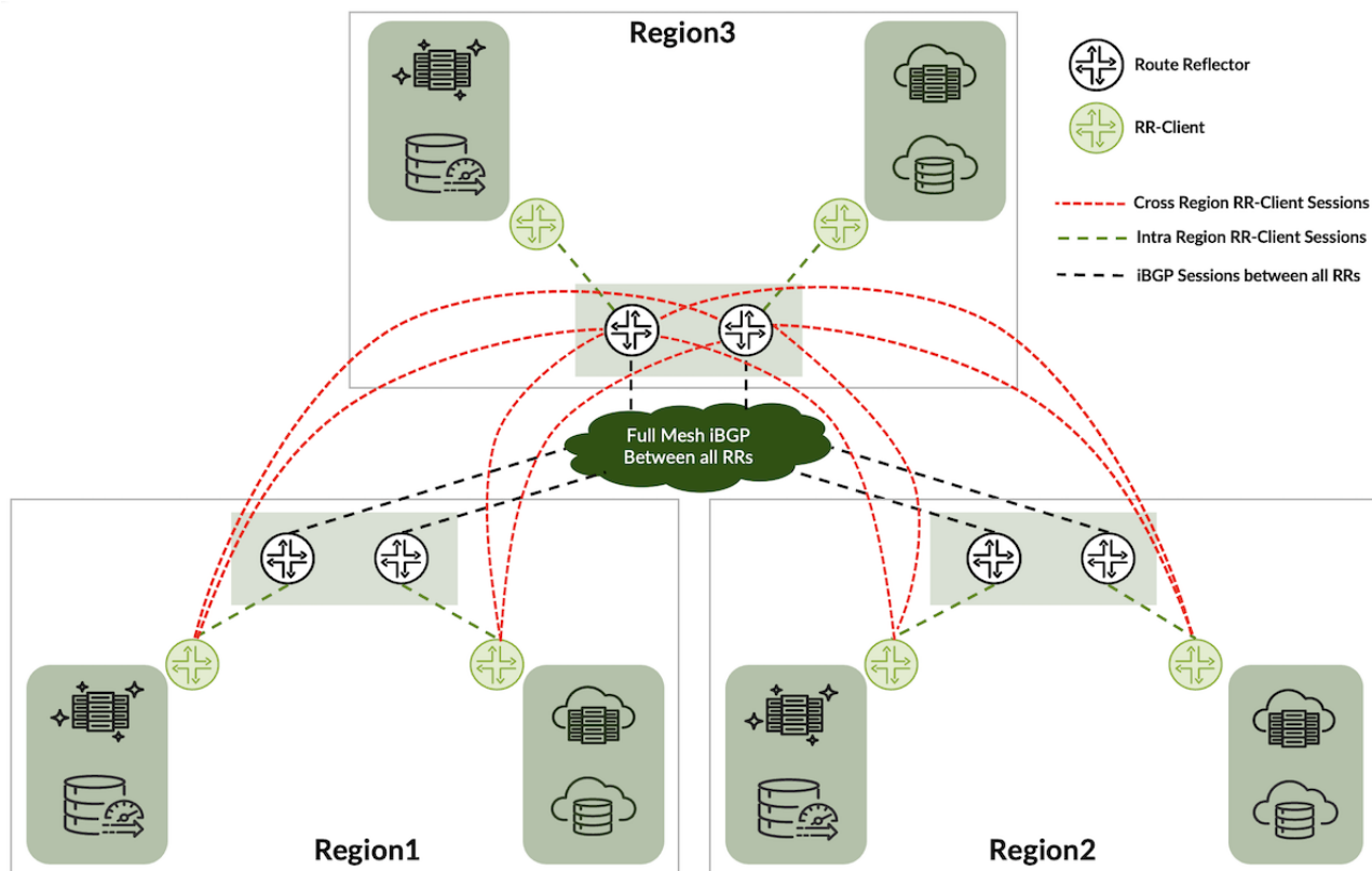
Figure 5: Route Reflector Strategic Design - (Logical Connectivity)
