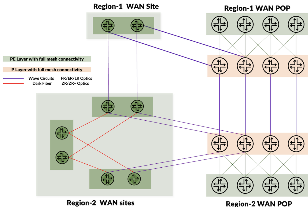
Figure 3: Diagram 3: WAN POP Regional and Cross-Regional Connectivity
