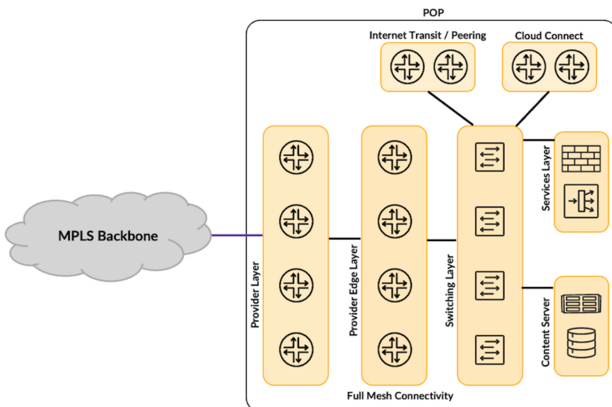
Figure 2: High-Level Architecture of WAN POP
