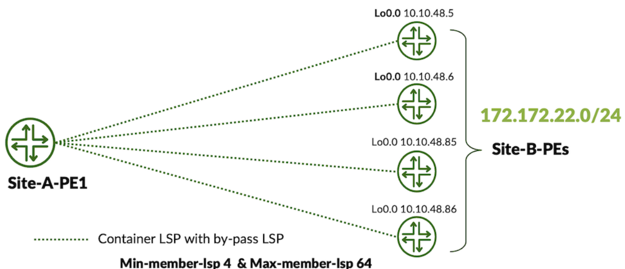
Figure 6: Base Topology to Depicts Next Hop Scaling
