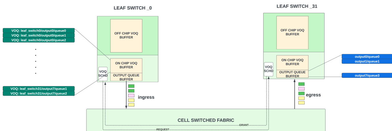
Figure 8: VOQ FABRIC
