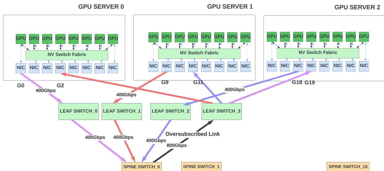
Figure 7: Example of switch getting oversubscribed
