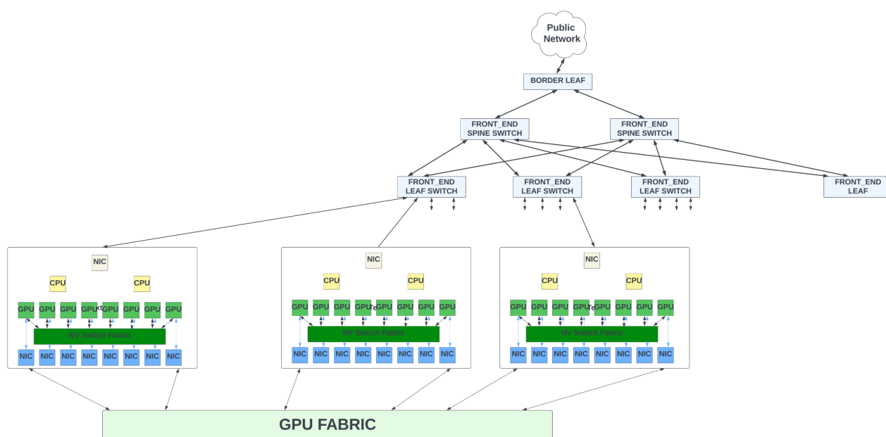
Figure 4: Conceptual diagram illustrating the GPU servers and the GPU fabric in a data center network.
