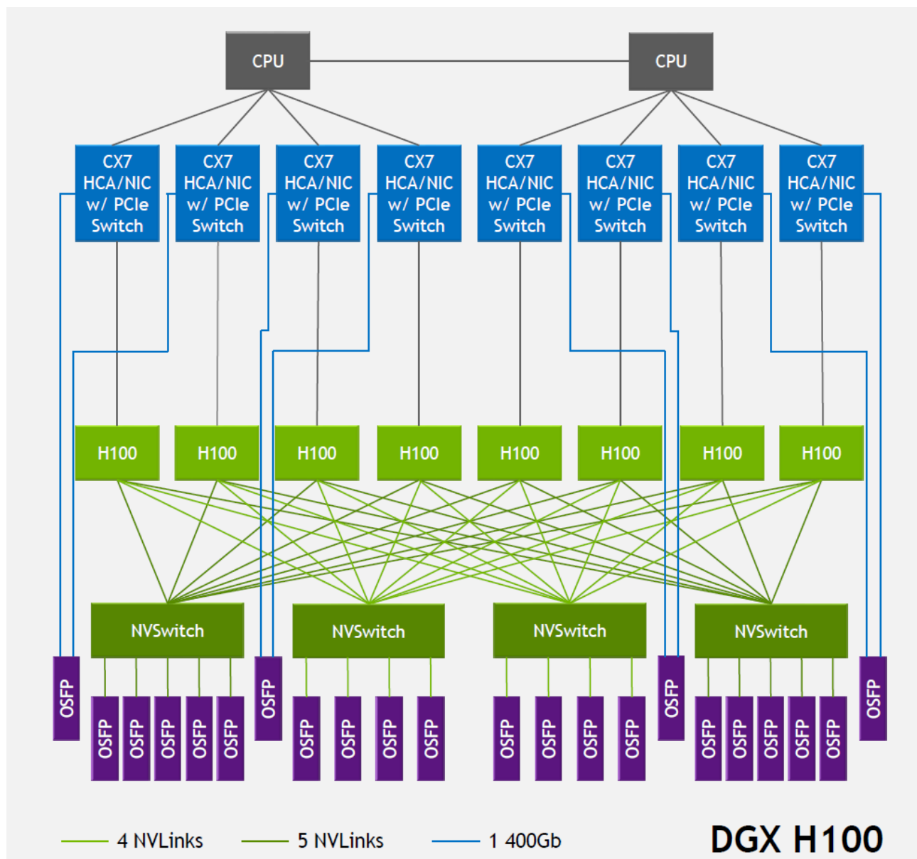
Figure 3: GPU server (node) with 8 GPUs.
