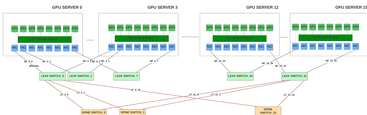
Figure 6: Conceptual diagram of a GPU fabric that connects 128 GPUs
