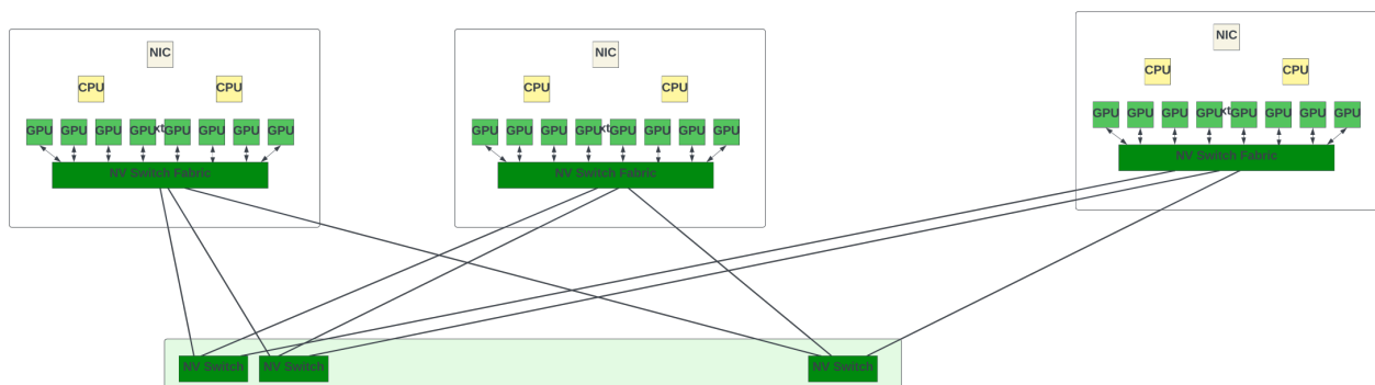
Figure 5: GPU Fabric with NV Switch System
