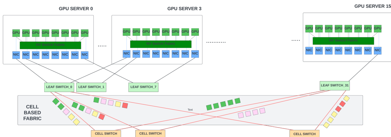
Figure 9: Cell-Based Fabric between Leaf Switches and cell switches
