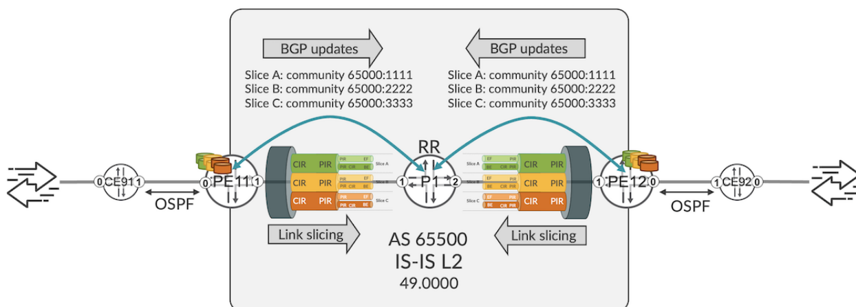
Figure 1: Link Slicing p2 Topology
