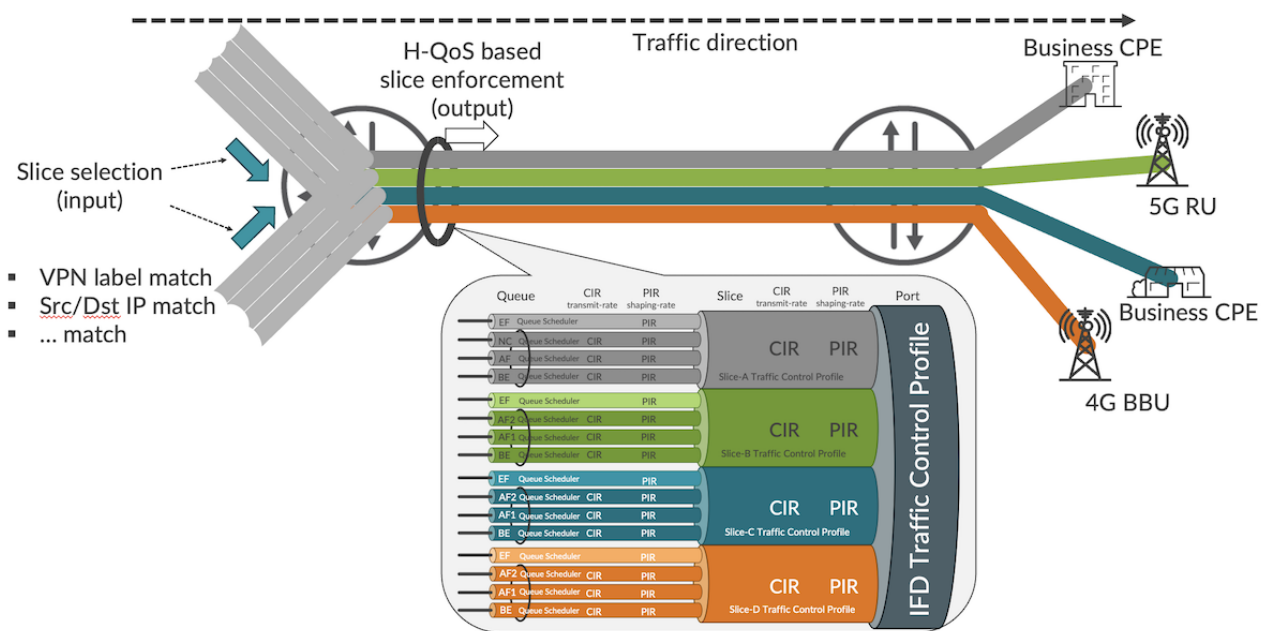
Figure 3: Link Slicing with slice-aware H-QoS
