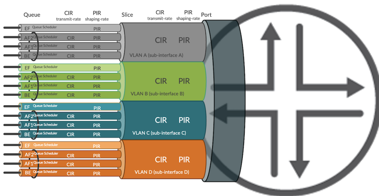
Figure 2: Link Slicing with legacy H-QoS
