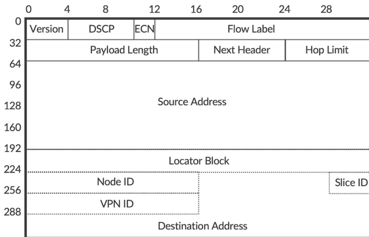
Figure 7: IPv6 header
