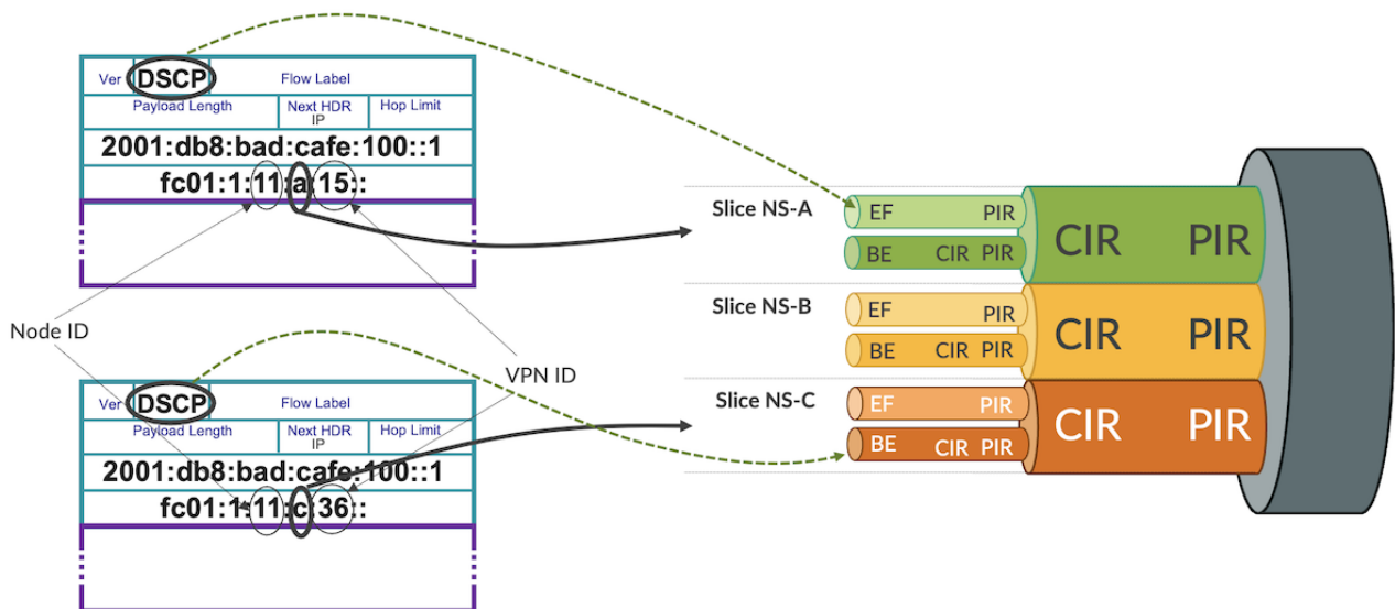
Figure 6: Traffic assignment to slices – SRv6
