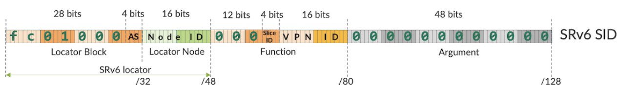
Figure 5: SRv6 SID Allocation Scheme
