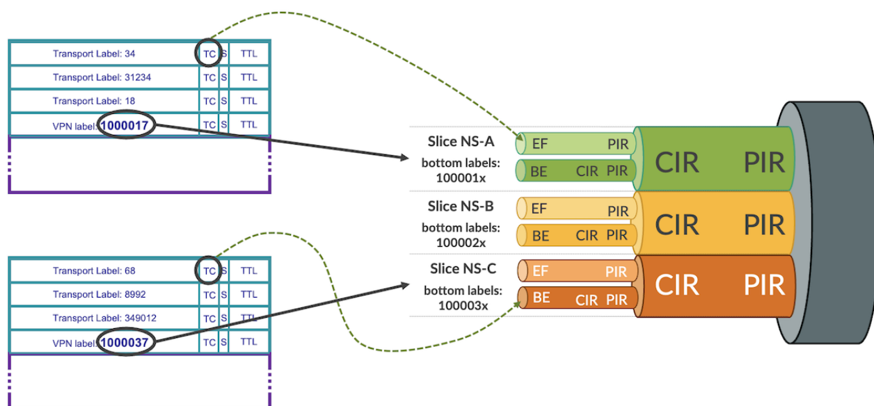
Figure 4: Traffic assignment to slices – MPLS
