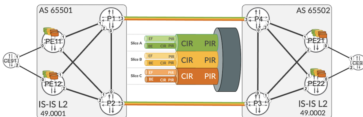
Figure 1: Inter-AS Topology with slicing on Inter-AS links
