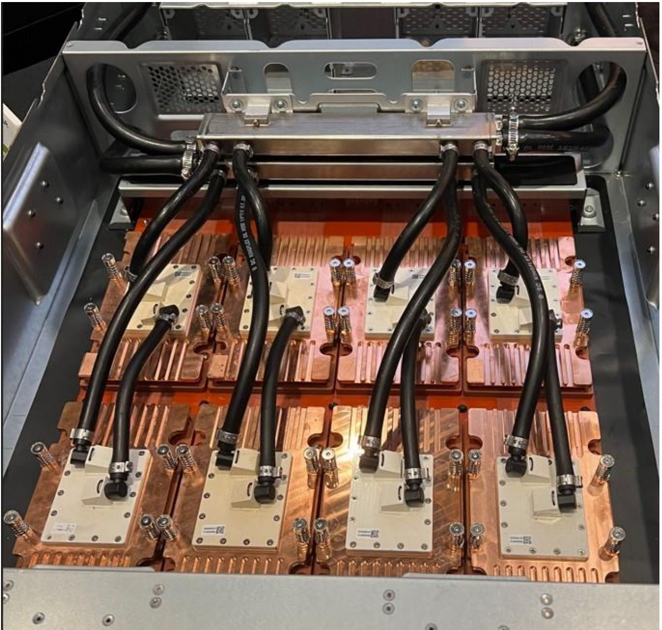
Figure 1: Cold plate with liquid loops cooling eight 1KW Accelerator chips
