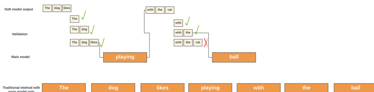
Figure 5: An illustration of how speculative decoding can speed up inference.
