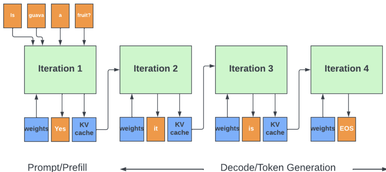
Figure 2: An illustration of LLM inference for generating the output sequence
