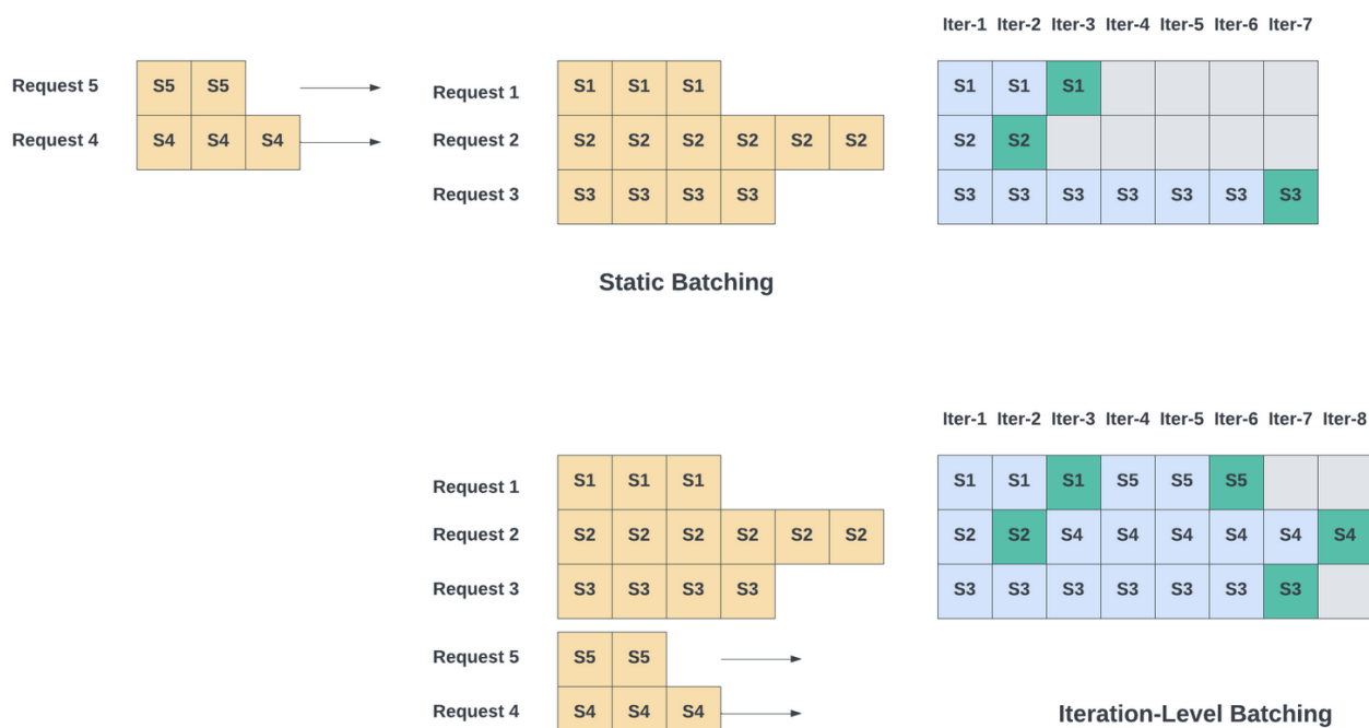
Figure 10: Simplified Illustration of static versus Iteration-level batching
