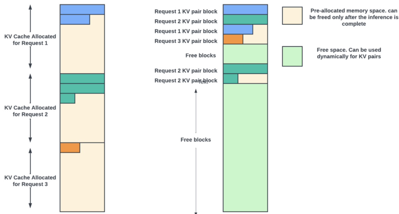
Figure 6: Simple illustration for dynamic allocation of memory blocks for KV cache.
