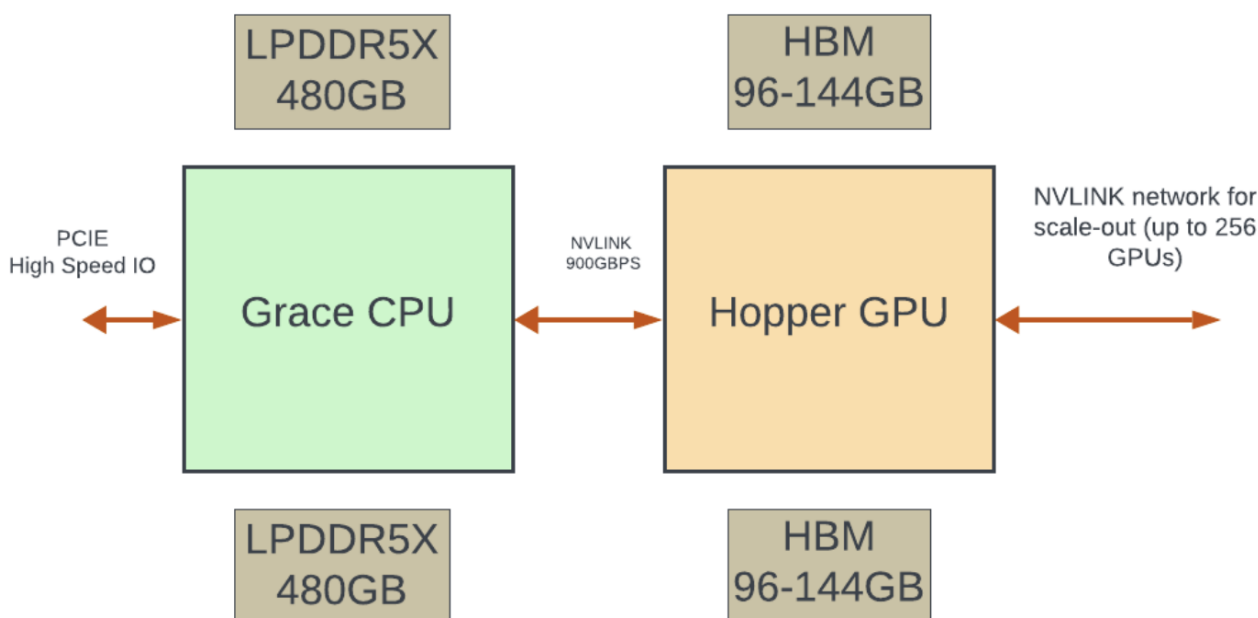
Figure 11: Illustration of GPU/CPU interconnected in GH200
