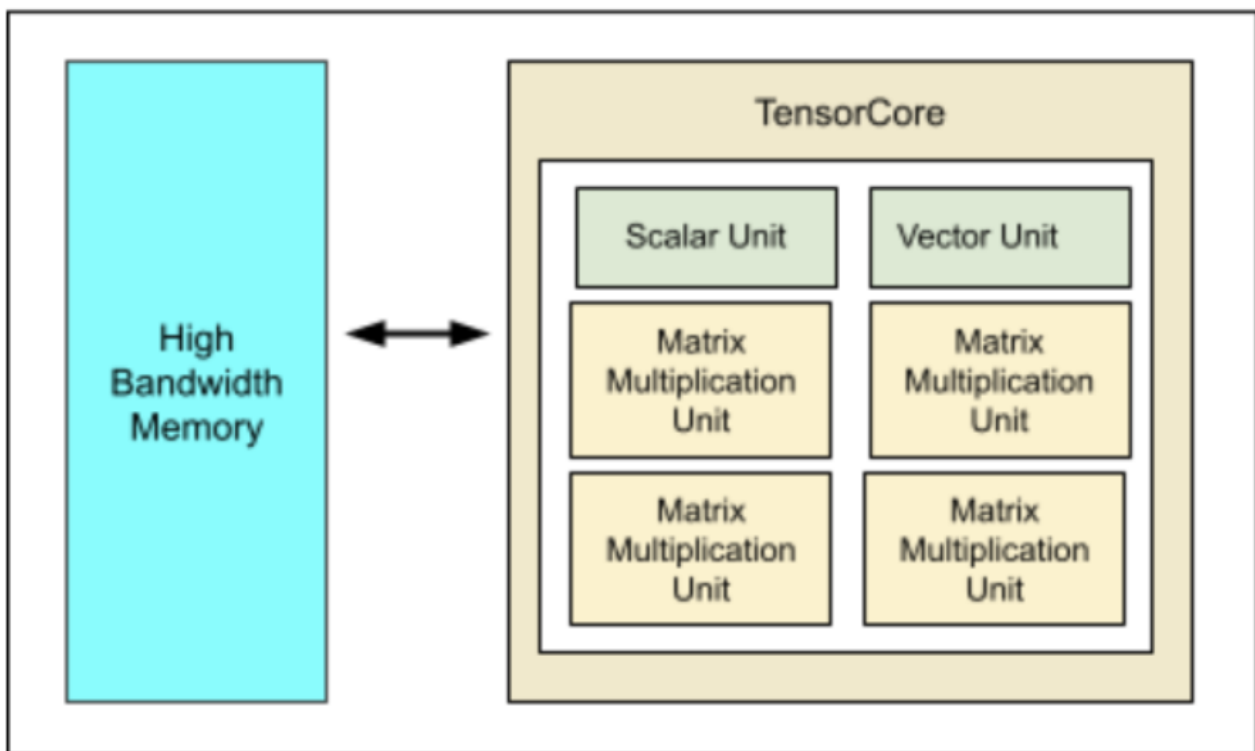
Figure 12: Google's TPUv5e is optimized for inference workloads.
