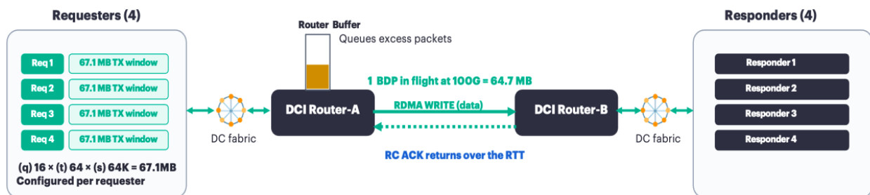
Figure 5: Buffer Sizing Considerations
