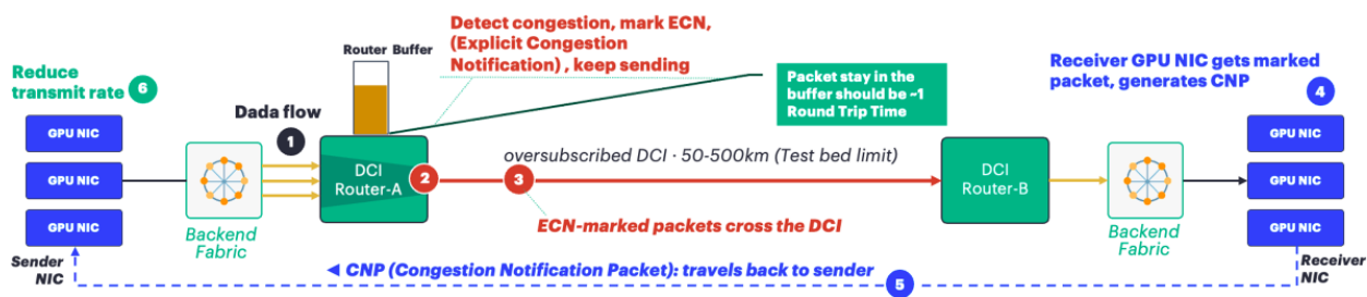
Figure 2: Anatomy of Lossless RDMA
