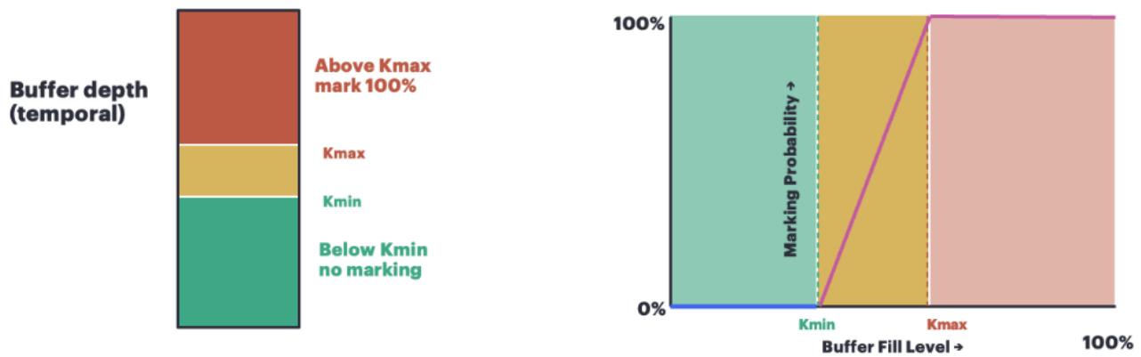
Figure 4: Buffer Depth and ECN Thresholds
