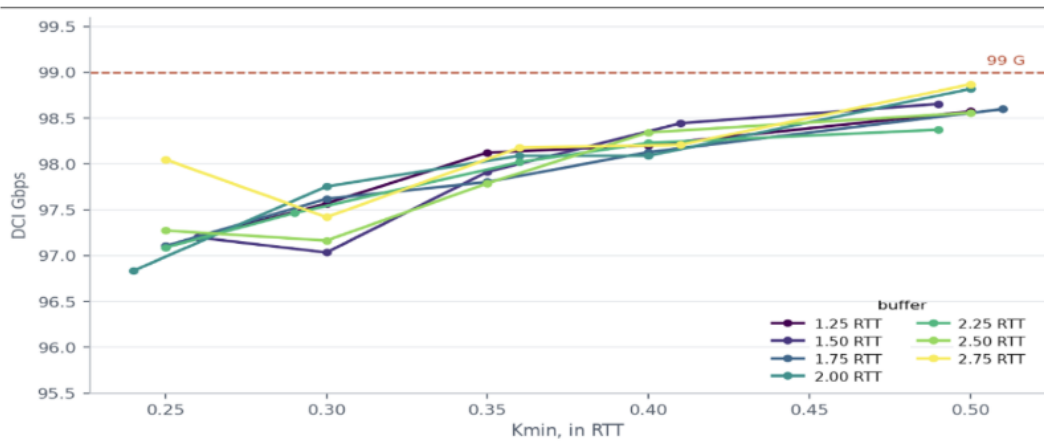
Figure 7: Buffer and Kmin Sweep at 200 km
