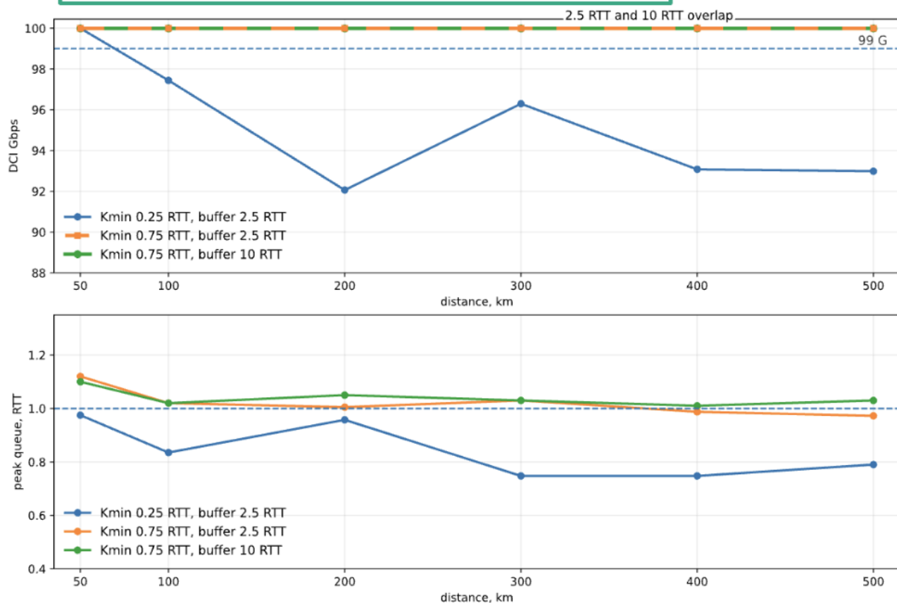
Figure 8: Soak Testing - 16 Queue Pairs
