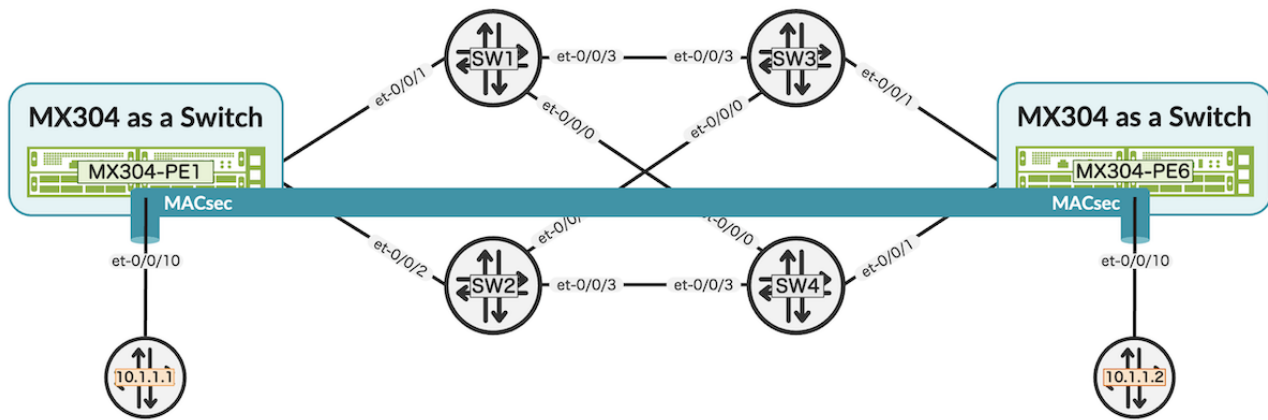
Figure 3: The MX provides MACsec and sends it transparently over the Layer 2 network.
