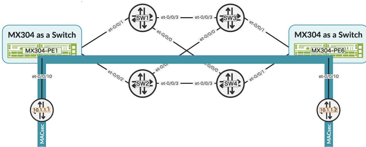
Figure 4: The MX carries MACsec transparently over the Layer 2 network.
