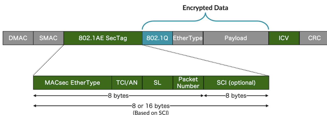
Figure 1: MACsec Frame and Header Structure.
