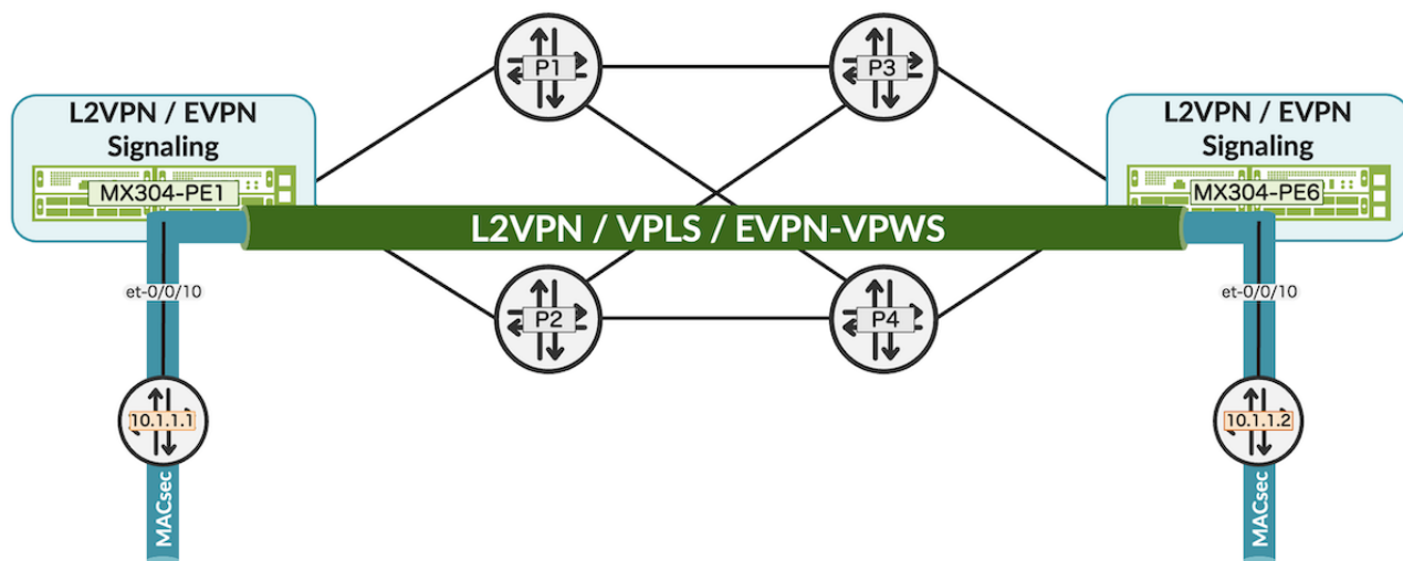
Figure 6: The MX carries MACsec transparently over the MPLS network.
