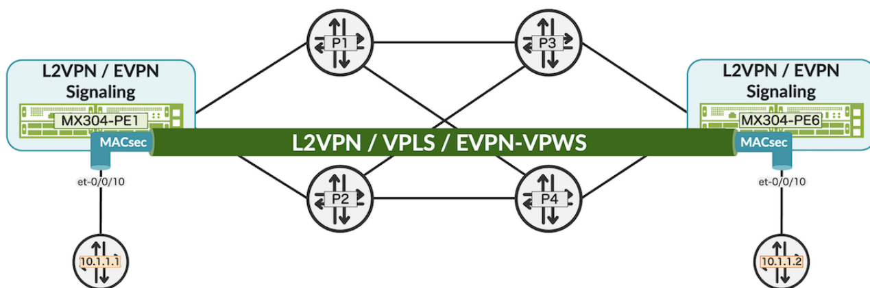
Figure 5: The MX provides MACsec and sends it transparently over the MPLS network.
