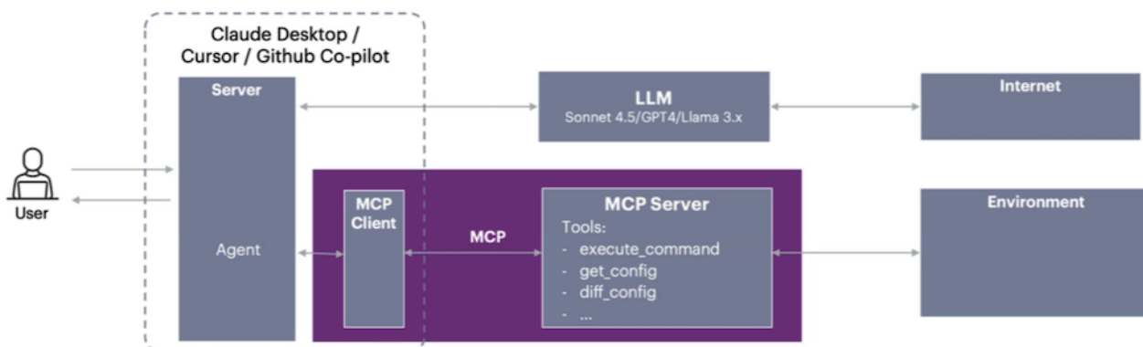
Figure 1: Basic LLM/MCP Infrastructure
