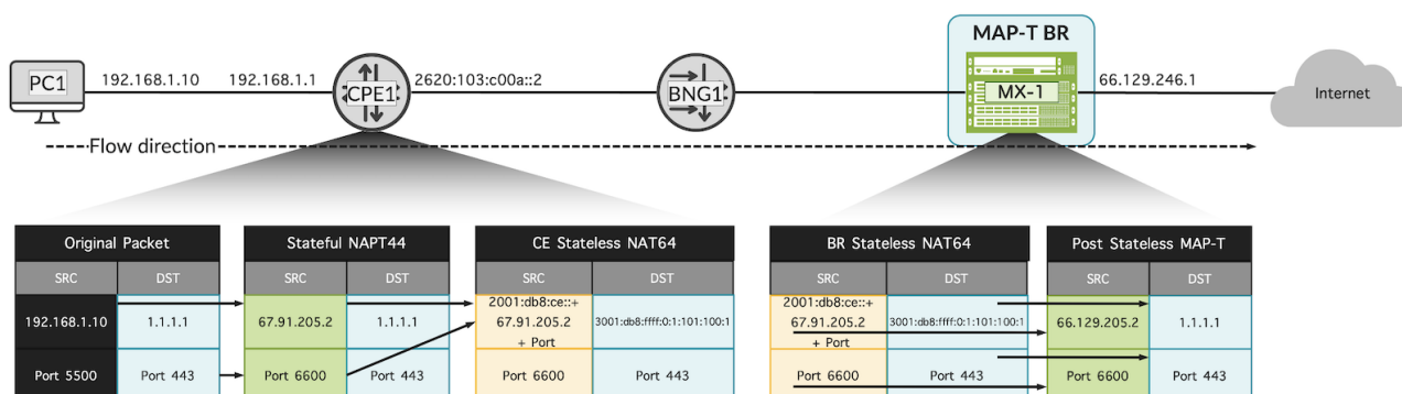
Figure 2: Packet flow and translation
