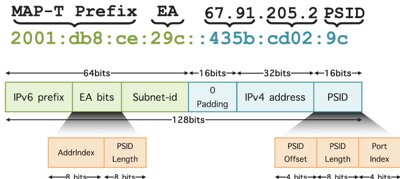
Figure 3: Embedded Address (EA) Bits
