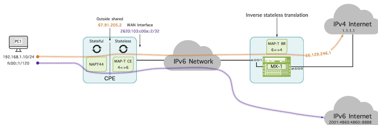
Figure 1: High level topology
