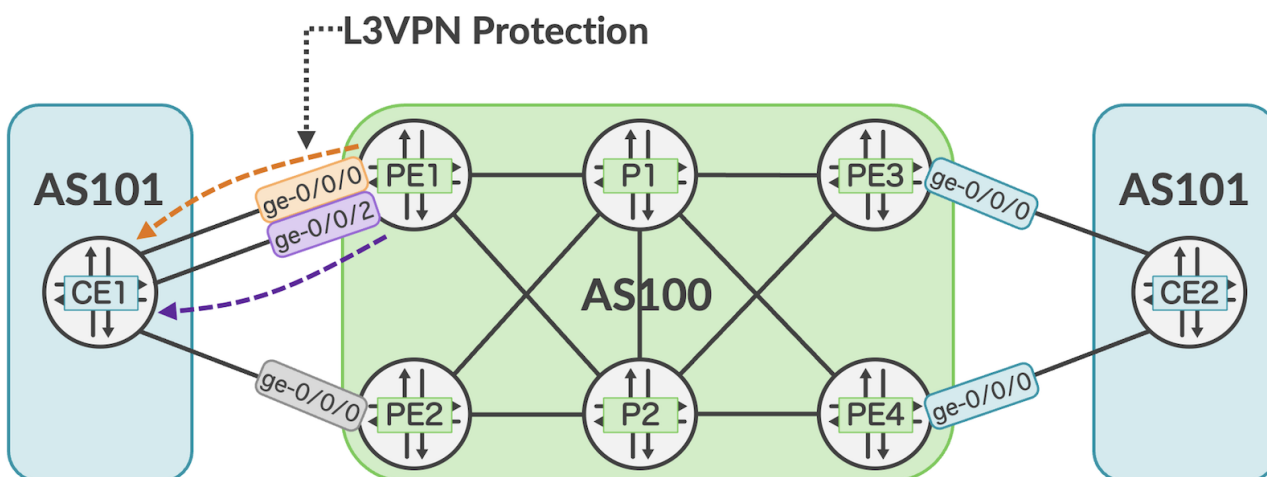
Figure 8: Protection within a VRF for two directly connected eBGP sessions to the same CE
