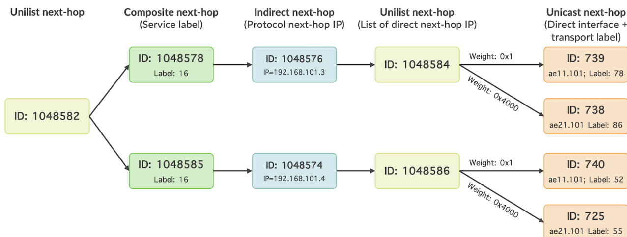
Figure 5: Hierarchical Routing Structure with service layer PIC feature
