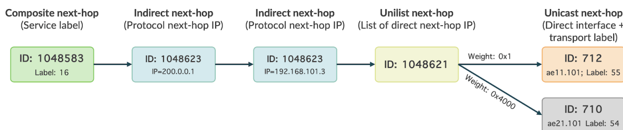
Figure 9: Hierarchical Routing Structure on PE1 for a destination with two INH
