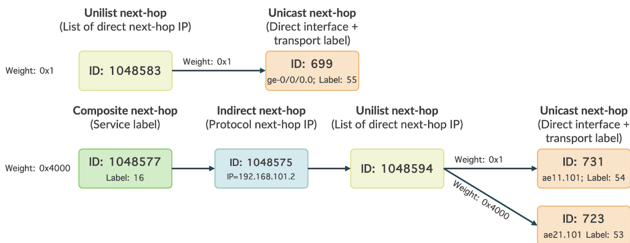
Figure 7: Hierarchical Routing Structure with protection feature.
