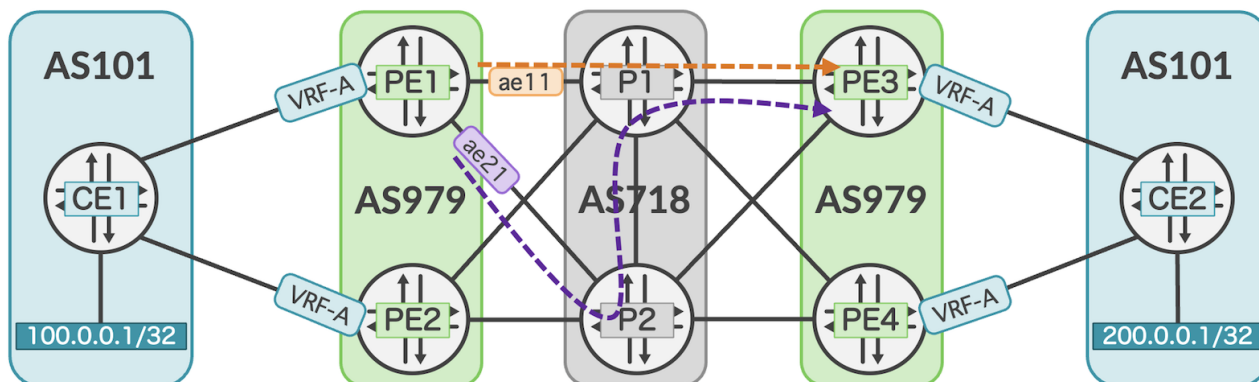
Figure 2: Fast reroute using backup path towards PE3
