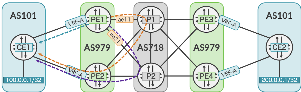
Figure 6: Fast reroute via two backup paths towards CE1
