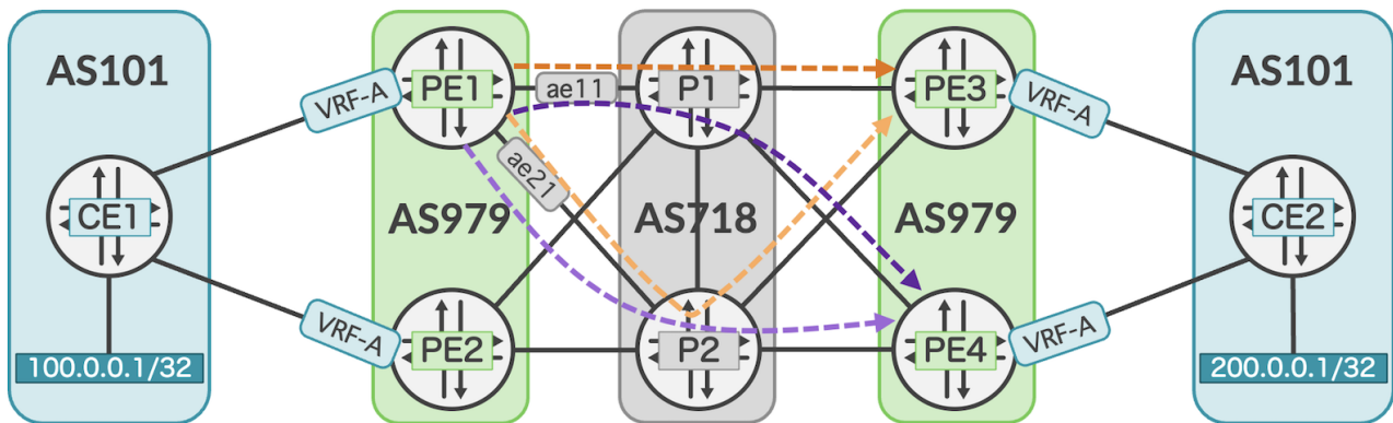
Figure 4: Fast Reroute with multiple backup paths to CE2, announced by PE3 and PE4
