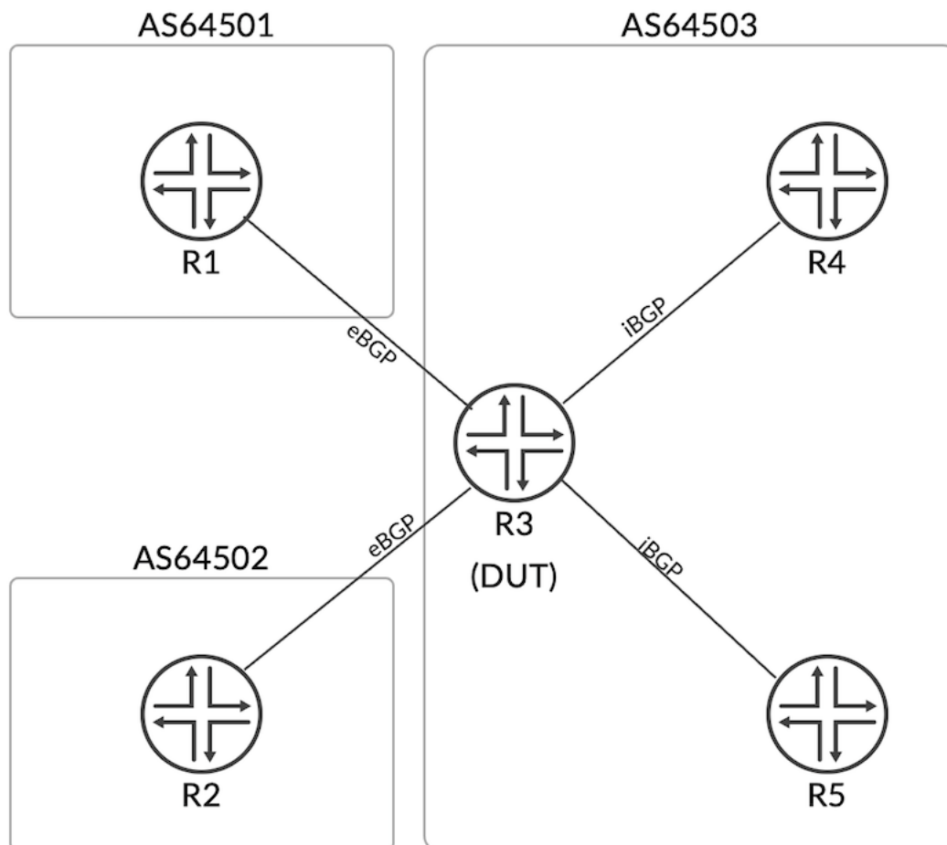
Figure 1: Topology
