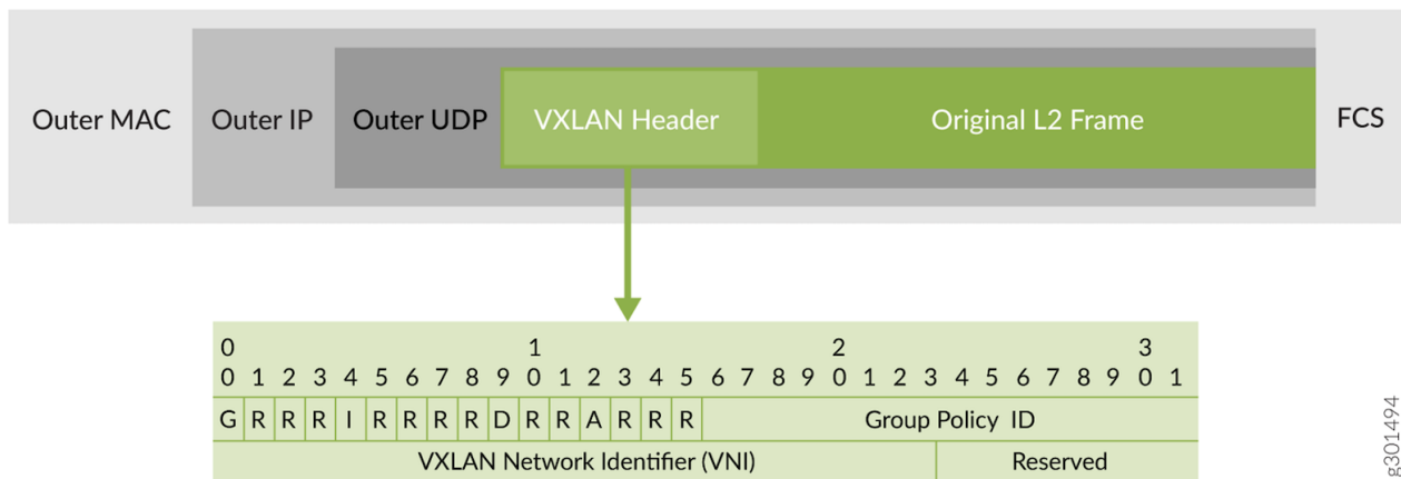
Figure 2: VXLAN-GBP uses reserved fields in the VXLAN header for Scalable Group Tags (SGTs).
