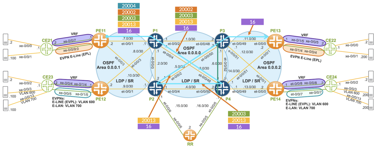
Figure 4: Static SR LSP Path Labels w/color
