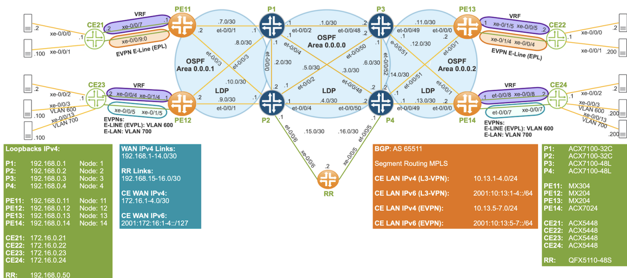
Figure 1: Multi OSPF Area and LDP
