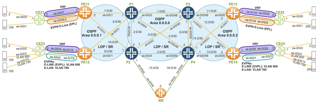
Figure 2: Multi OSPF Area, LDP and Segment Routing
