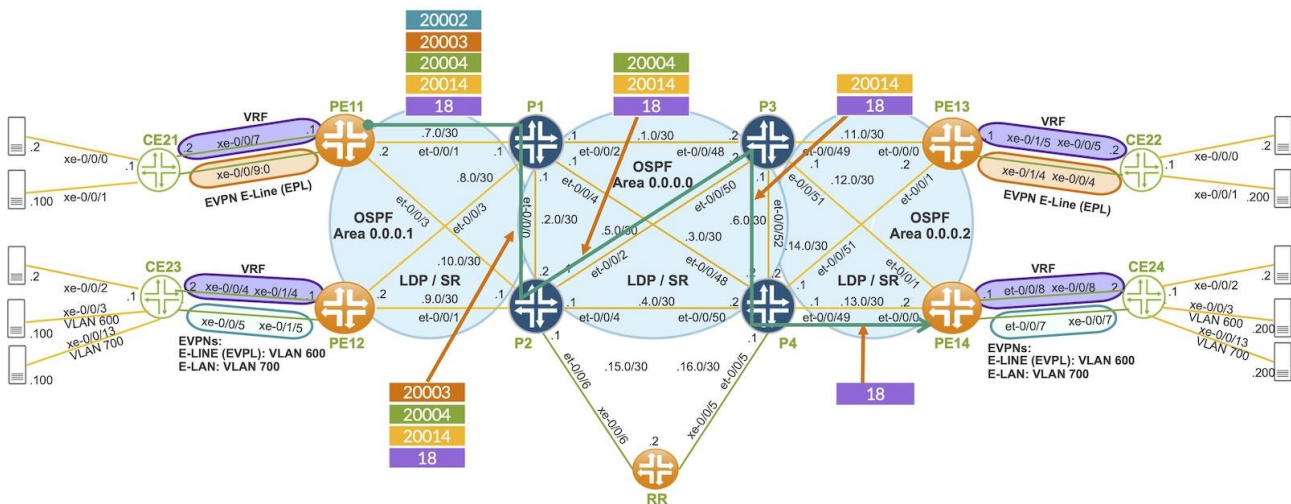
Figure 3: Static SR LSP Path Labels
