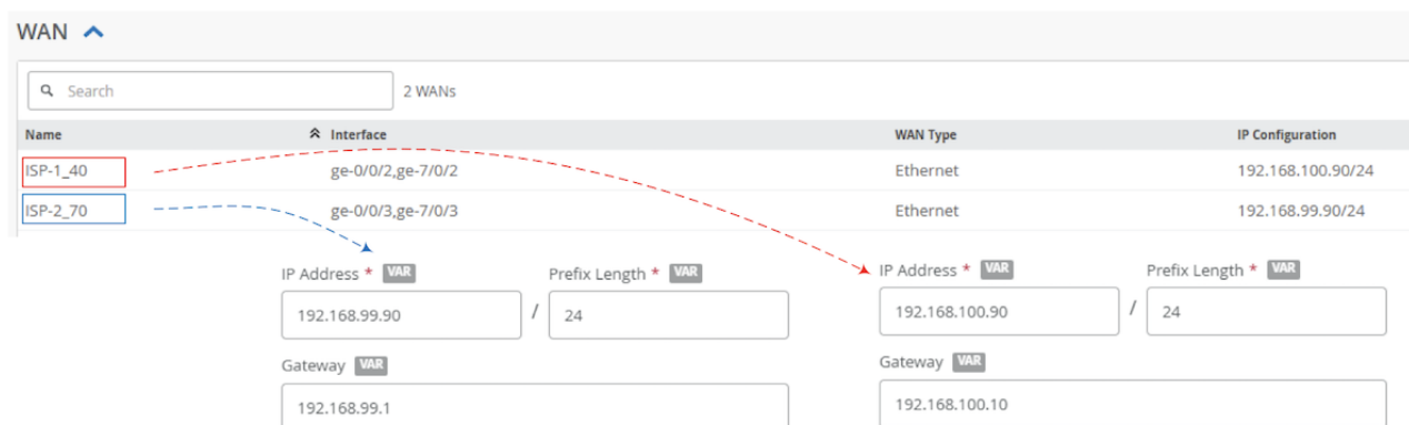
Figure 21: WAN Interfaces and Gateway Configurations
