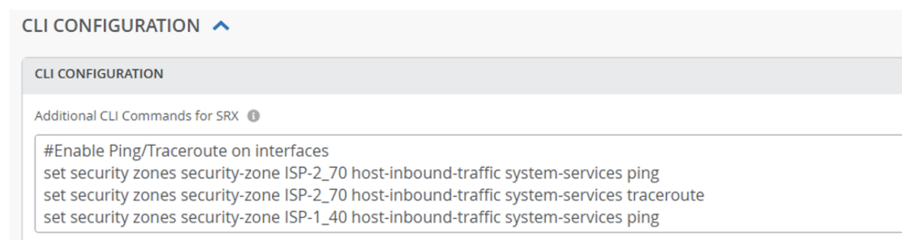
Figure 15: CLI Configuration Window
