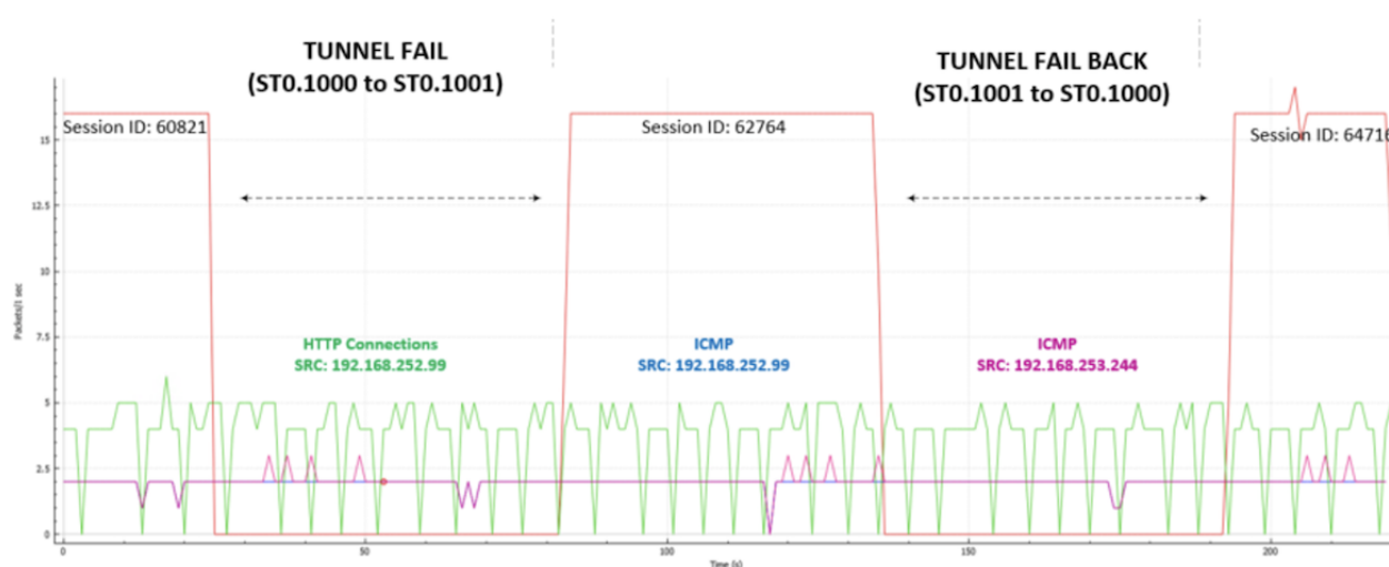
Figure 14: Traffic on Failover and Failback
