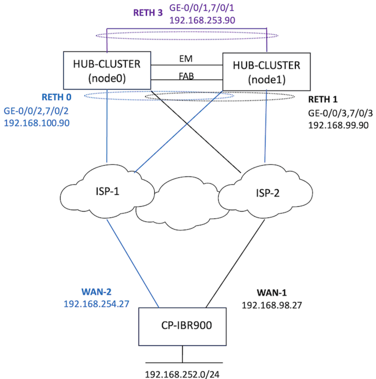
Figure 7: Figure 7. High Level Topology
