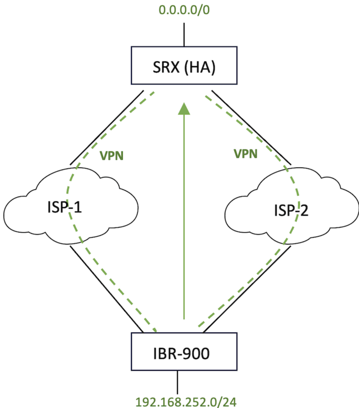
Figure 9: No Split Tunneling
