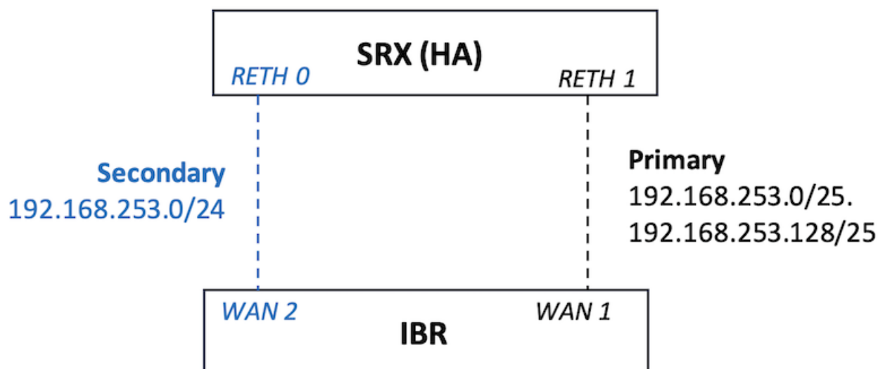
Figure 10: Primary Secondary Tunnel Selection via specific routes
