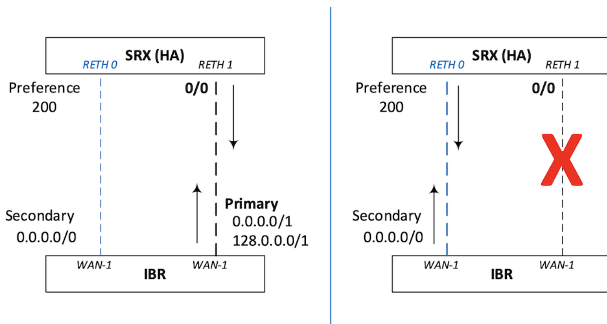
Figure 22: Primary and Secondary Tunnel Selection
