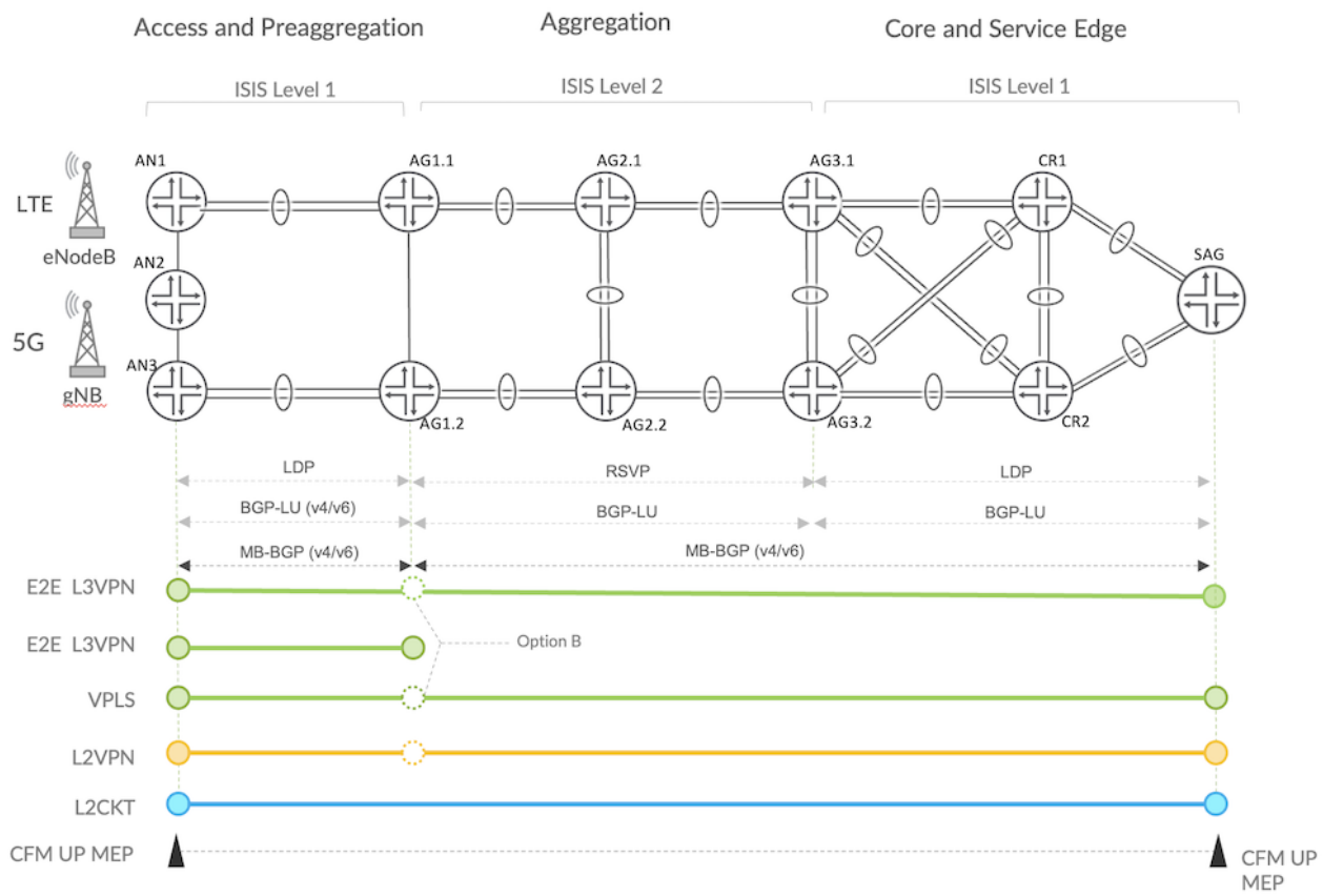
Figure 2: Featured Overlay Services
