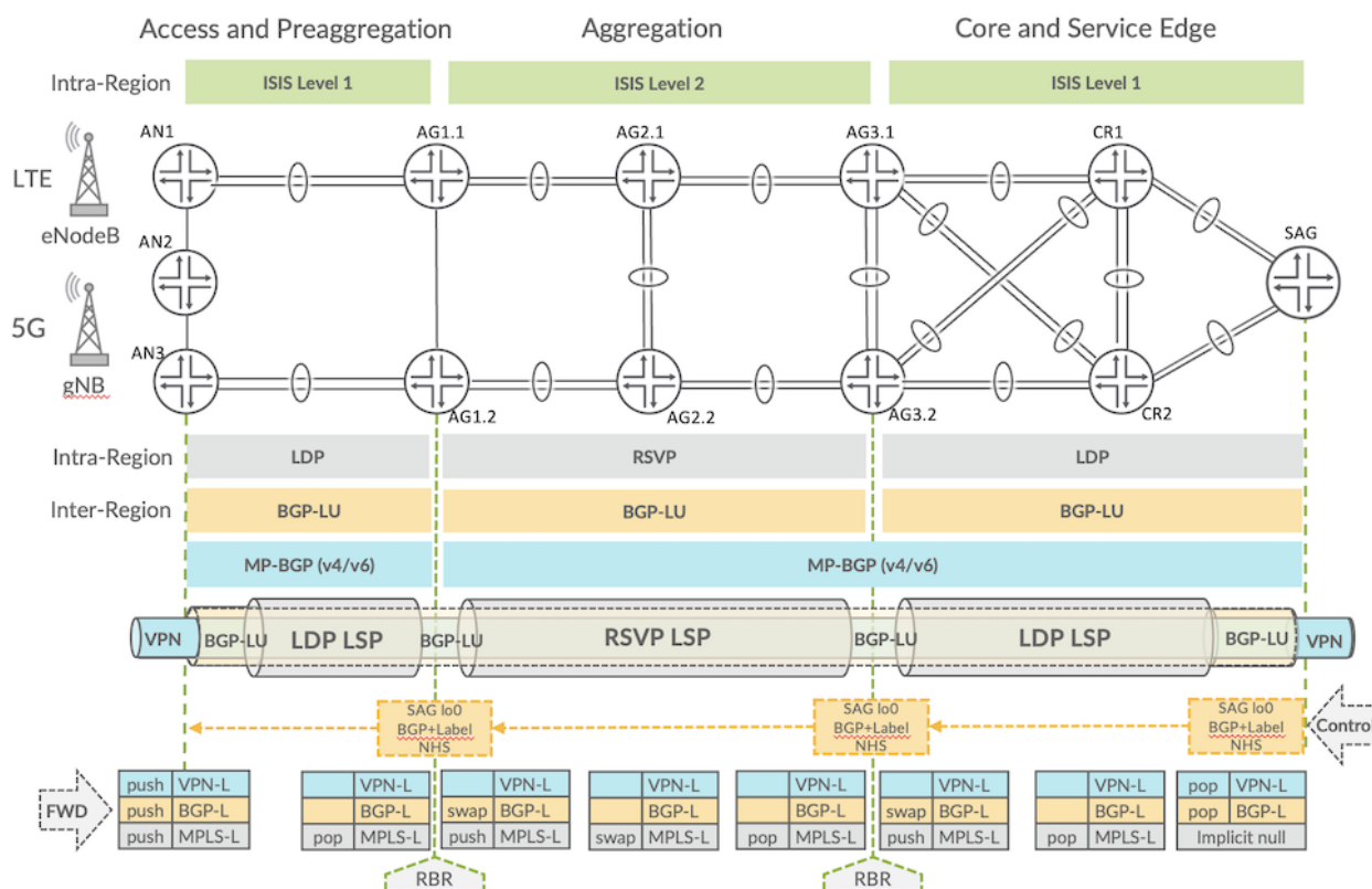
Figure 1: Multi-Region Seamless MPLS with BGP-LU
