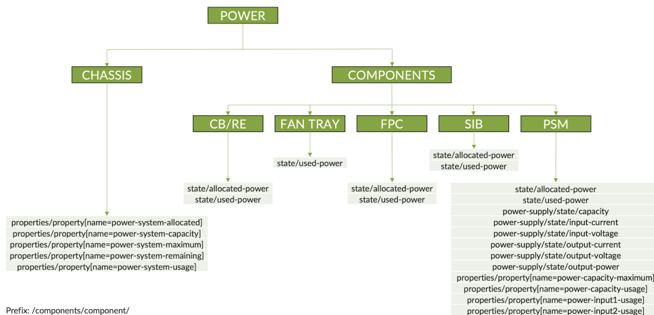
Figure 3: Power counters from /components OC path
