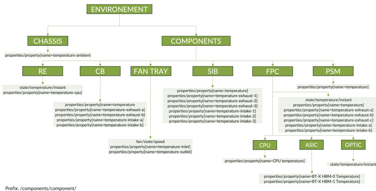
Figure 4: Temperature & Fan state counters from /components OC path
