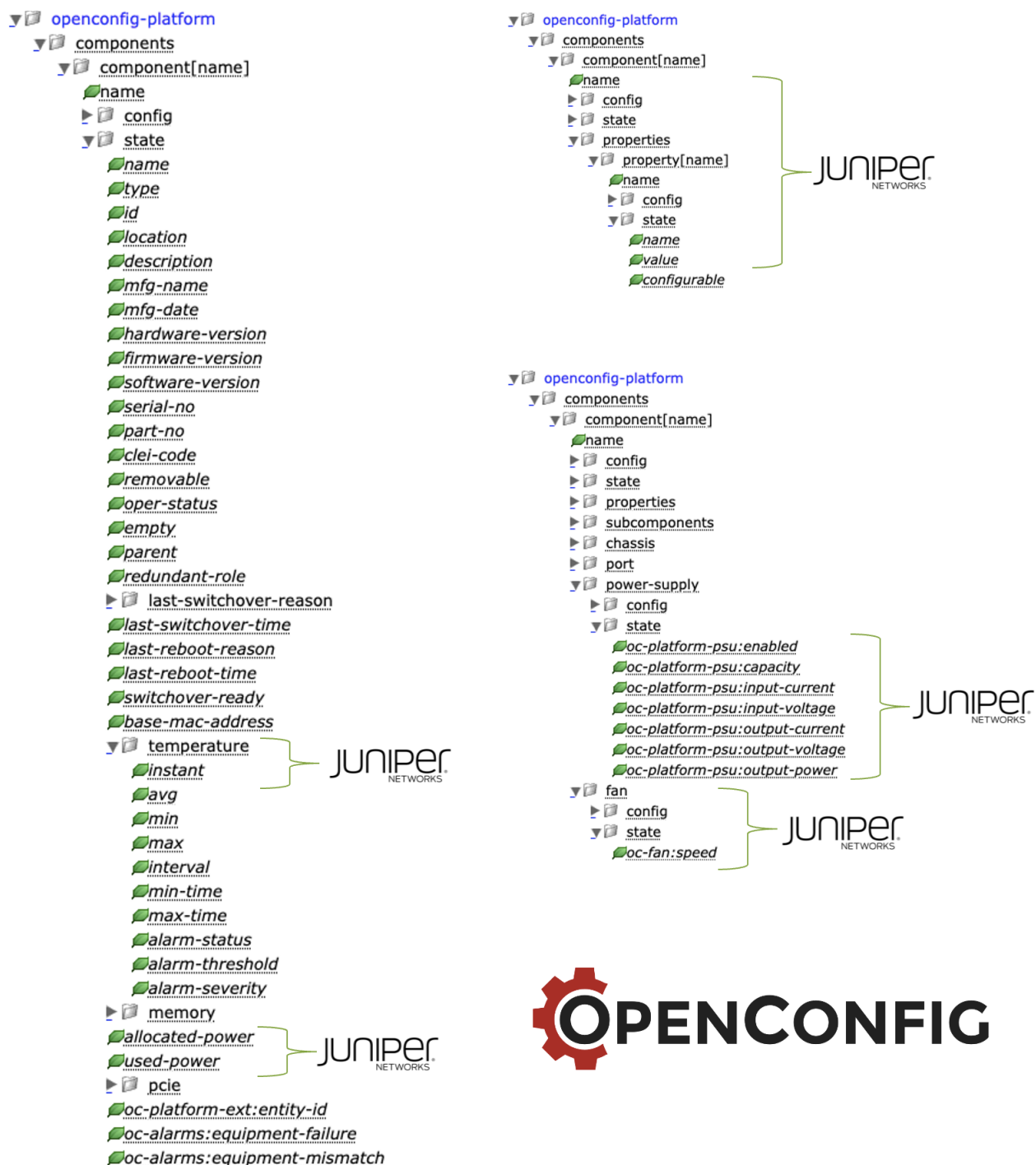
Figure 2: The /components path
