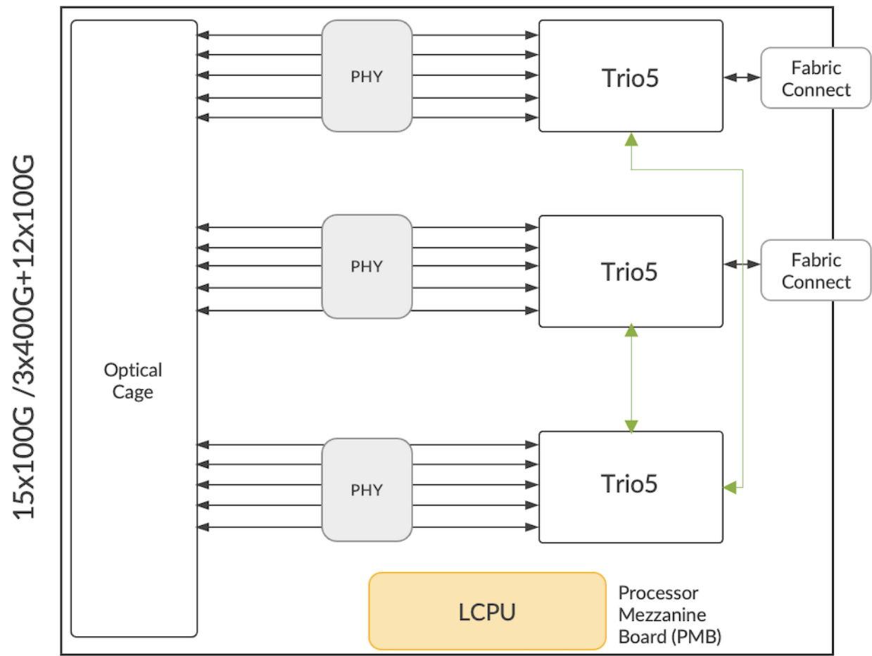
Figure 5: MPC10E-15C Architecture
