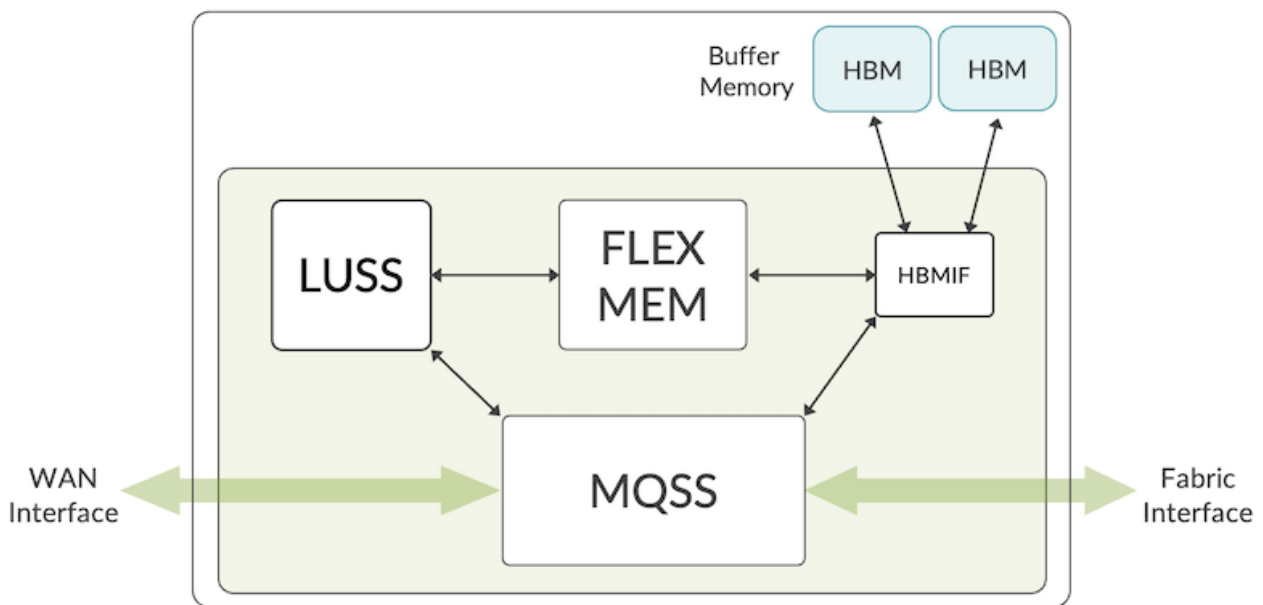
Figure 3: Trio5 Architecture
