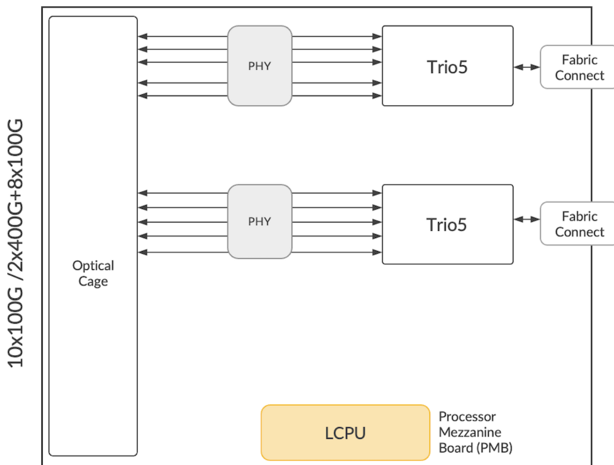
Figure 6: MPC10E-10C Architecture
