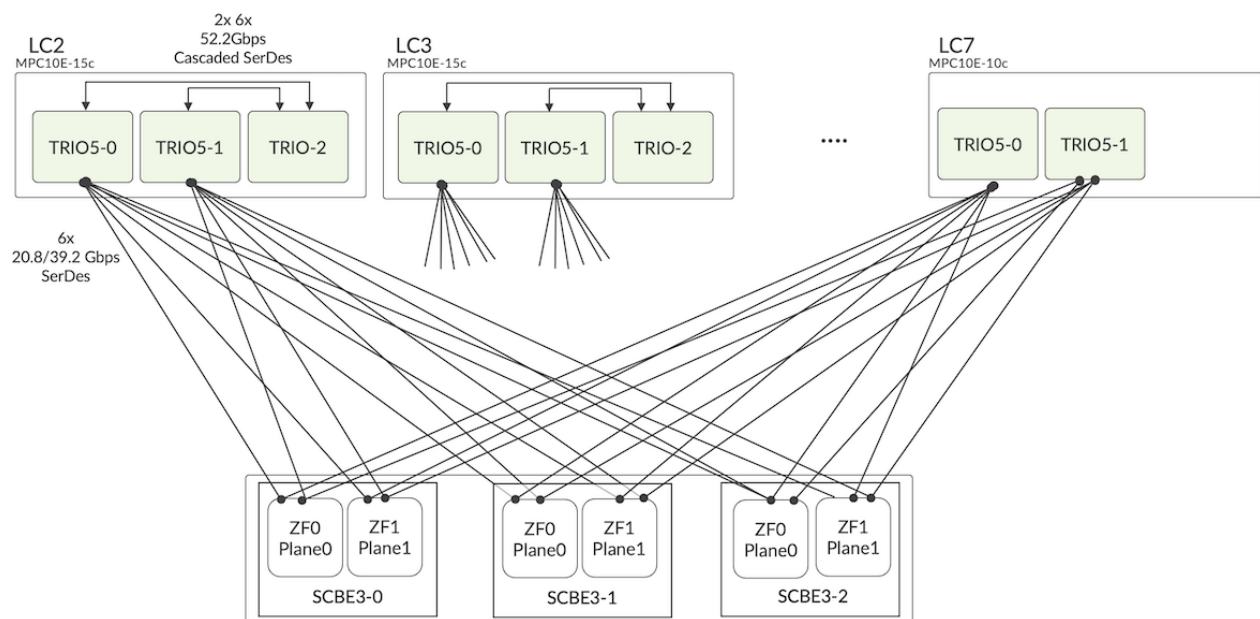
Figure 7: MPC10E and SCBE3 (MX960) Interconnect
