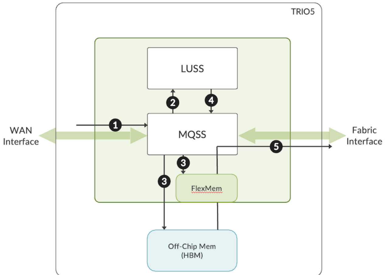
Figure 4: Trio5 Life of a Packet
