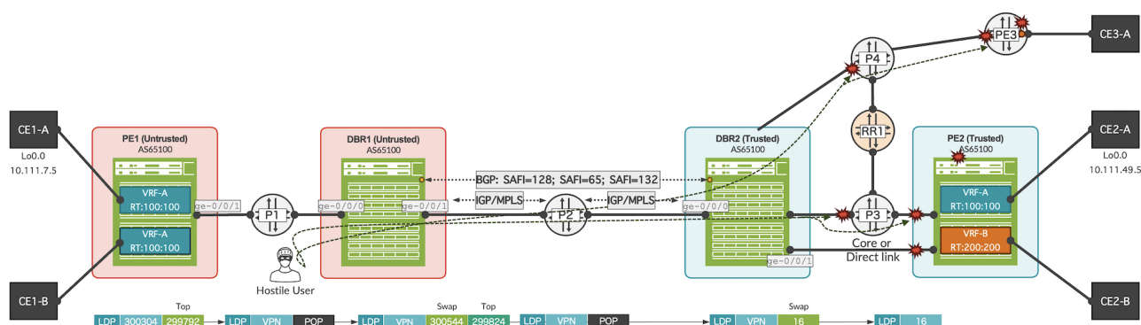
Figure 1: End to End topology, attack scenario
