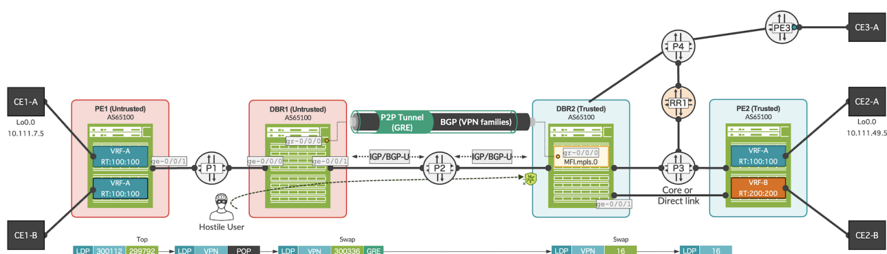
Figure 2: End to End Topology with Anti-Spoofing Feature Activated
