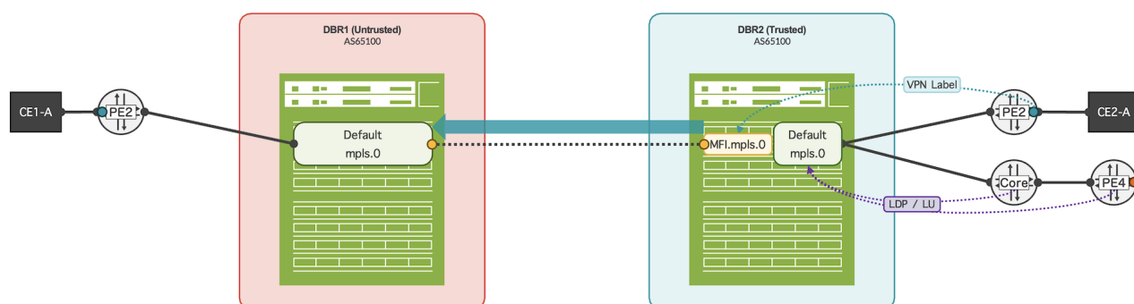
Figure 4: Label advertisement with RTC enabled
