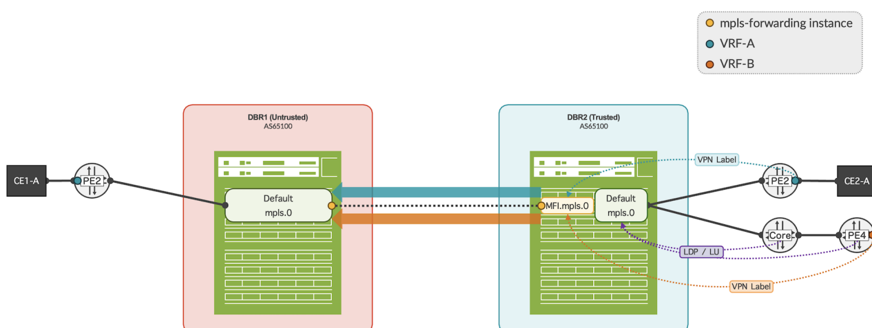
Figure 3: Label advertisement with MPLS anti-spoofing enabled for BGP option 10b
