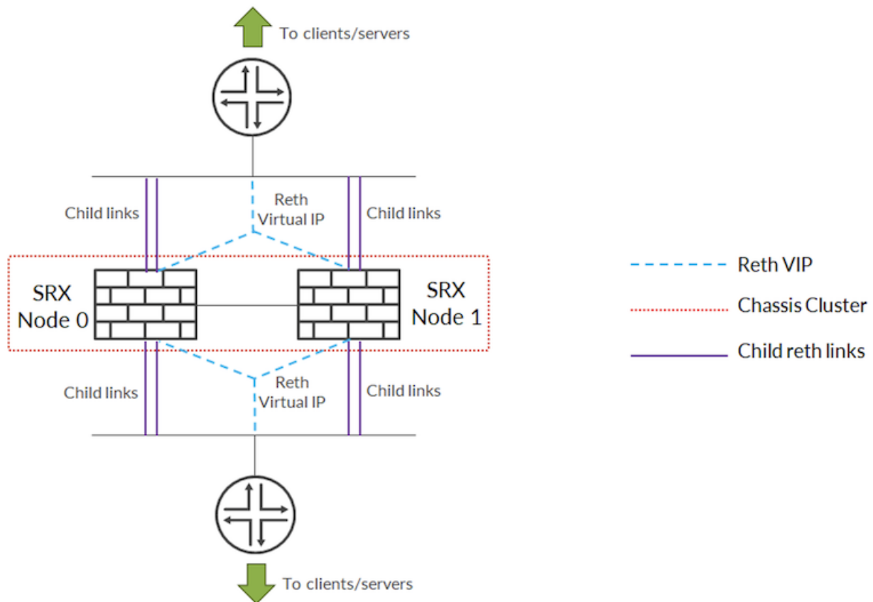
Figure 1: Chassis Clustering Topology
