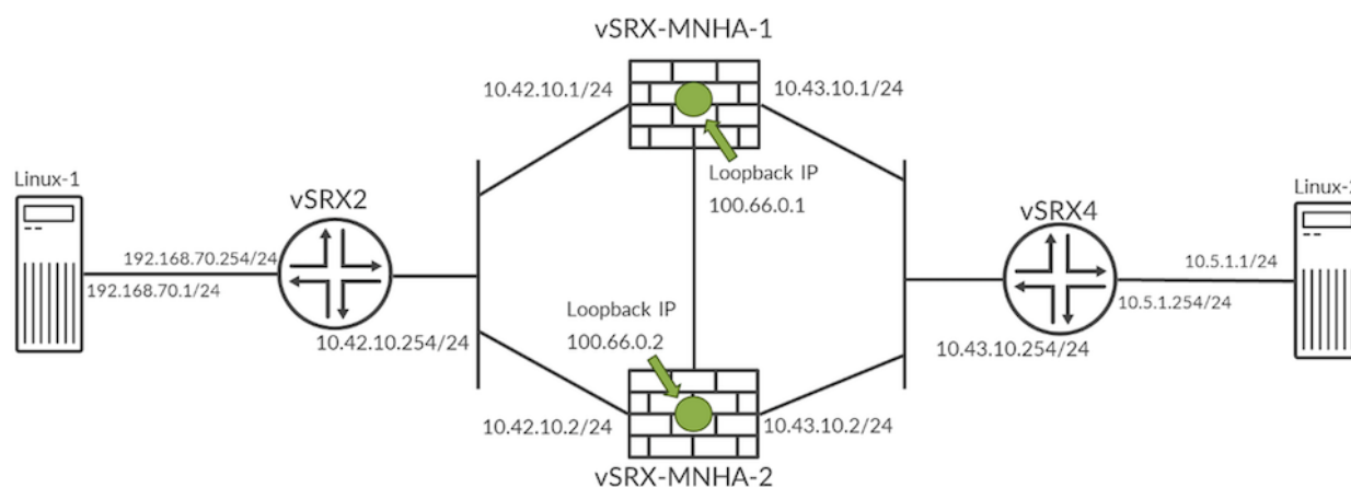
Figure 4: Simple lab MNHA setup
