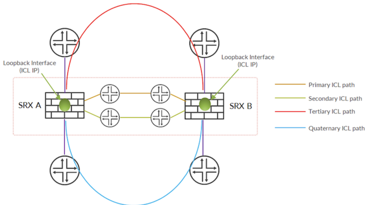
Figure 3: Inter-Chassis topology
