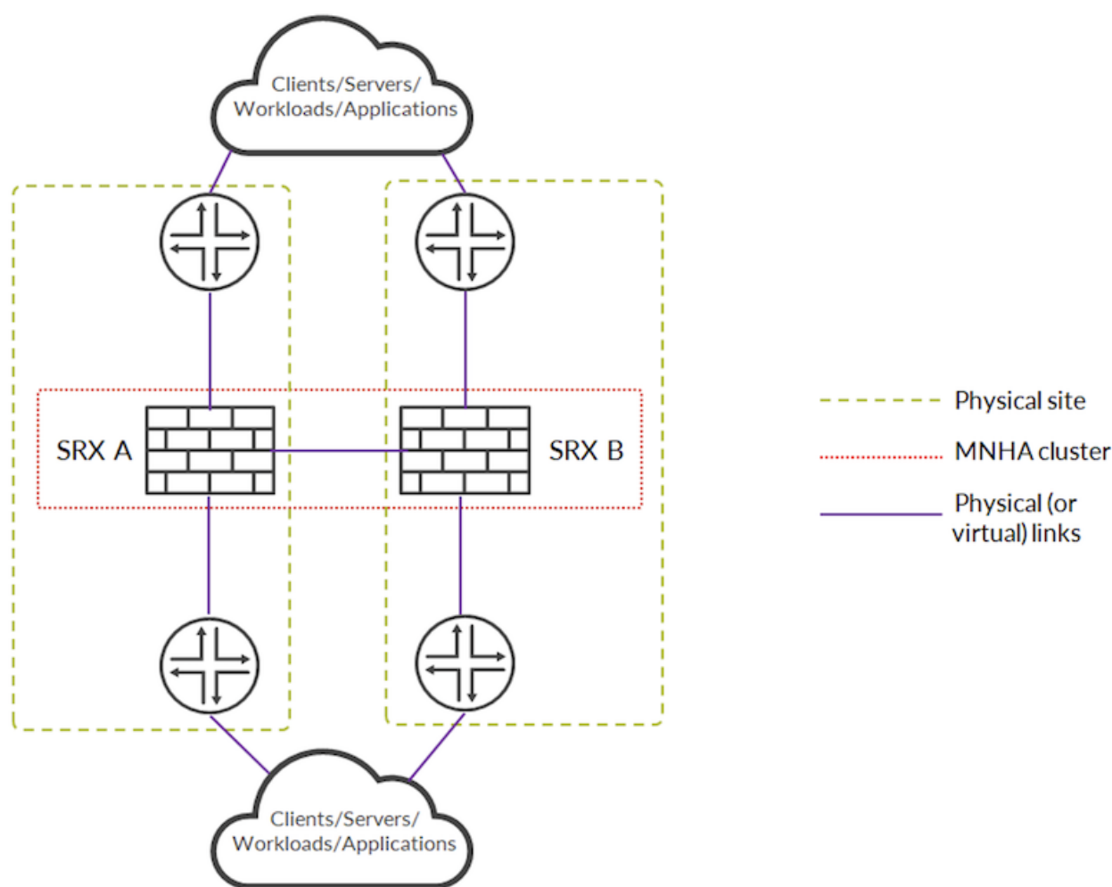
Figure 2: Topology example with MNHA
