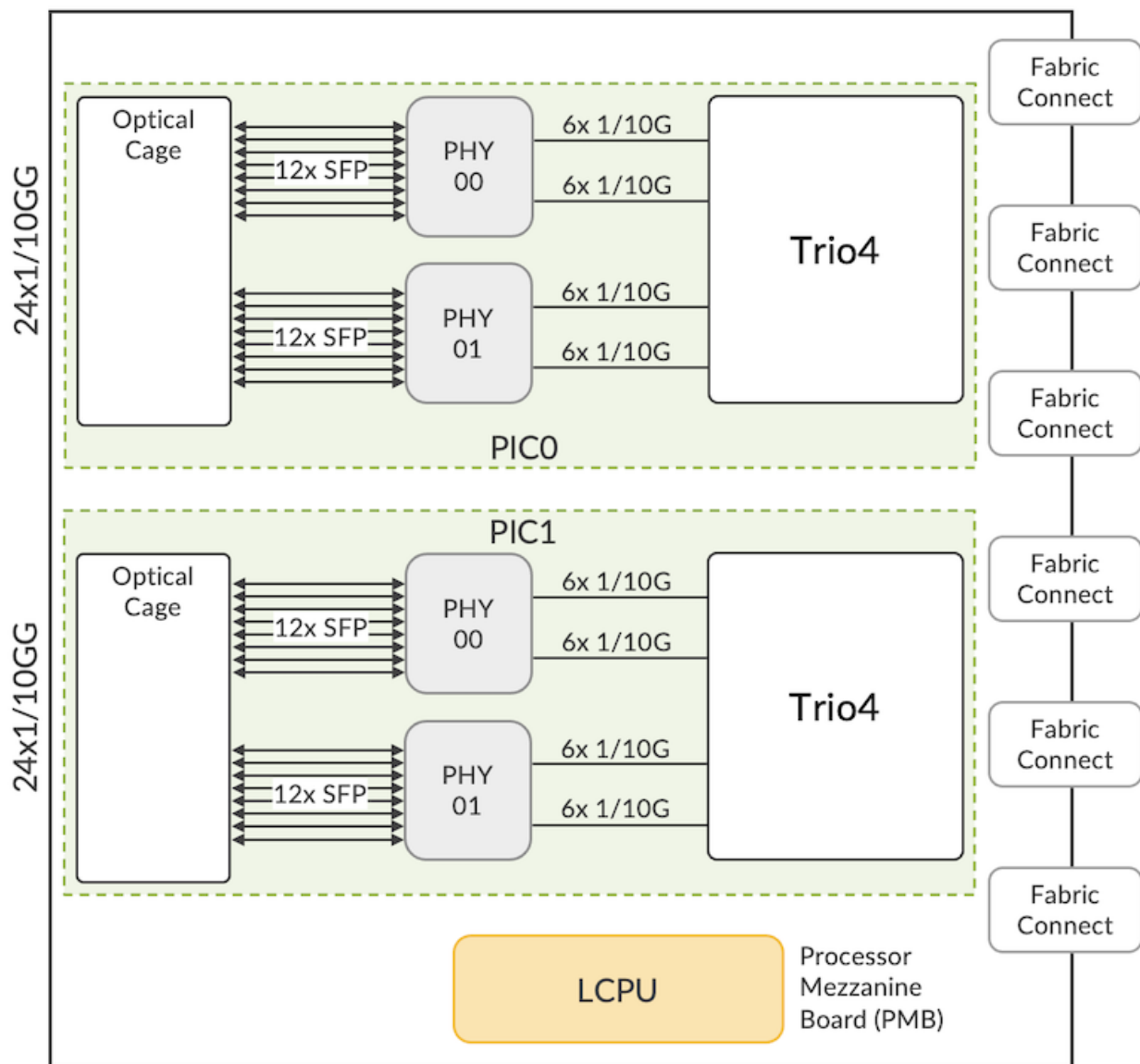
Figure 5: LC 480 Architecture
