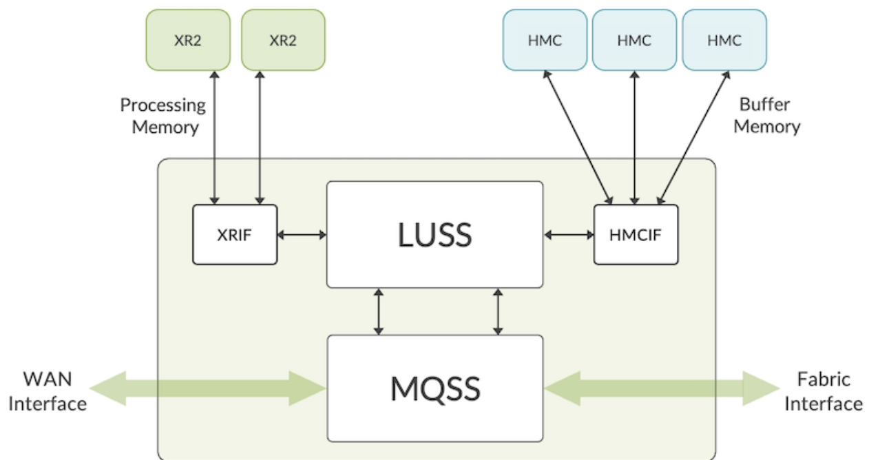
Figure 3: Trio 4 Architecture
