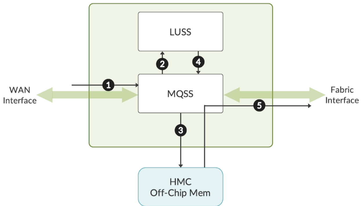
Figure 4: Packet Flow in Trio 4
