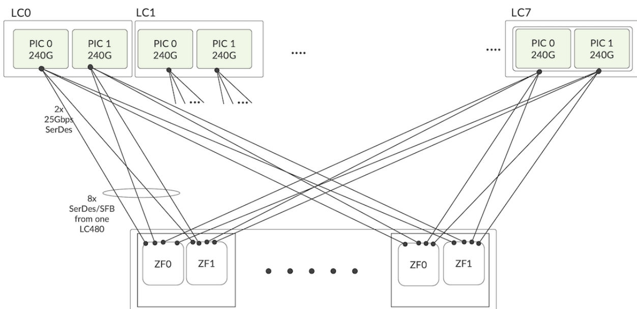
Figure 6: LC480 and SFB2 Interconnect
