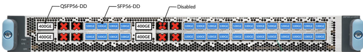
Figure 6: Configuration with 400GbE optics inserted in QSFP slots
