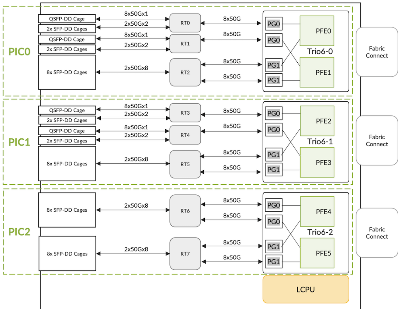
Figure 4: LC4800 Block Diagram with PHYs and Port Groups
