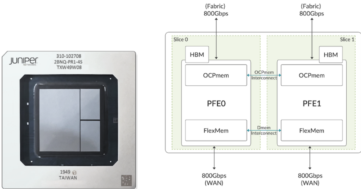
Figure 2: Trio 6 Picture and High-Level Architecture
