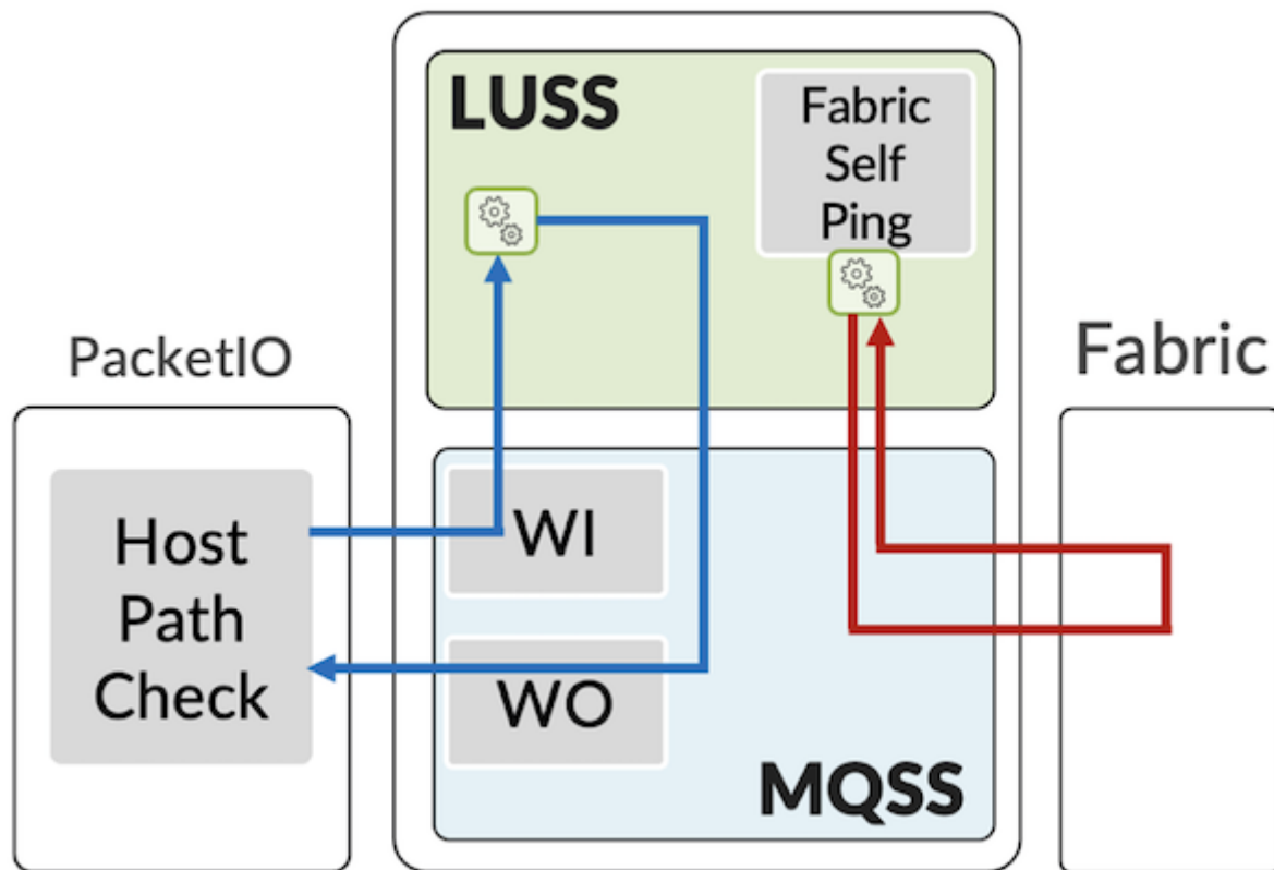
Figure 10: MPC Data Path and Fabric Path Health Check
