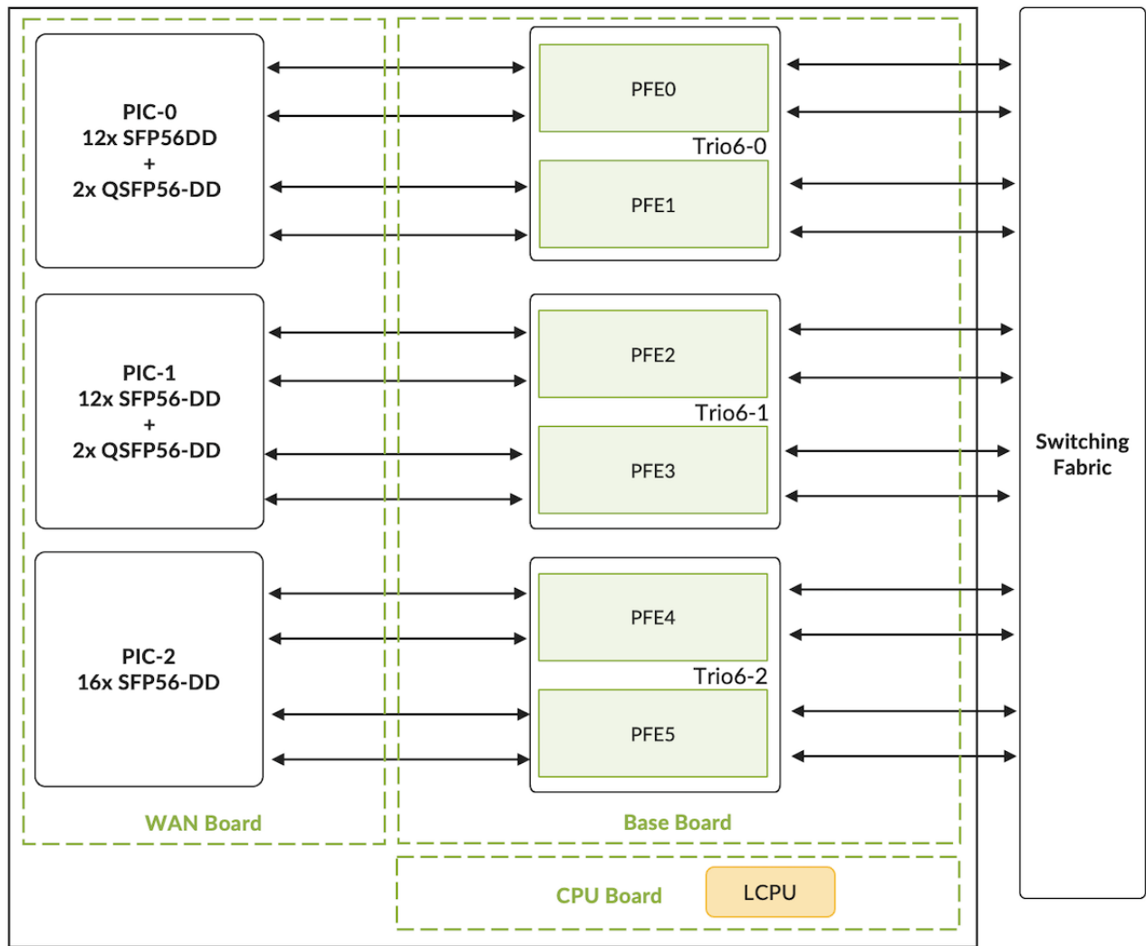
Figure 3: LC4800 High-Level Architecture
