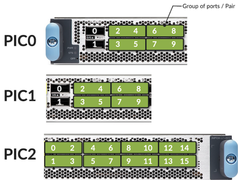
Figure 10: Pair of ports per PIC
