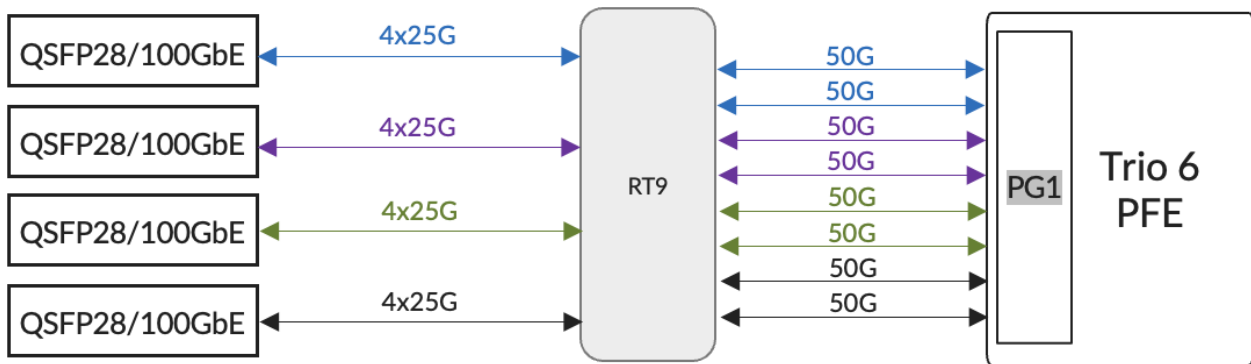
Figure 8: RT/PHY Example1 with 100GbE Optics
