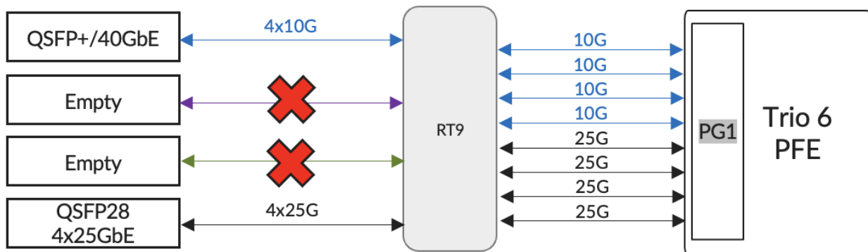
Figure 9: RT/PHY Example2 with 40GbE, 4x10GbE and/or 4x25GbE Optics
