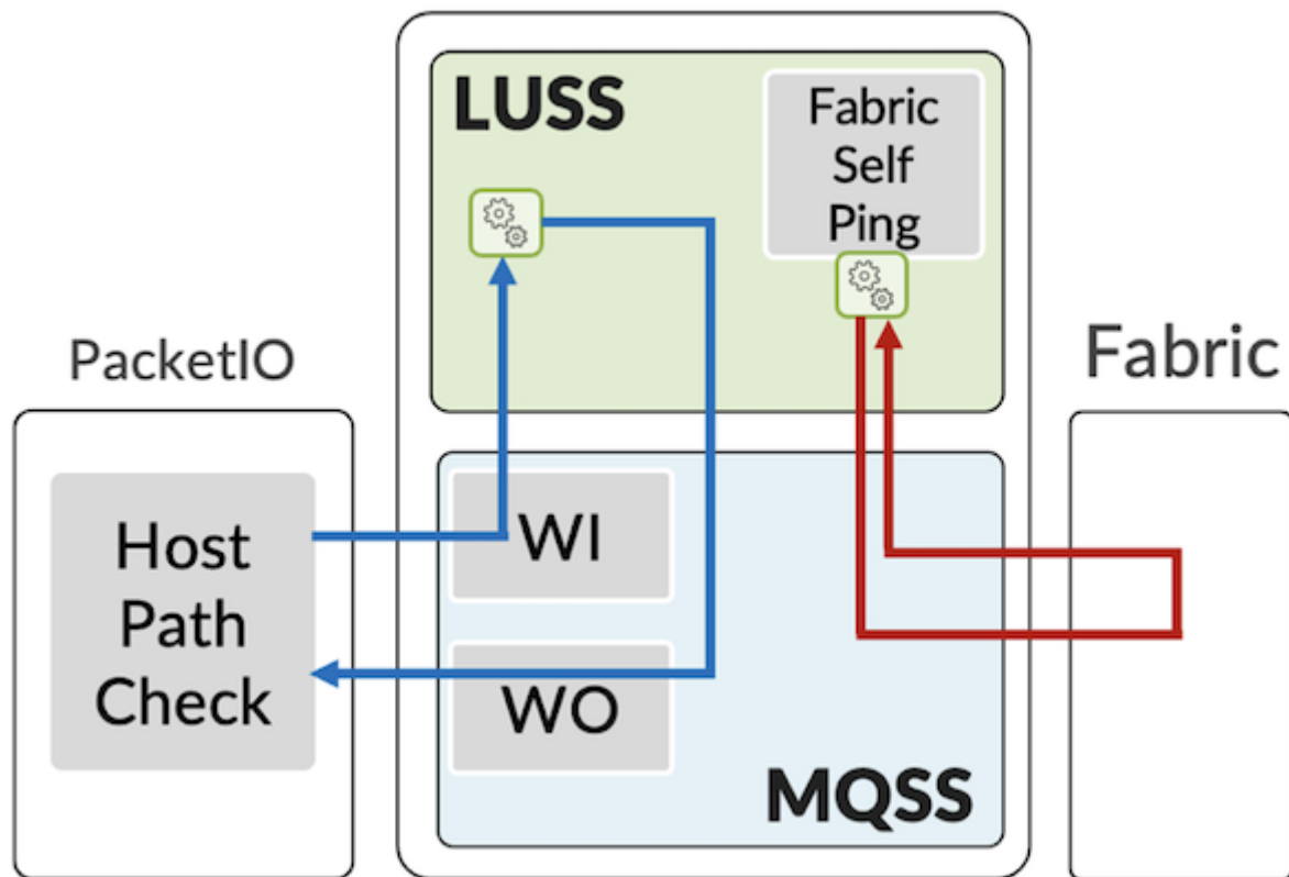
Figure 14: MPC Data Path and Fabric Path Health Check
