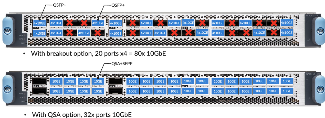
Figure 12: 10GbE options on LC4802
