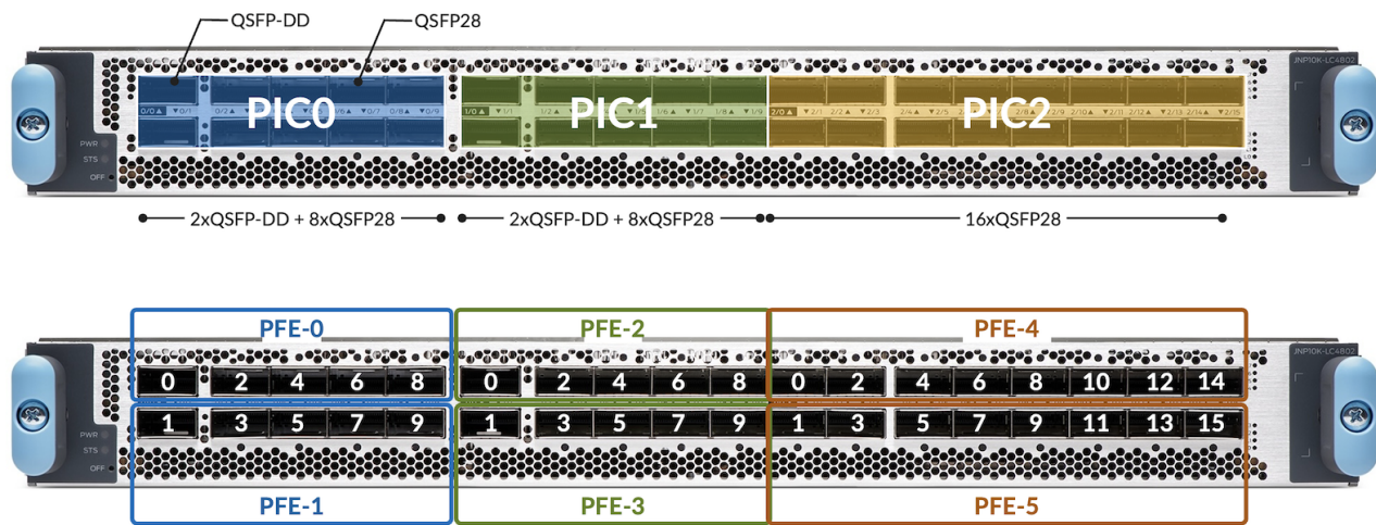
Figure 5: LC4800 PICs, PFEs, and Port Numbers
