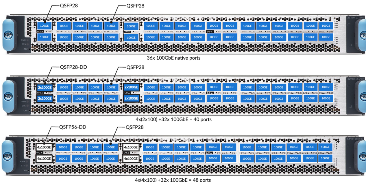
Figure 7: 100GbE Options in LC4800
