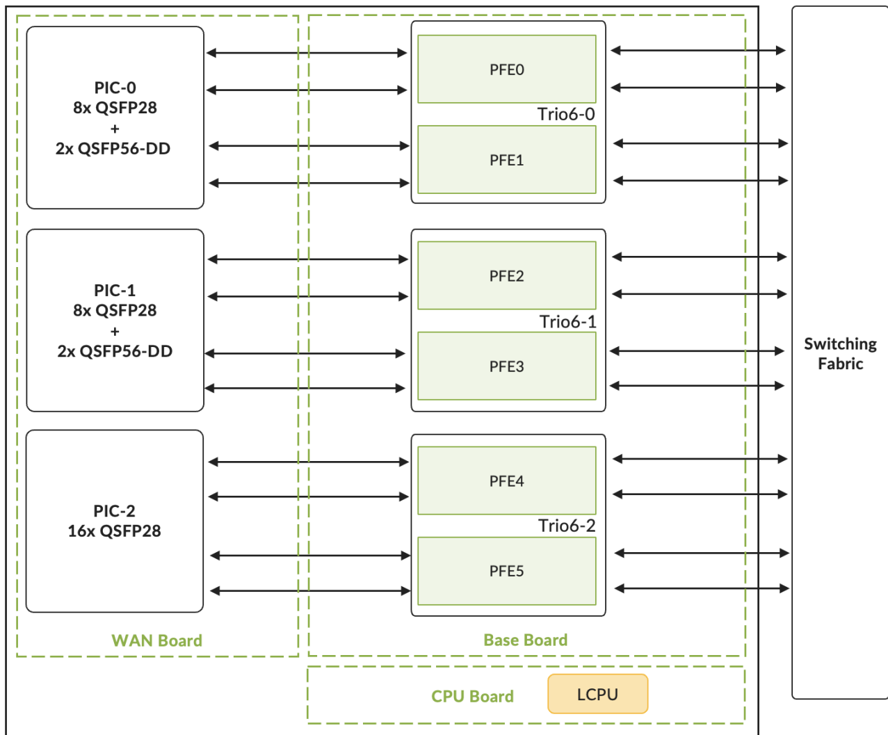
Figure 3: LC4802 High-Level Architecture
