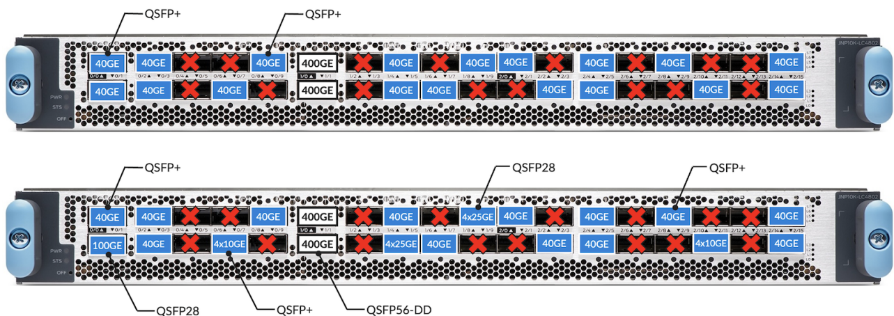
Figure 11: Examples of port distribution options
