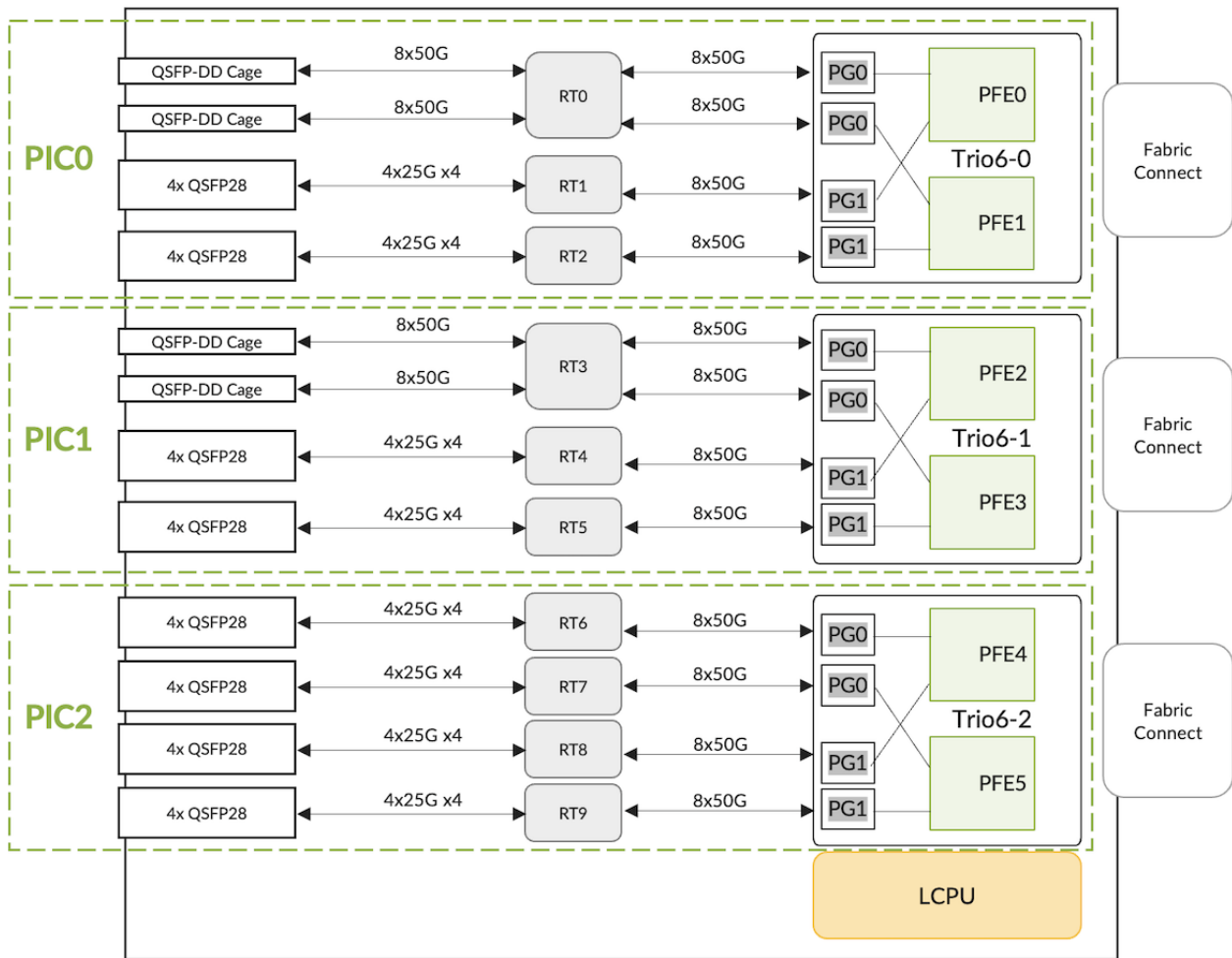
Figure 4: LC4802 Block Diagram with PHYs and Port Groups
