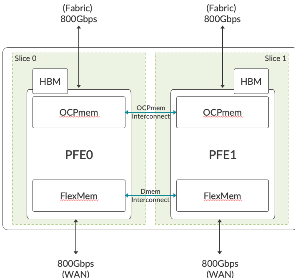
Figure 1: Trio 6 Architecture
