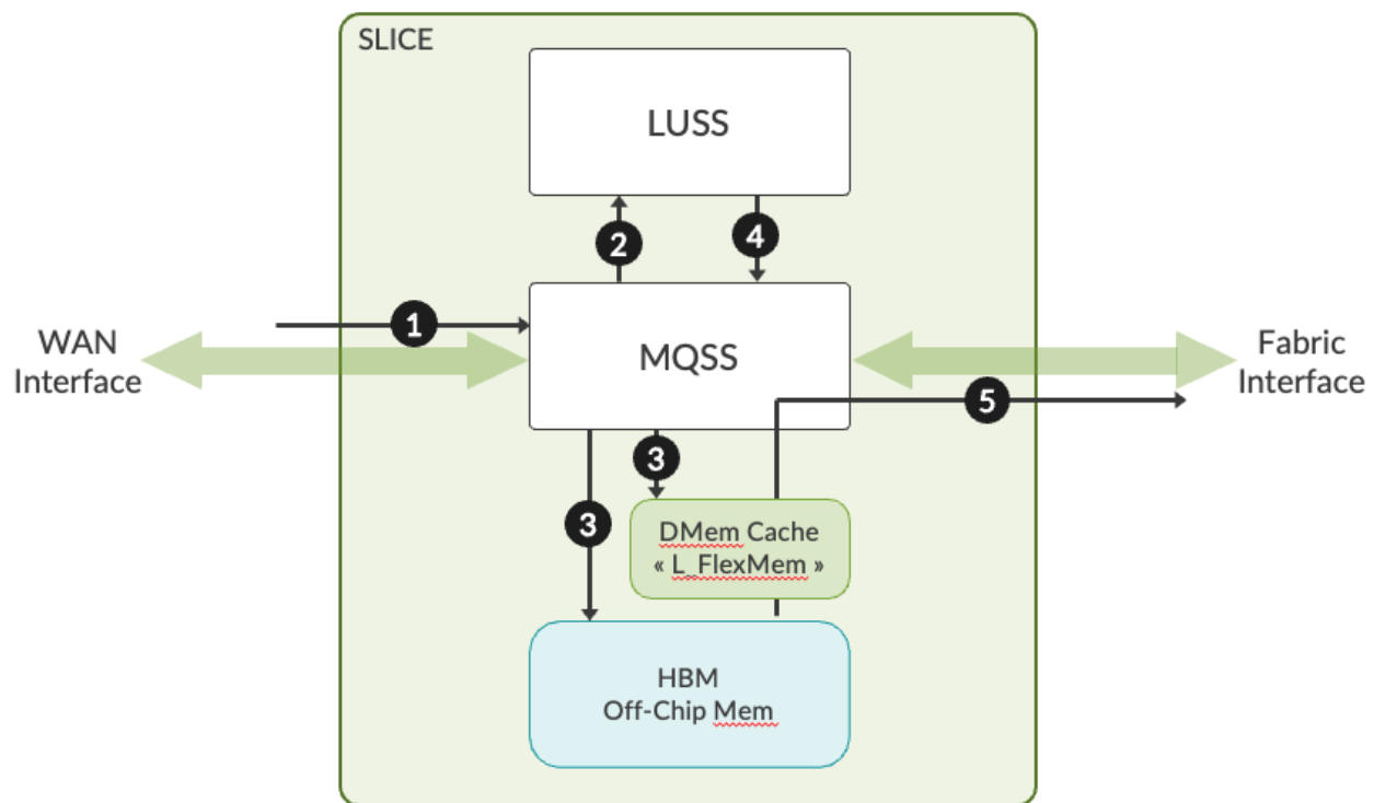
Figure 2: Packet Flow
