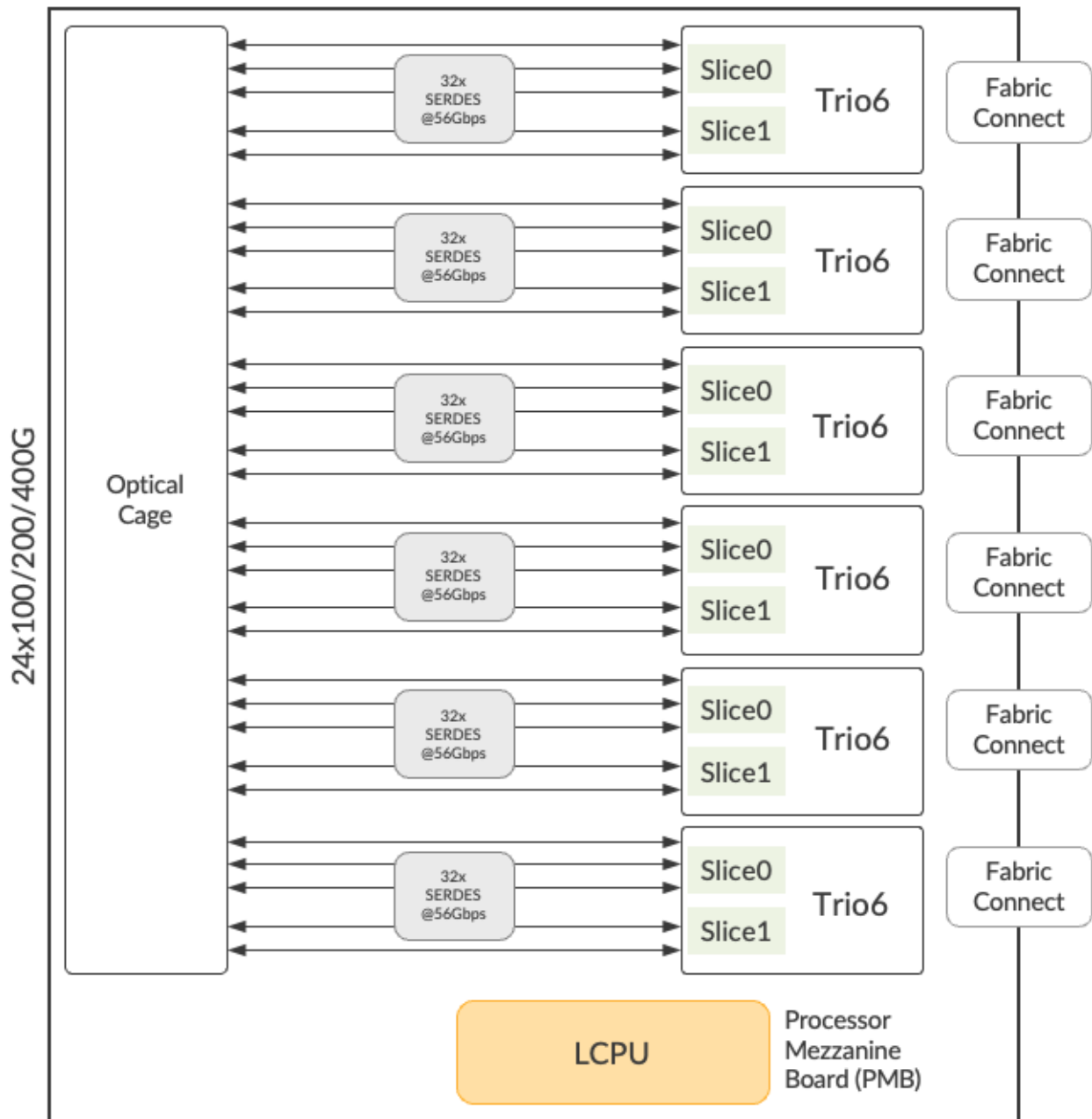
Figure 3: LC9600 Architecture
