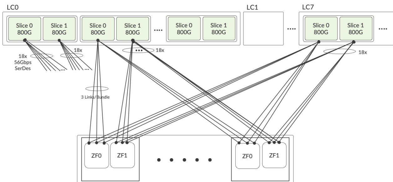
Figure 4: LC9600 and SFB2 Interconnect
