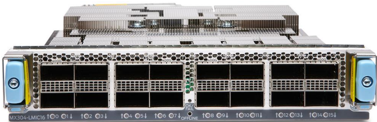
Figure 10: MX304 LMIC
