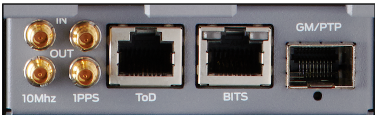
Figure 14: MX304 TIB
