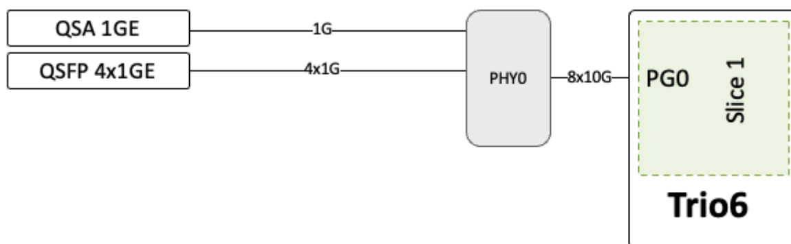
Figure 25: Sub-ports configuration
