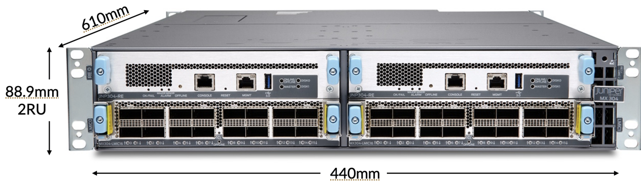
Figure 2: MX304 Dimensions
