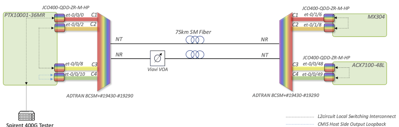
Figure 1: Physical Topology - Traffic Flow
