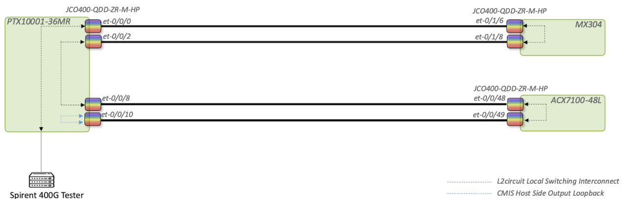
Figure 2: Logical Topology - Traffic Flow
