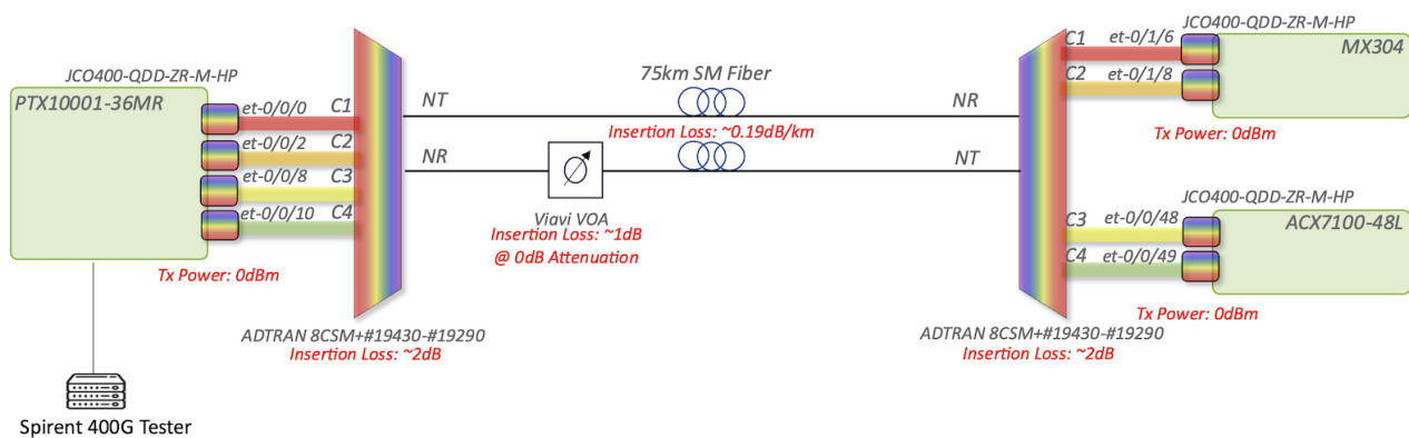
Figure 3: Power Propagation Calculation
