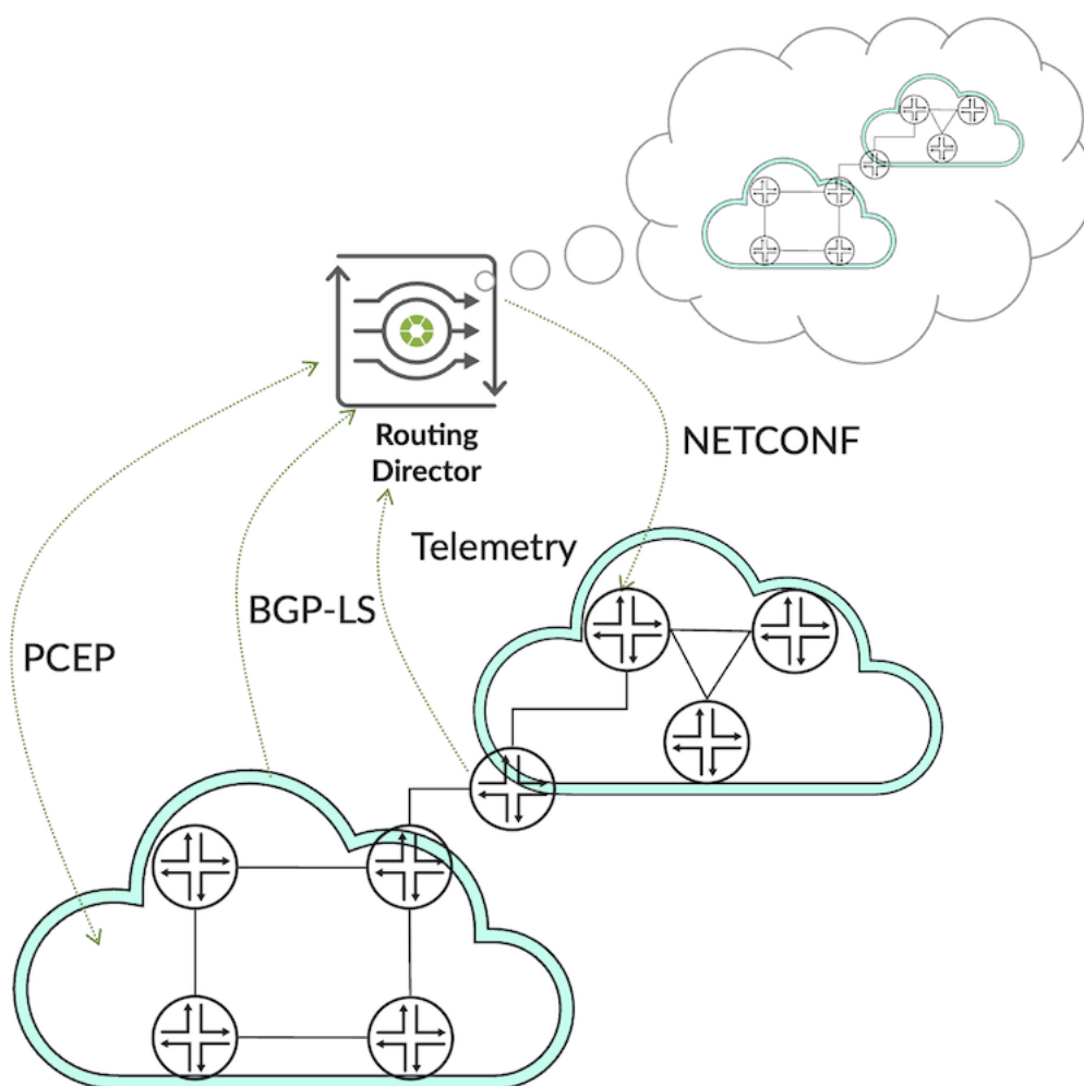
Figure 1: Logical Connection Infrastructure
