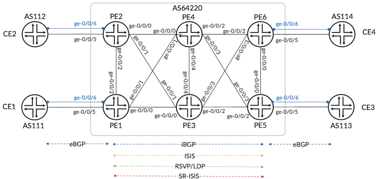
Figure 2: Network Topology
