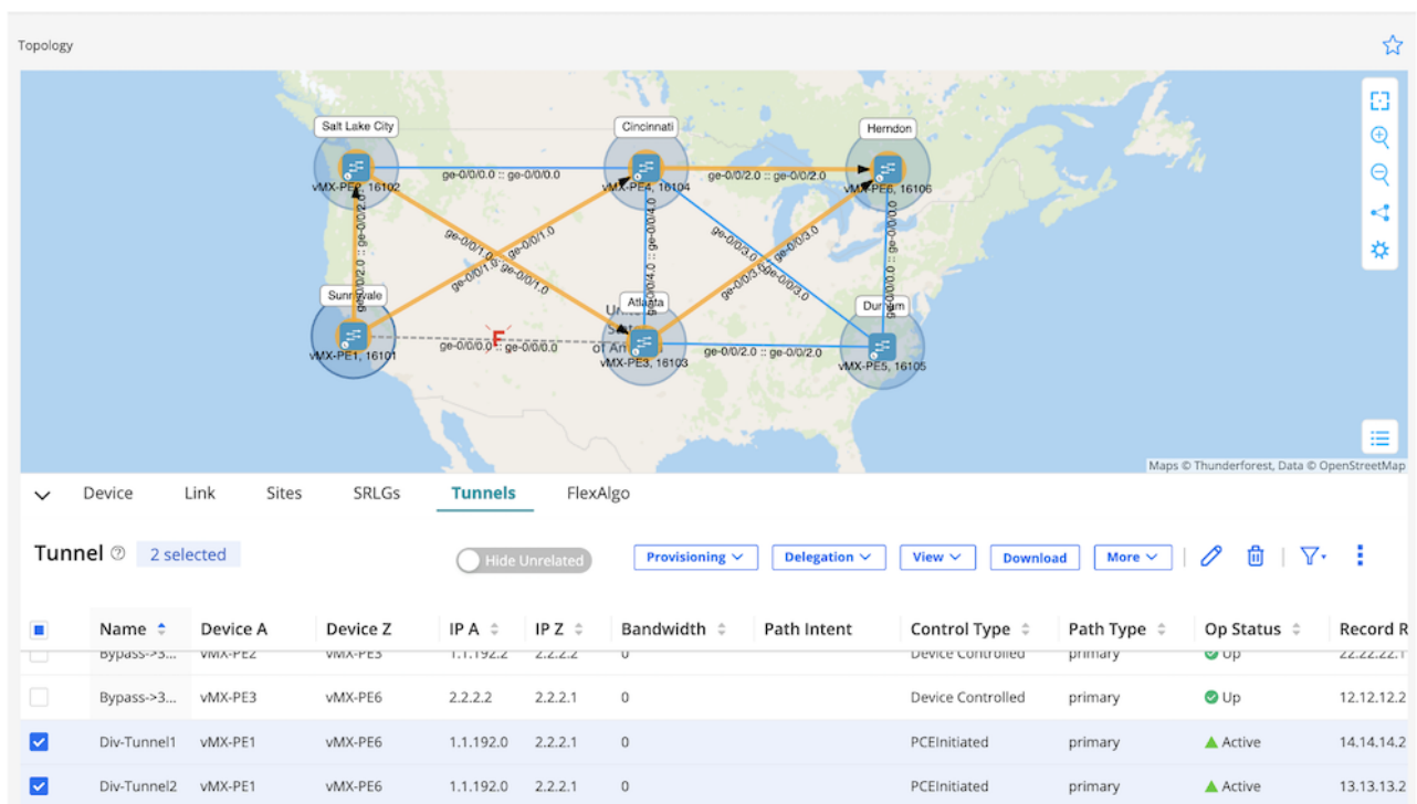
Figure 11: - Tunnel Diversity Path After Simulate Fibre Cut
