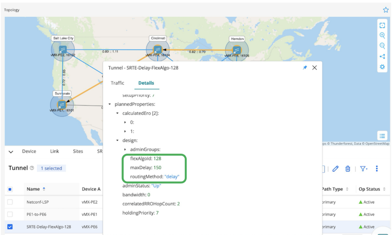
Figure 25: Detail Tunnel Information Align with Defined Variables
