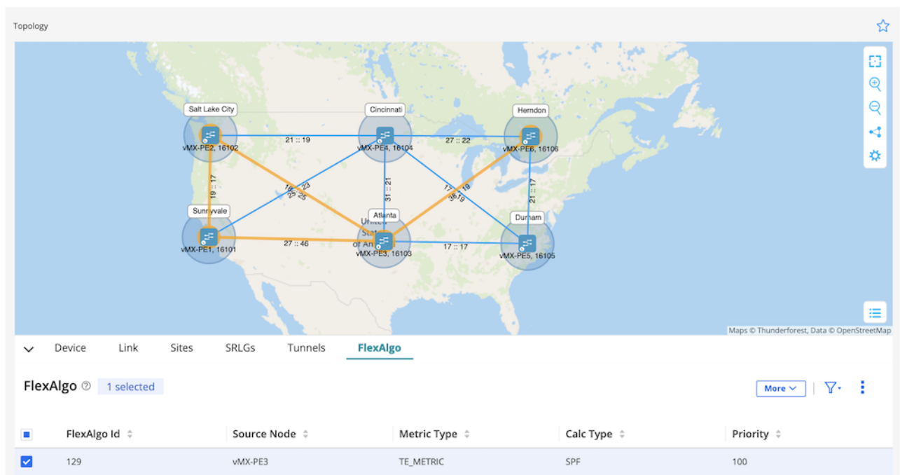
Figure 21: Flex-Algo 129 Topology
