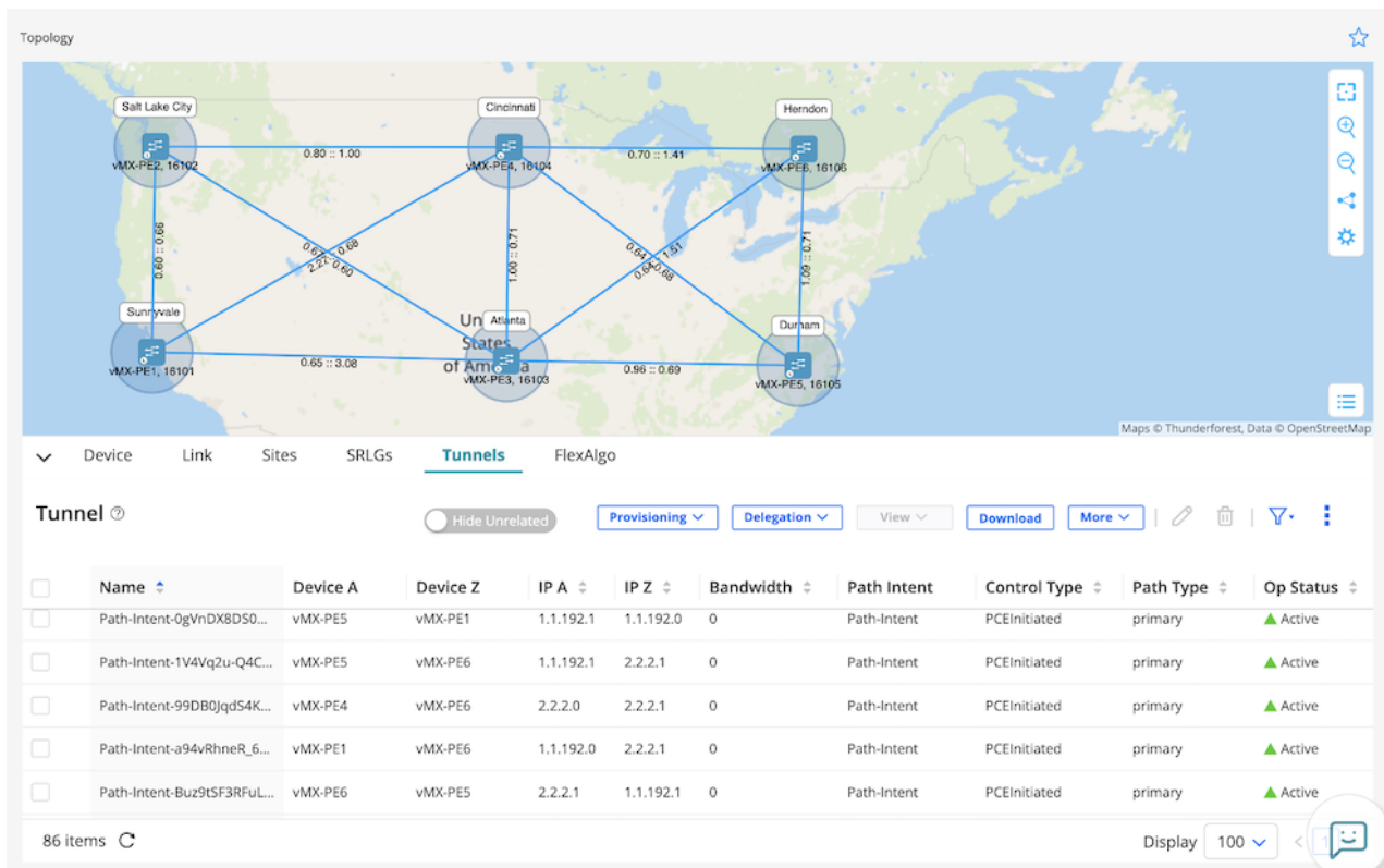
Figure 35: all SR-TE Tunnels Up
